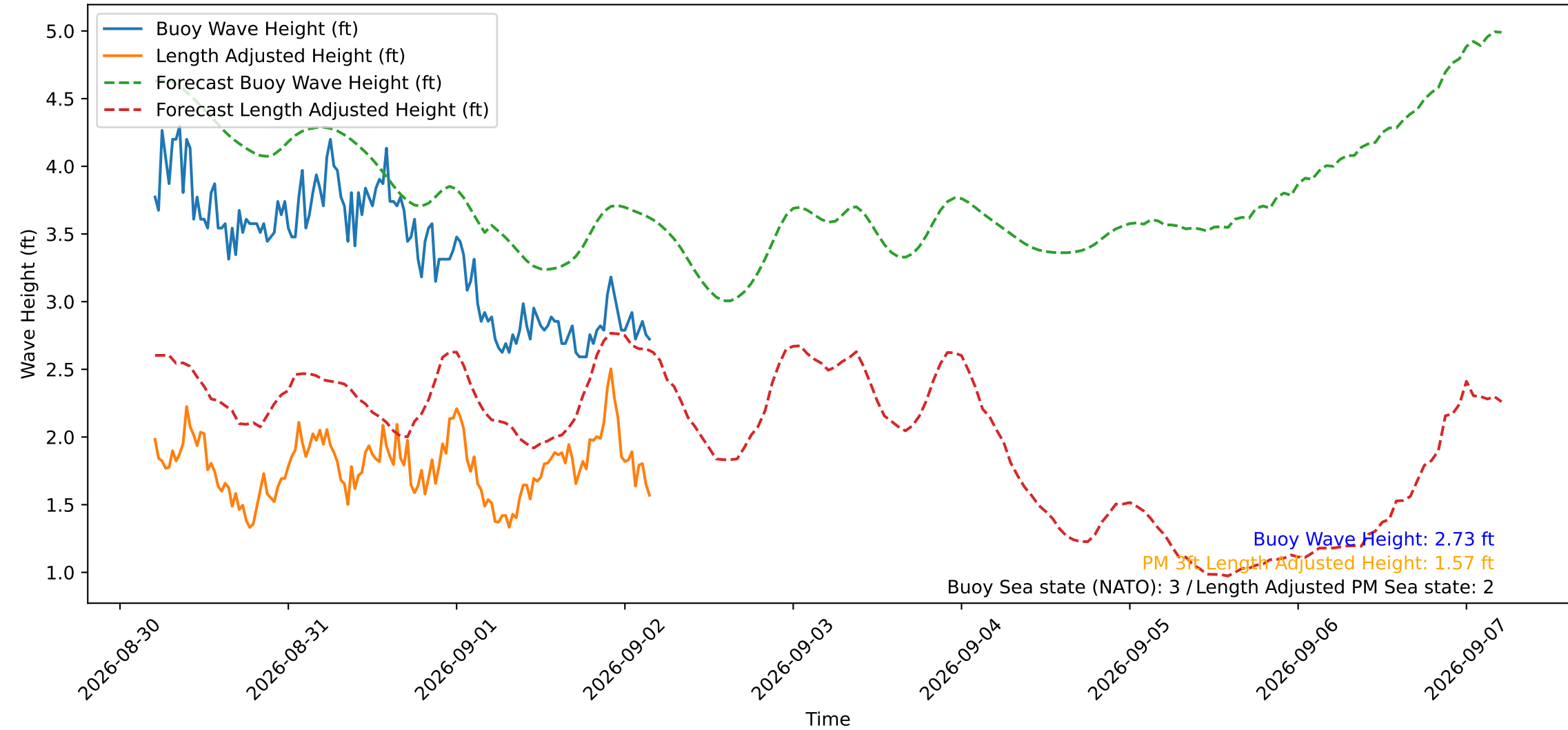
Wave Heights over Time for Red Beach at 2026-09-02 04:30:50
