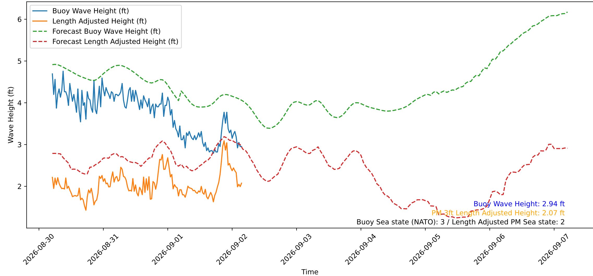
Wave Heights over Time for Green Beach at 2026-09-02 04:31:13
