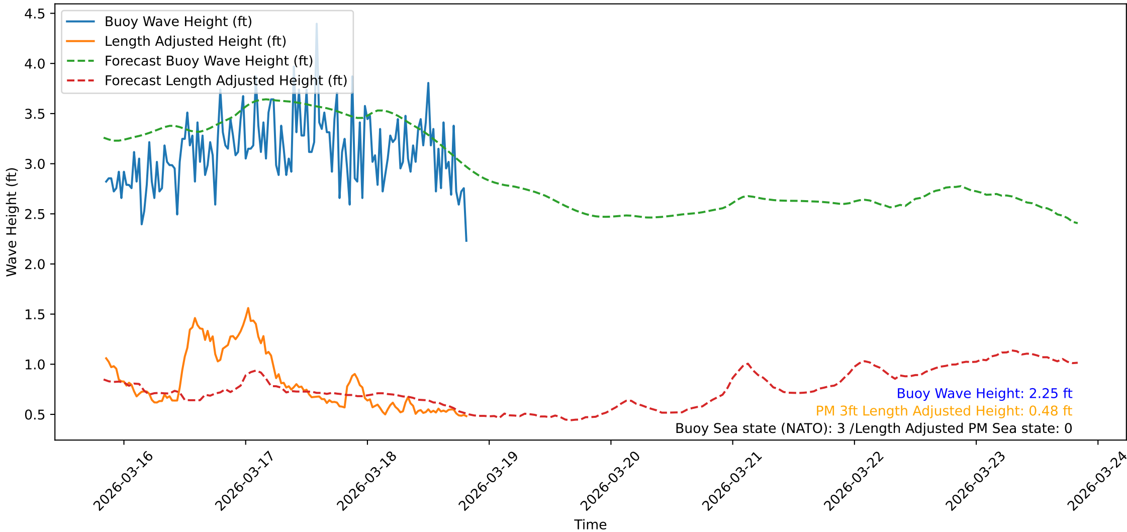
Wave Heights over Time for Oceanside Harbor at 2026-03-18 20:20:31
