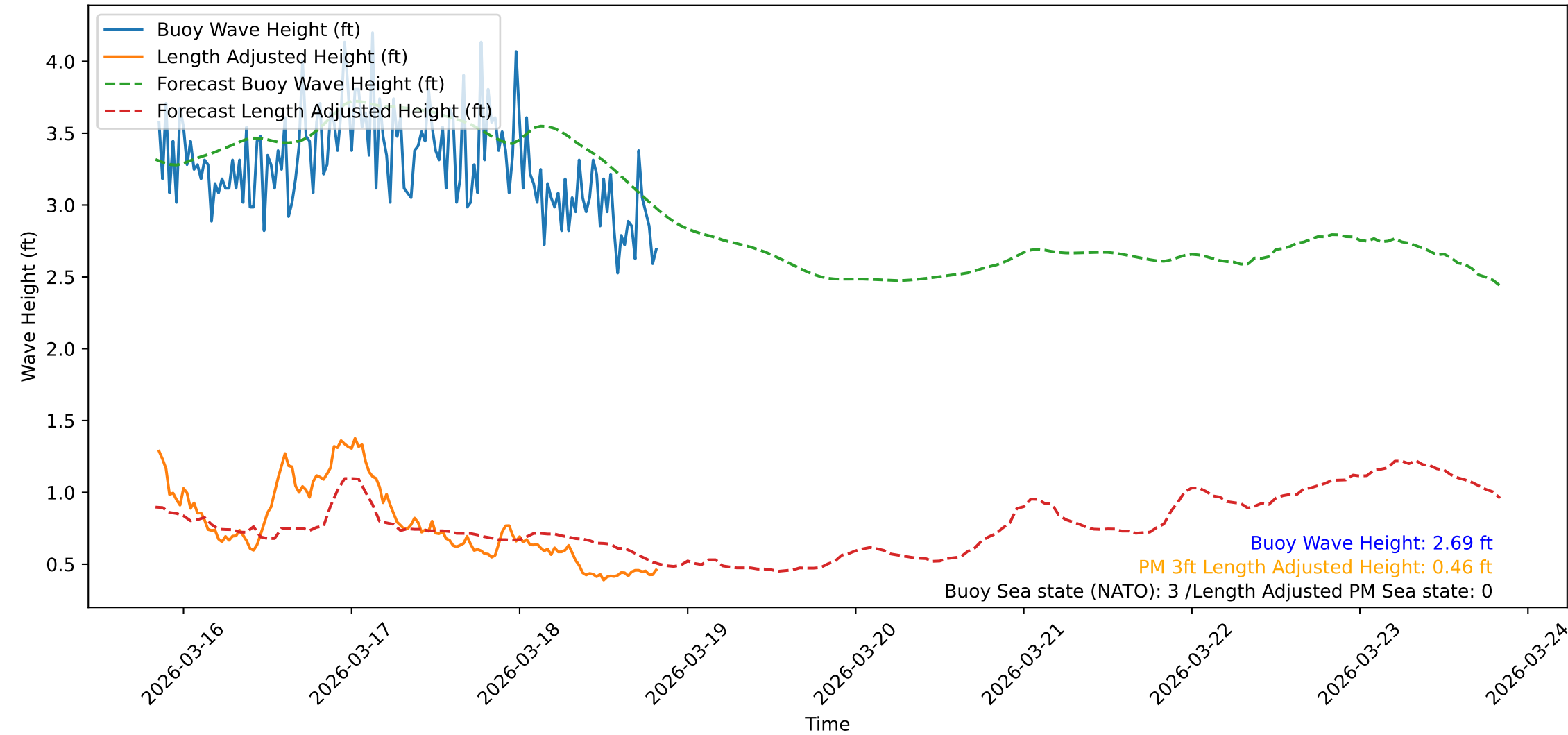
Wave Heights over Time for Green Beach at 2026-03-18 20:21:10
