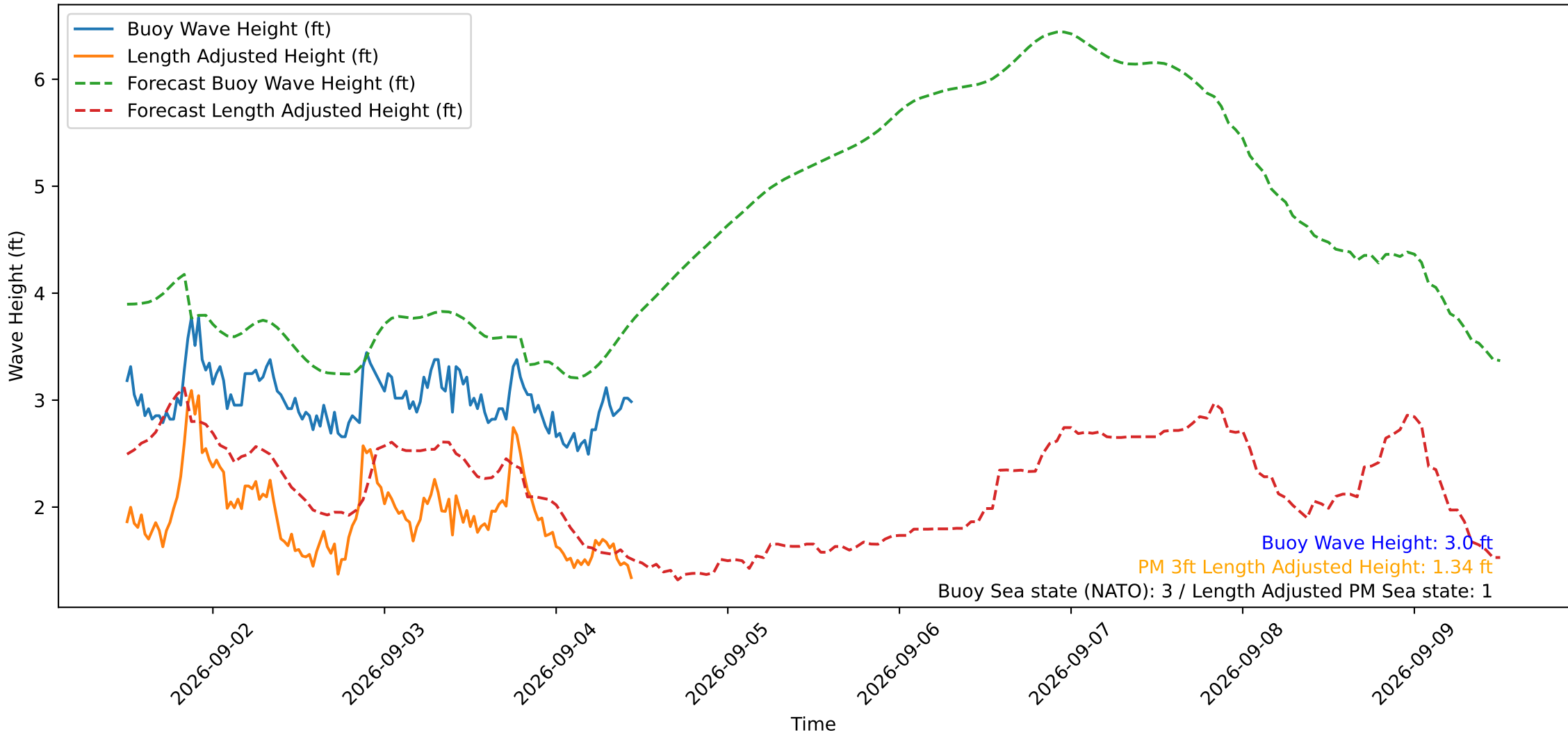
Wave Heights over Time for Green Beach at 2026-09-04 11:31:11
