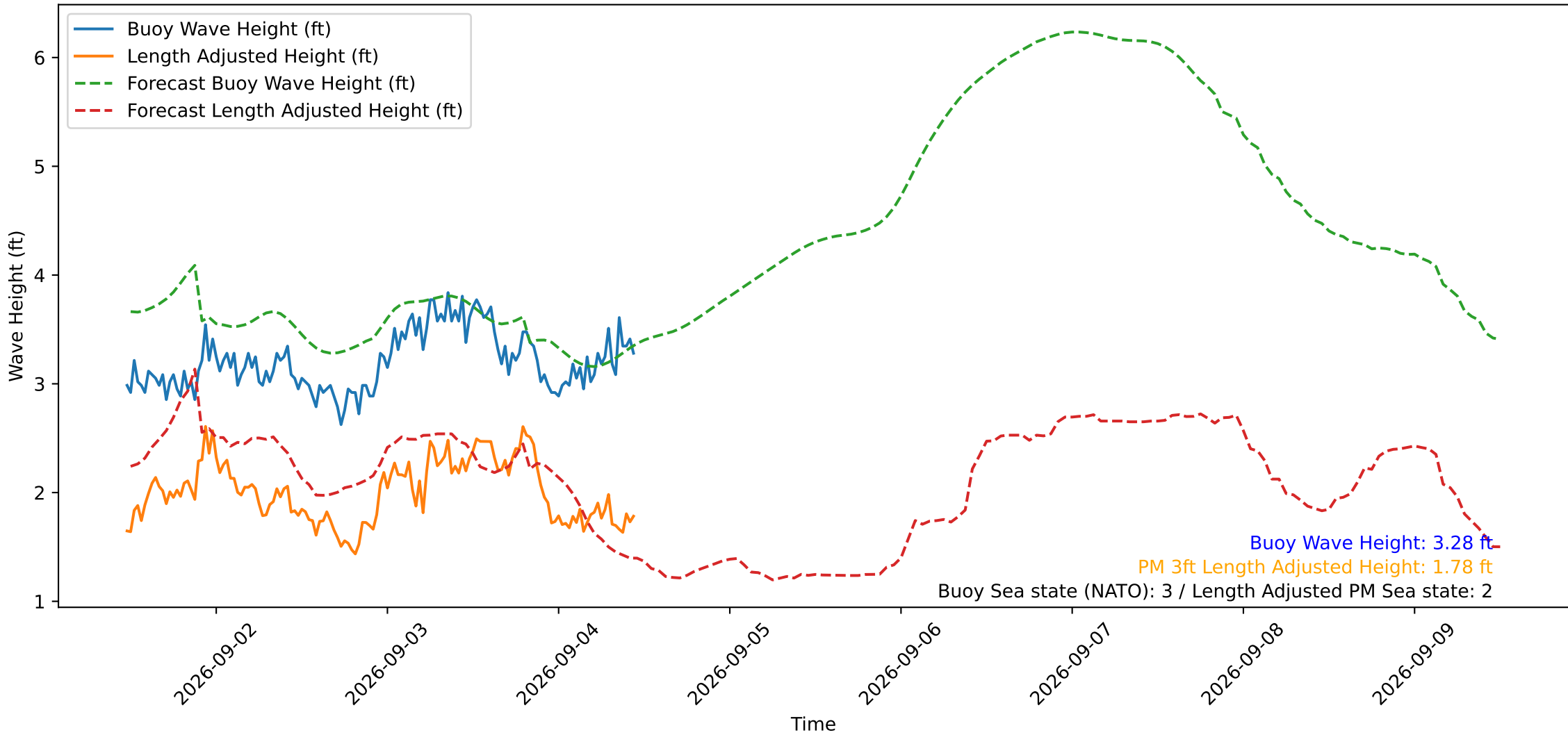
Wave Heights over Time for Oceanside Harbor at 2026-09-04 11:30:29
