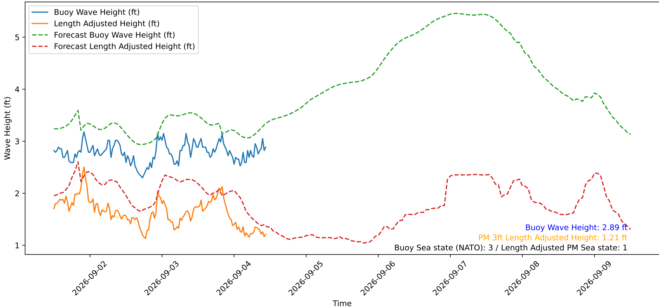
Wave Heights over Time for Red Beach at 2026-09-04 11:30:49
