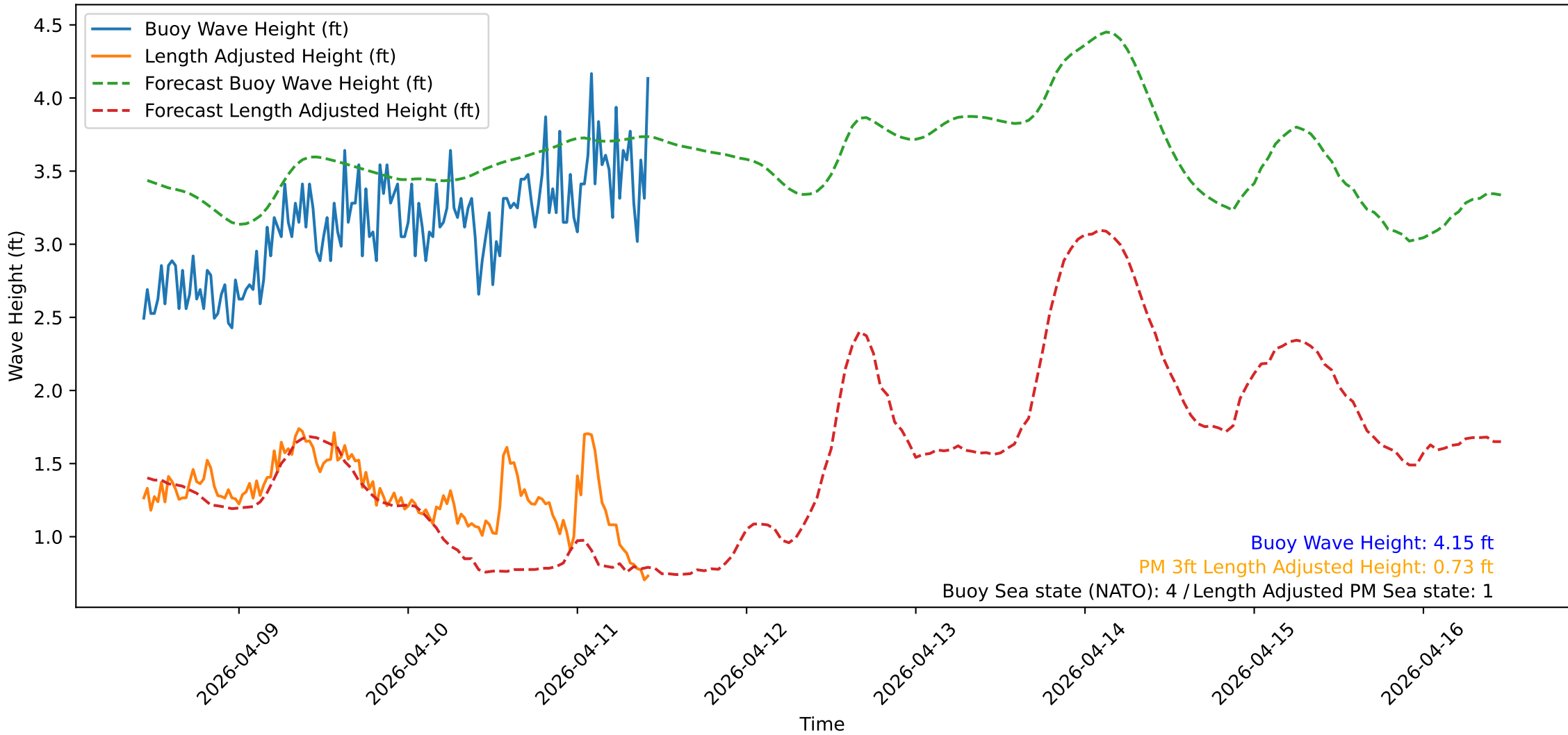
Wave Heights over Time for Oceanside Harbor at 2026-04-11 10:40:31
