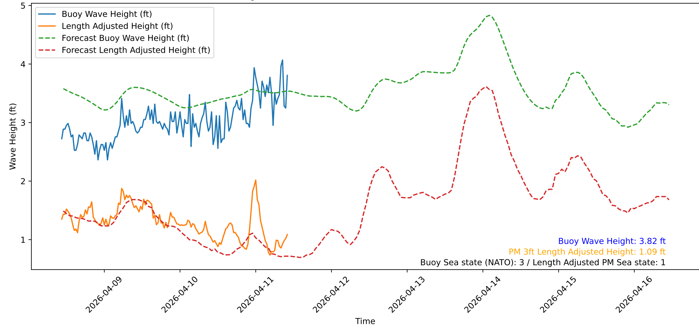
Wave Heights over Time for Green Beach at 2026-04-11 10:41:13
