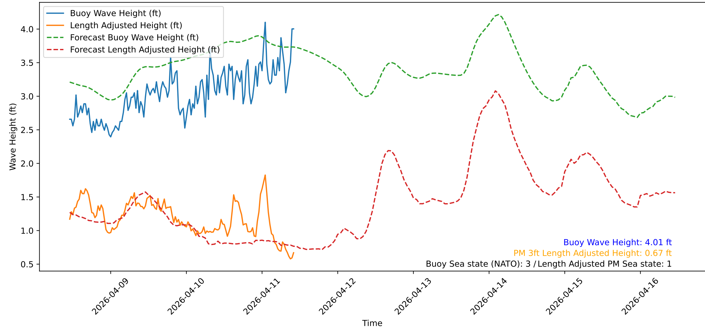
Wave Heights over Time for Red Beach at 2026-04-11 10:40:50
