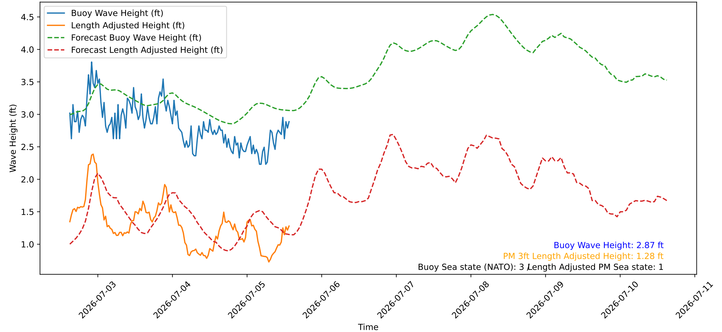
Wave Heights over Time for Red Beach at 2026-07-05 14:30:47
