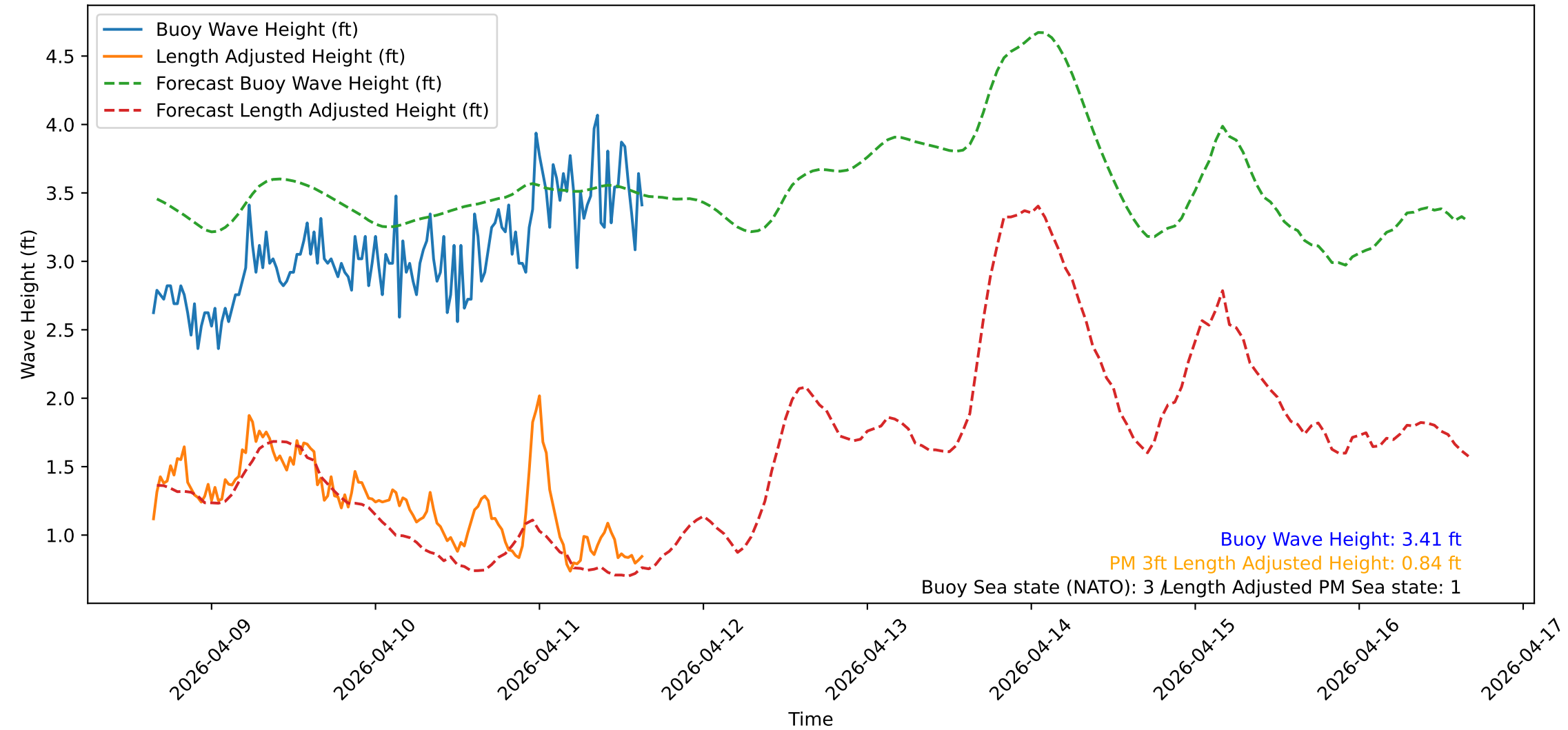
Wave Heights over Time for Green Beach at 2026-04-11 15:41:13
