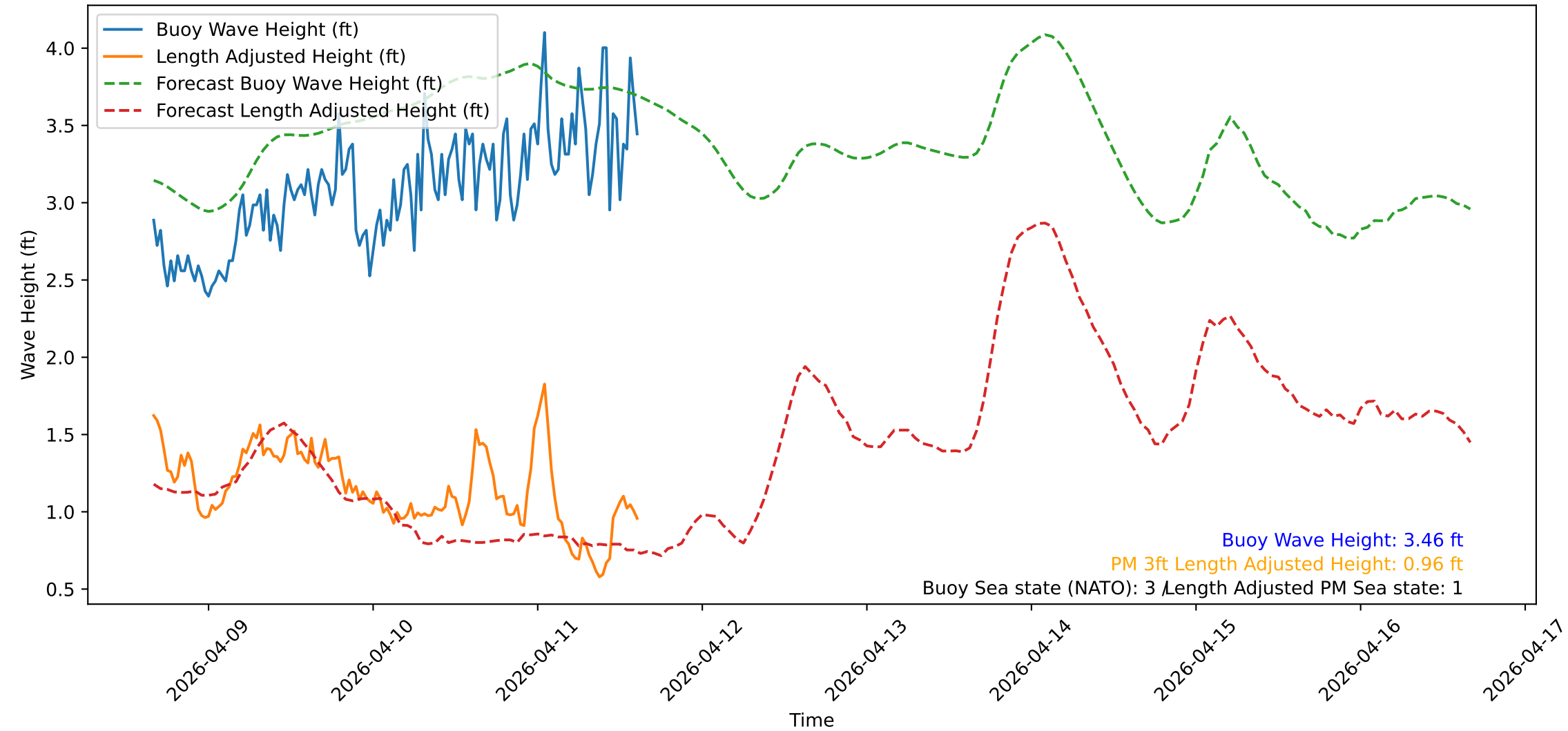
Wave Heights over Time for Red Beach at 2026-04-11 15:40:50
