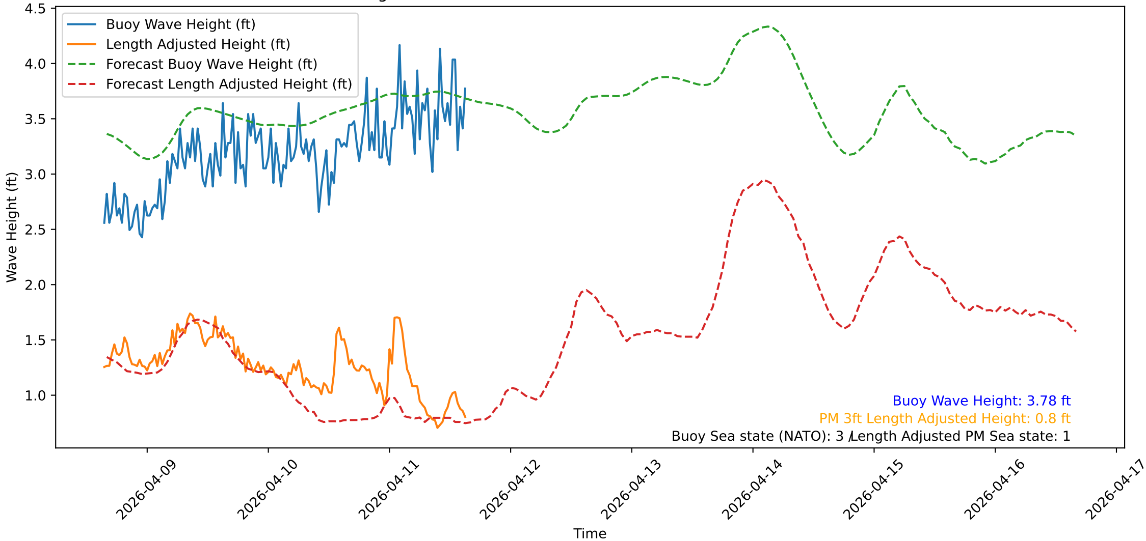
Wave Heights over Time for Oceanside Harbor at 2026-04-11 15:40:31
