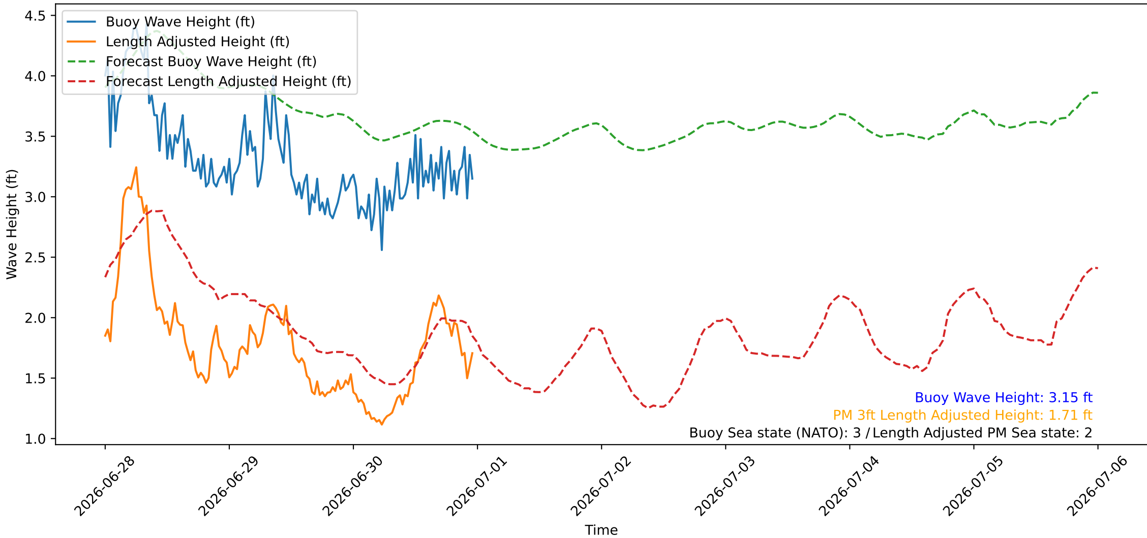
Wave Heights over Time for Oceanside Harbor at 2026-06-30 23:50:26
