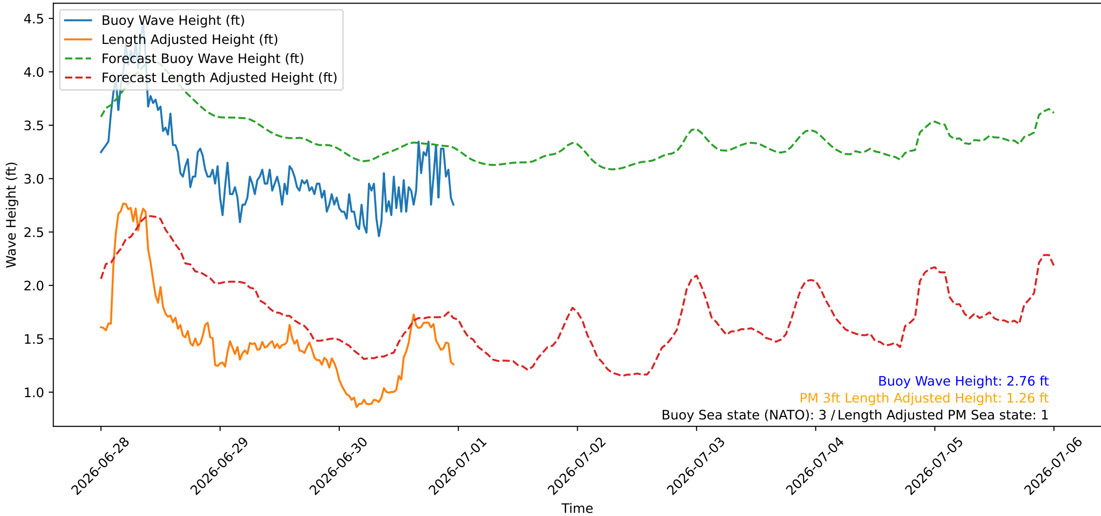
Wave Heights over Time for Red Beach at 2026-06-30 23:50:46
