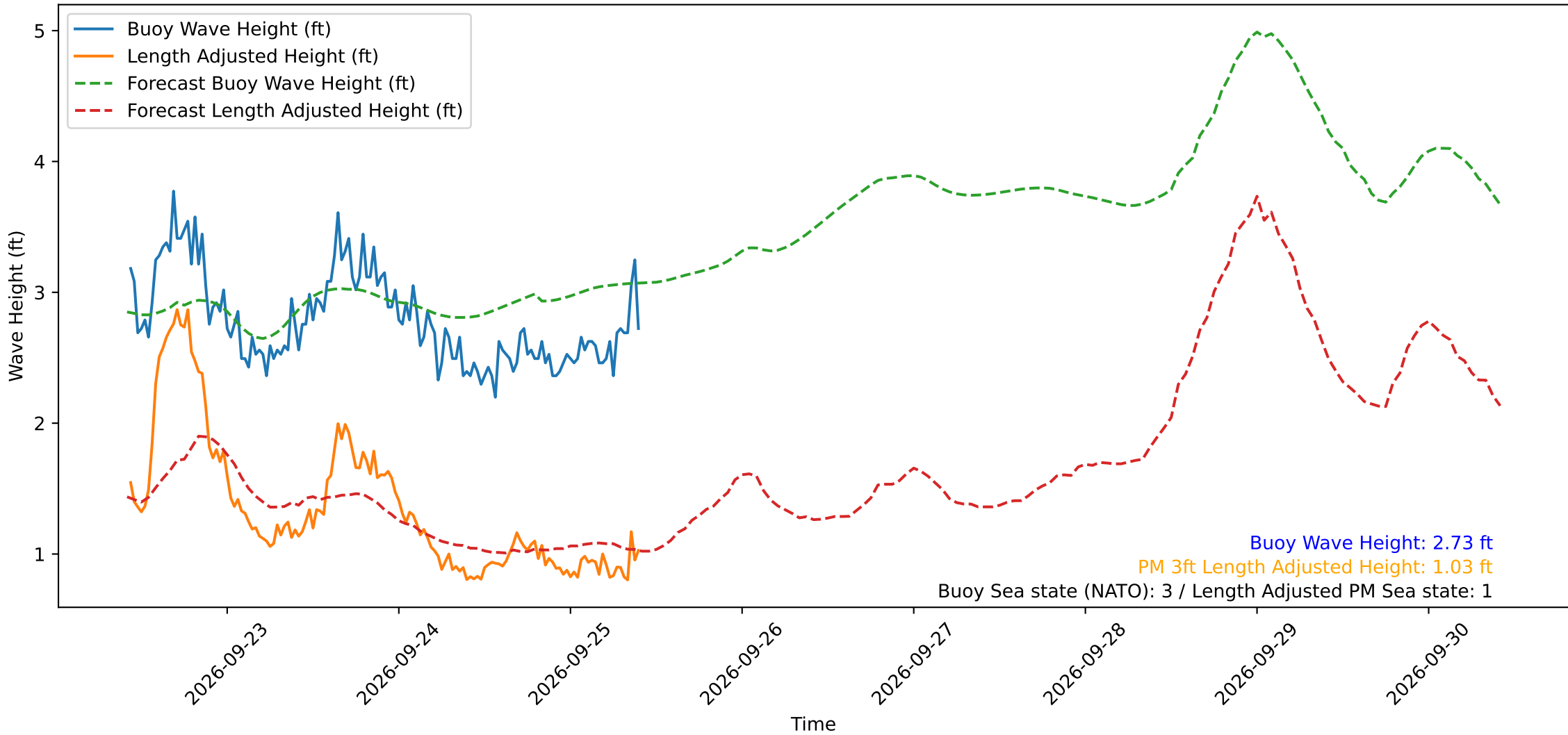
Wave Heights over Time for Oceanside Harbor at 2026-09-25 10:20:29
