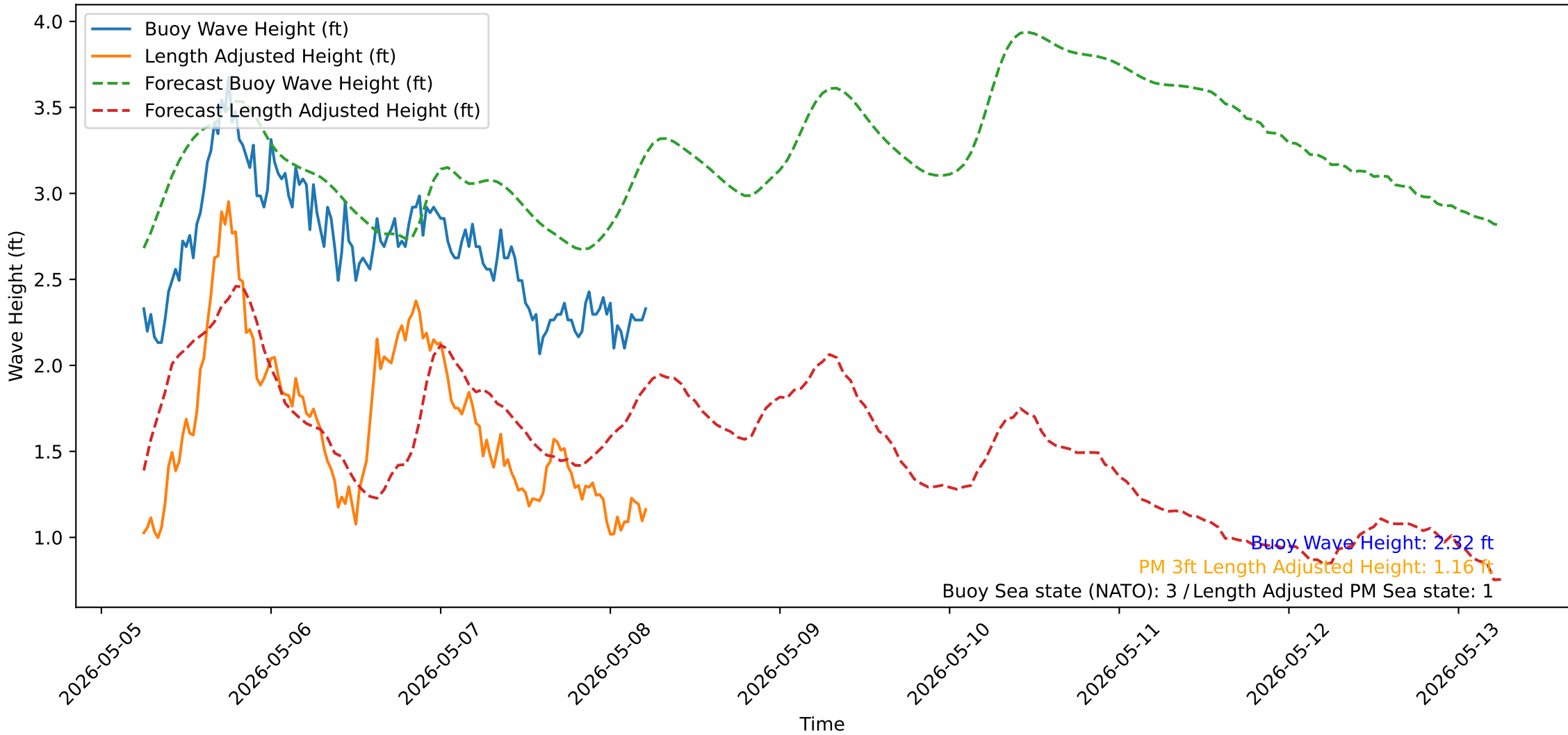
Wave Heights over Time for Green Beach at 2026-05-08 05:51:15
