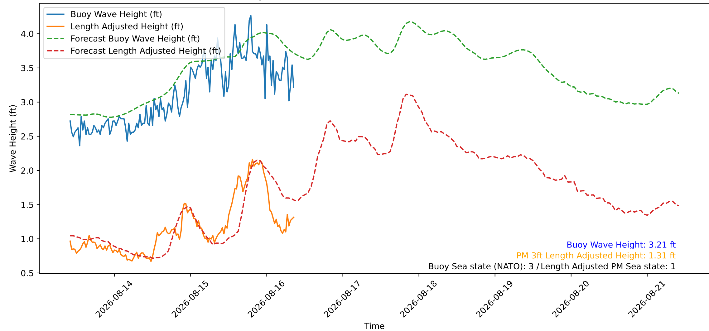
Wave Heights over Time for Green Beach at 2026-08-16 09:31:08
