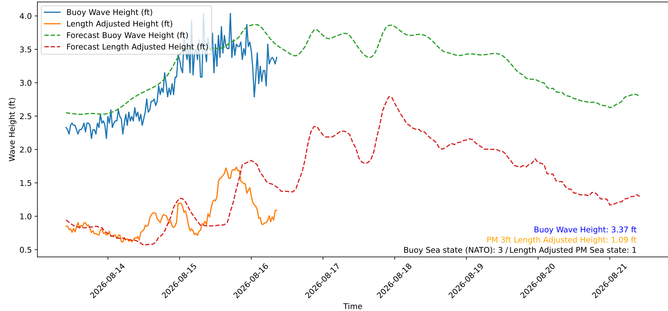
Wave Heights over Time for Red Beach at 2026-08-16 09:30:45
