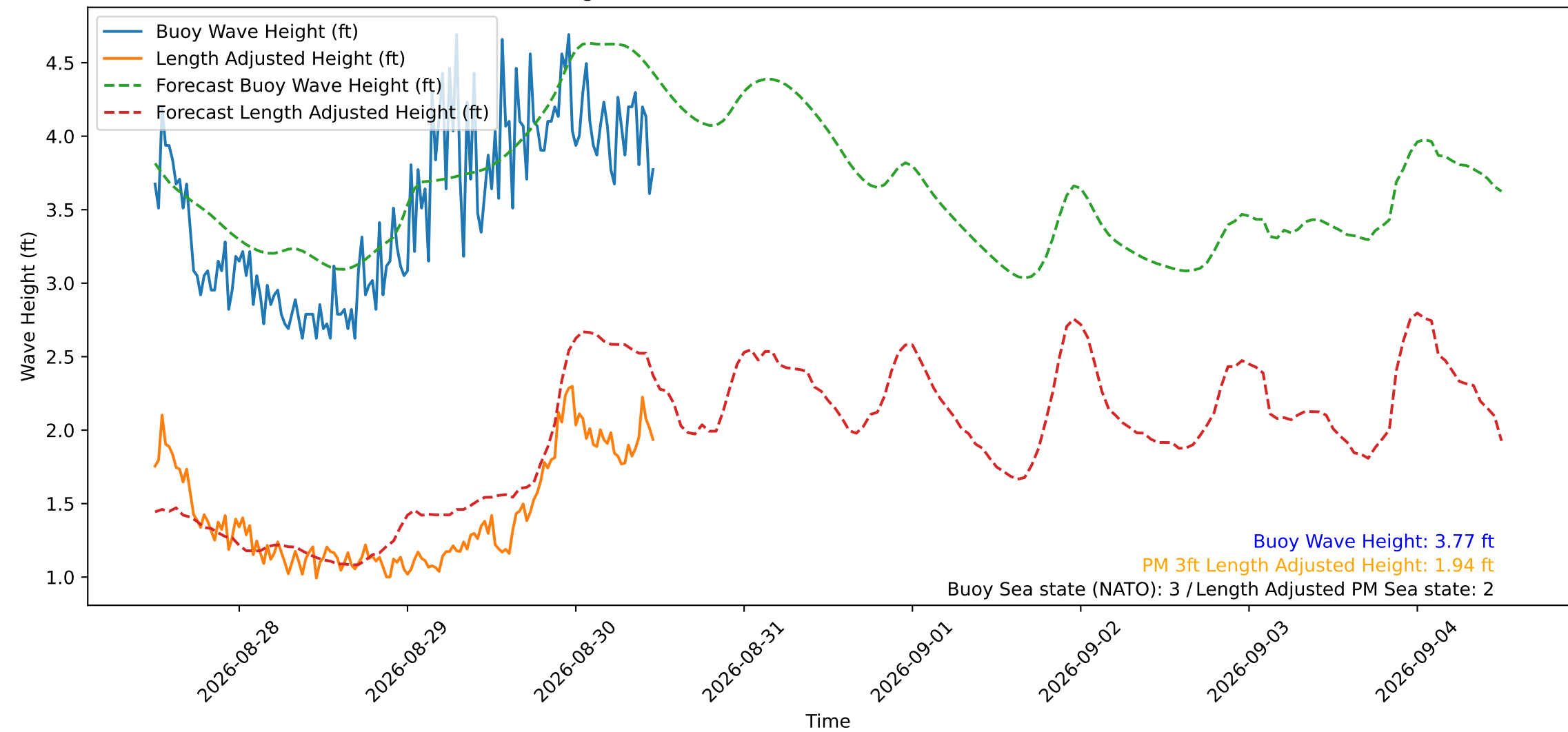
Wave Heights over Time for Red Beach at 2026-08-30 11:50:50
