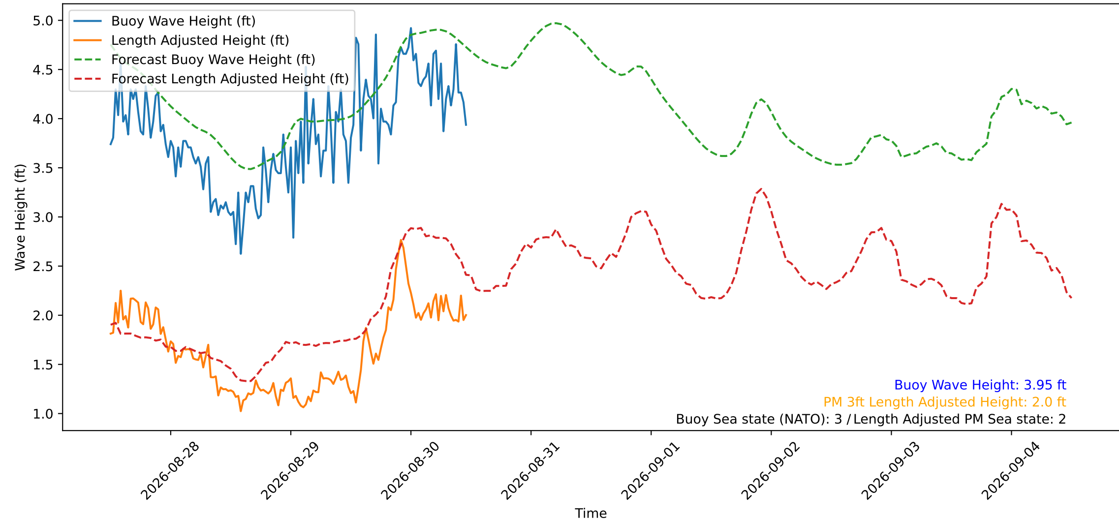
Wave Heights over Time for Green Beach at 2026-08-30 11:51:14
