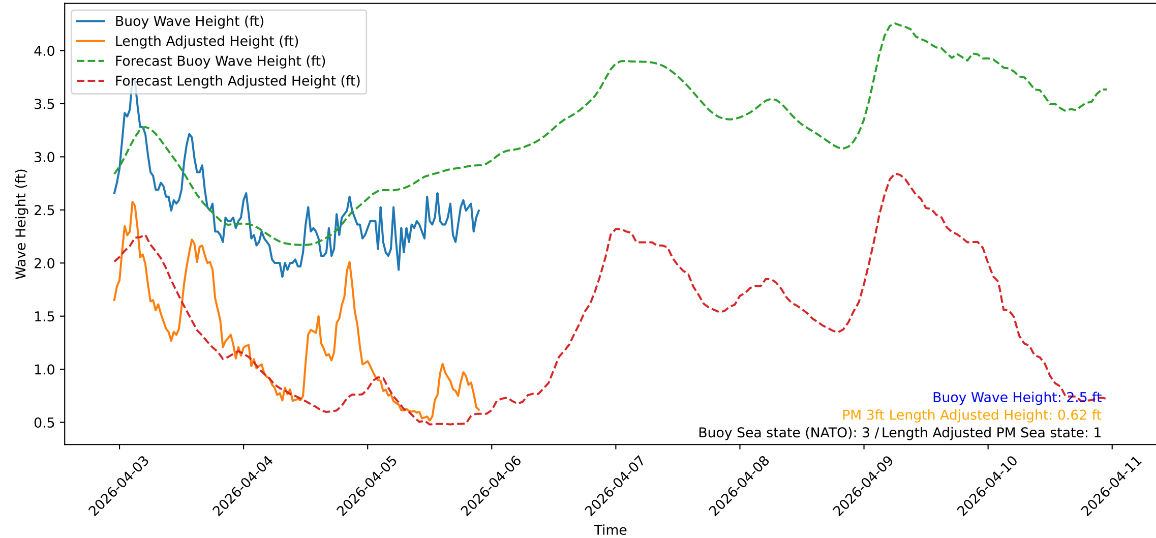
Wave Heights over Time for Red Beach at 2026-04-05 22:30:51
