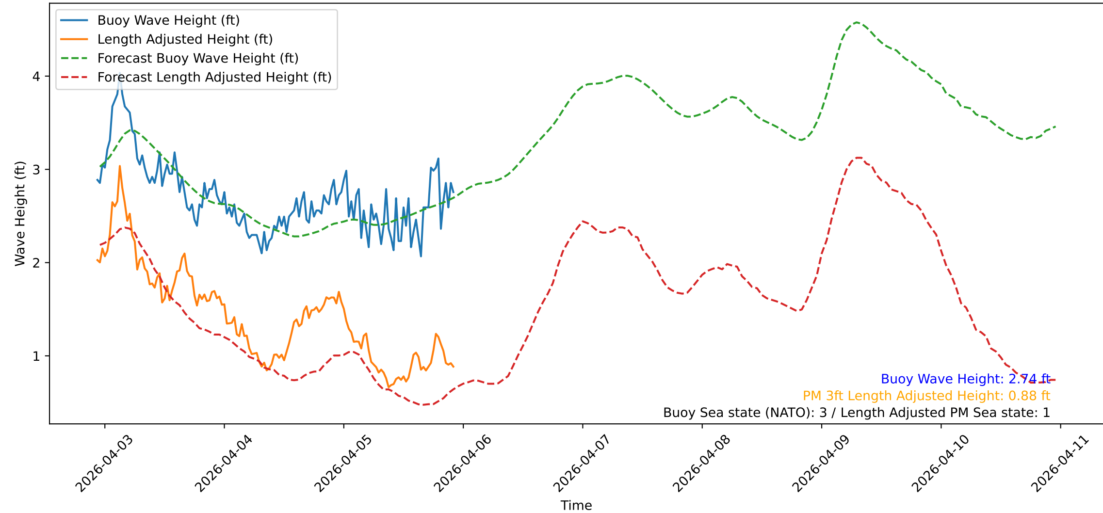
Wave Heights over Time for Oceanside Harbor at 2026-04-05 22:30:34
