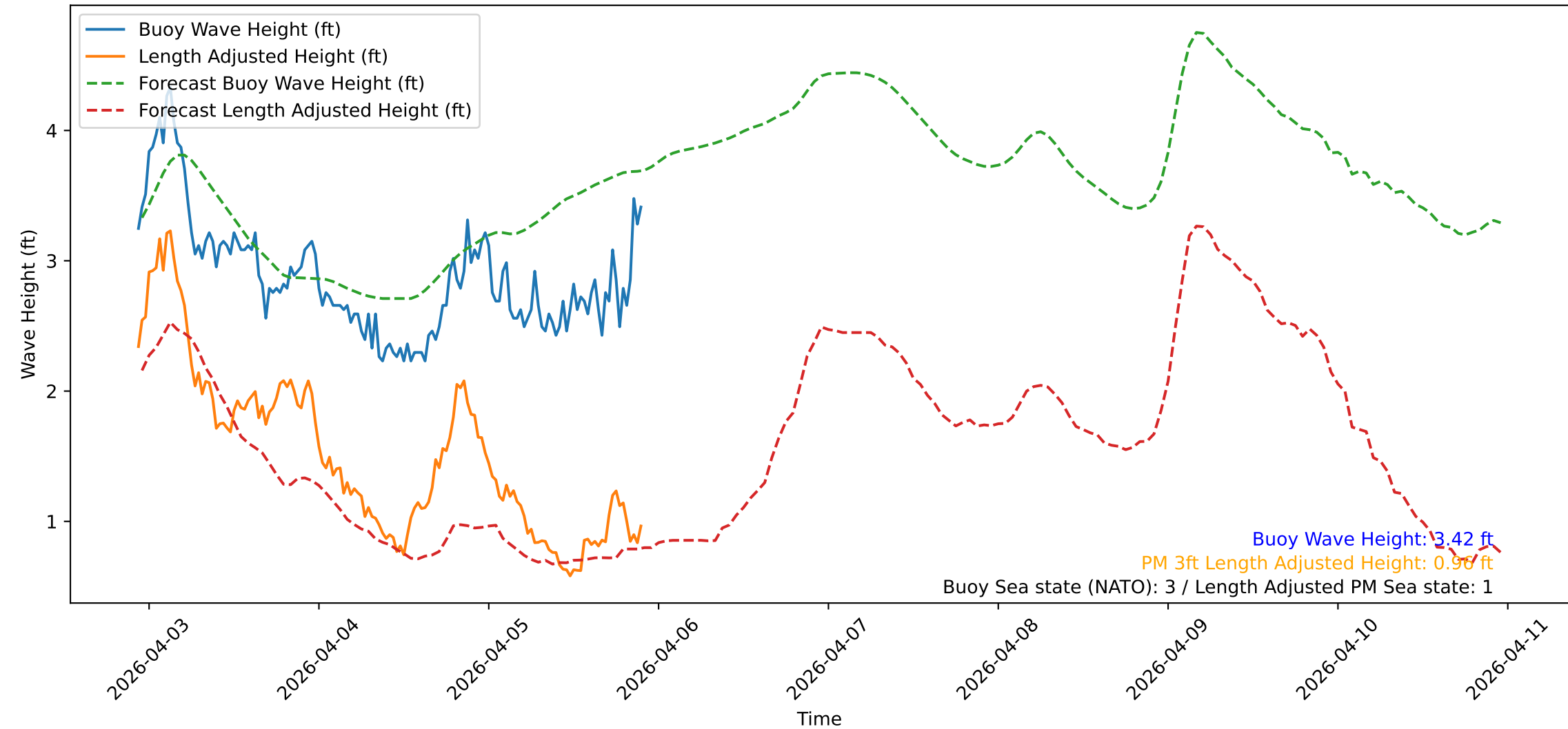
Wave Heights over Time for Green Beach at 2026-04-05 22:31:23
