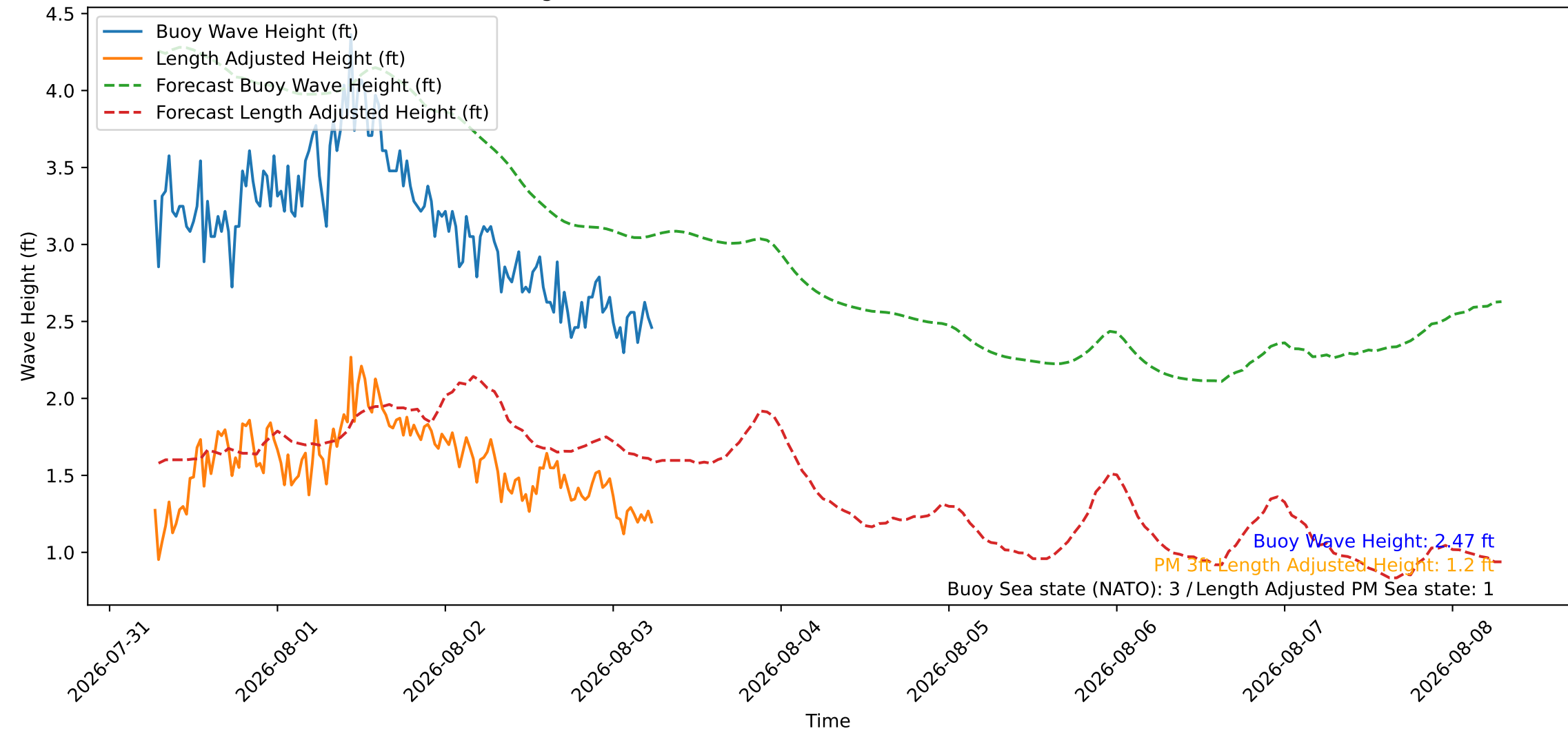
Wave Heights over Time for Oceanside Harbor at 2026-08-03 06:30:27
