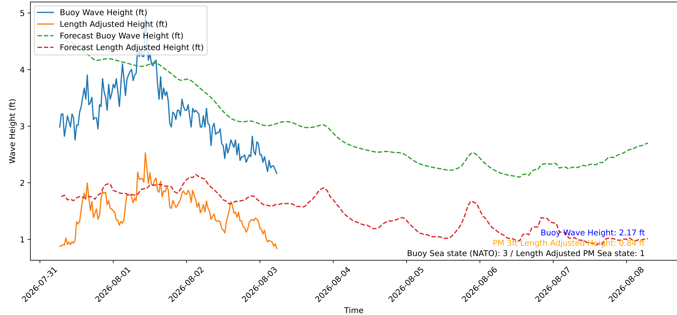
Wave Heights over Time for Green Beach at 2026-08-03 06:31:08
