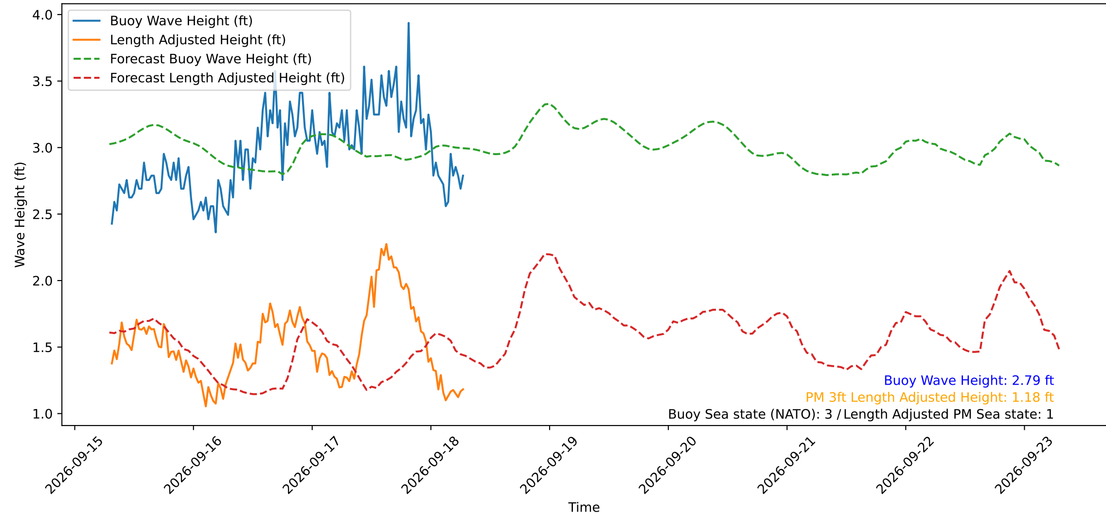
Wave Heights over Time for Oceanside Harbor at 2026-09-18 07:20:29
