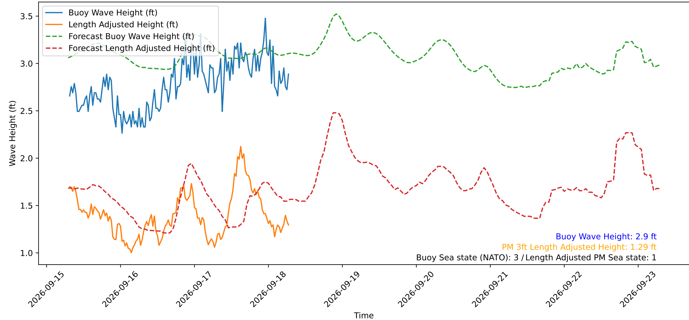
Wave Heights over Time for Green Beach at 2026-09-18 07:21:13
