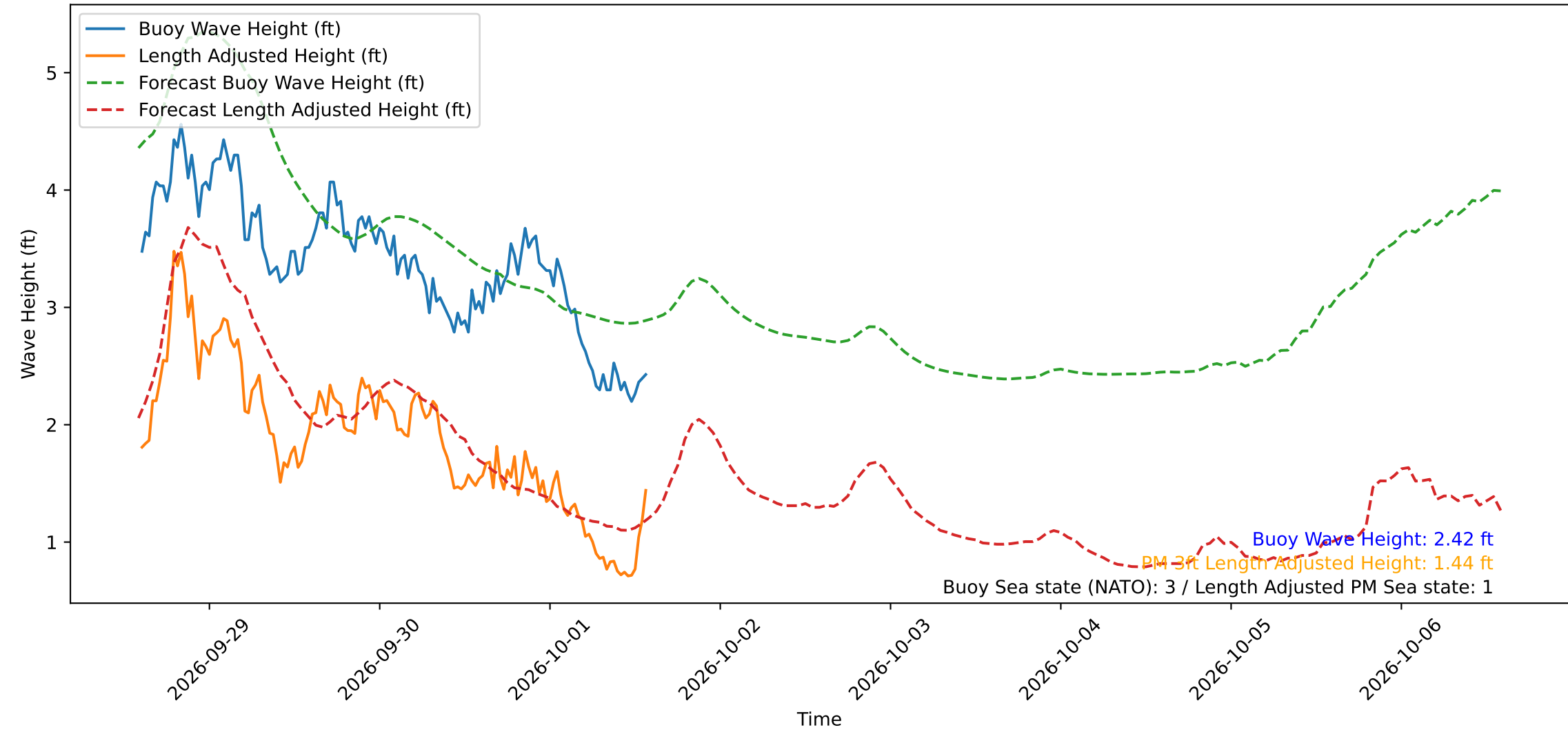
Wave Heights over Time for Green Beach at 2026-10-01 14:11:12
