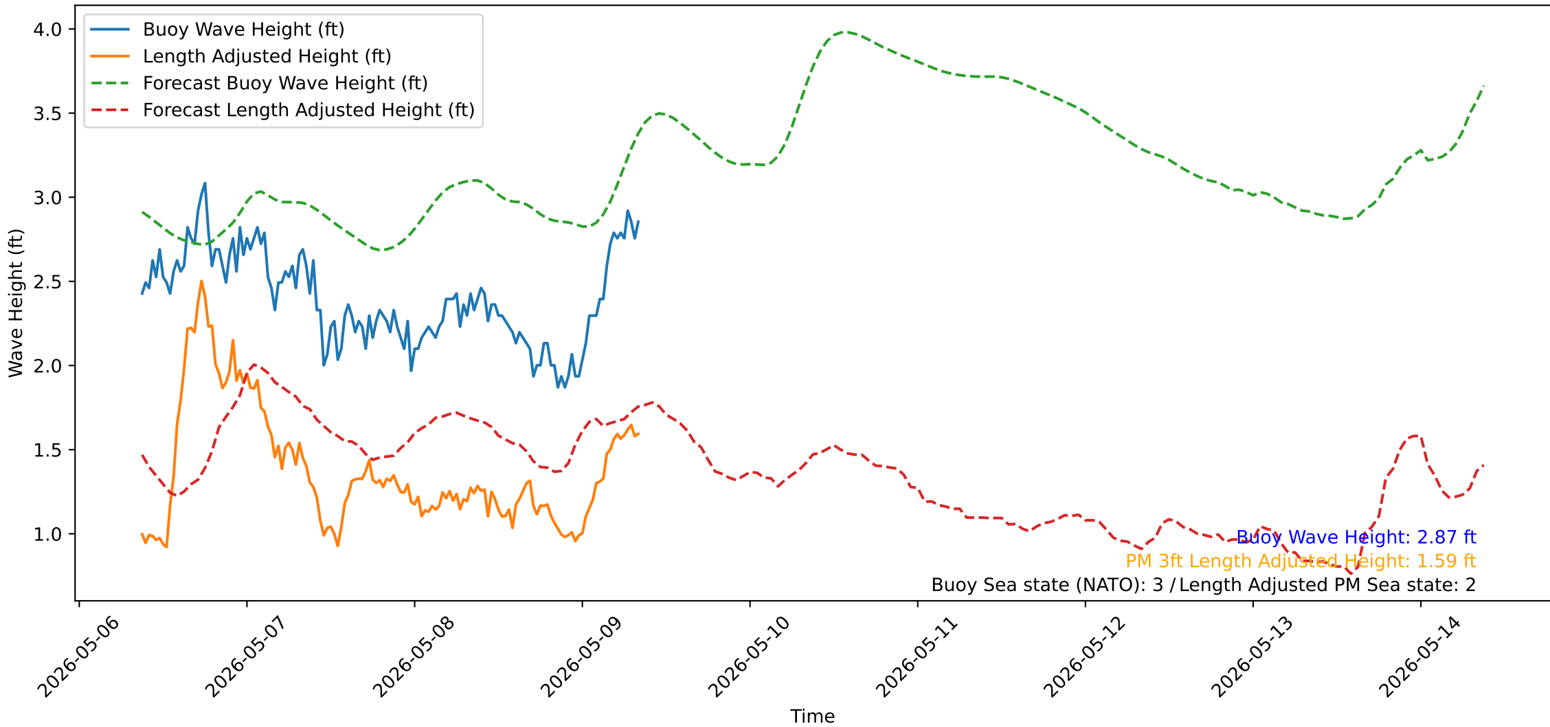
Wave Heights over Time for Oceanside Harbor at 2026-05-09 08:50:31
