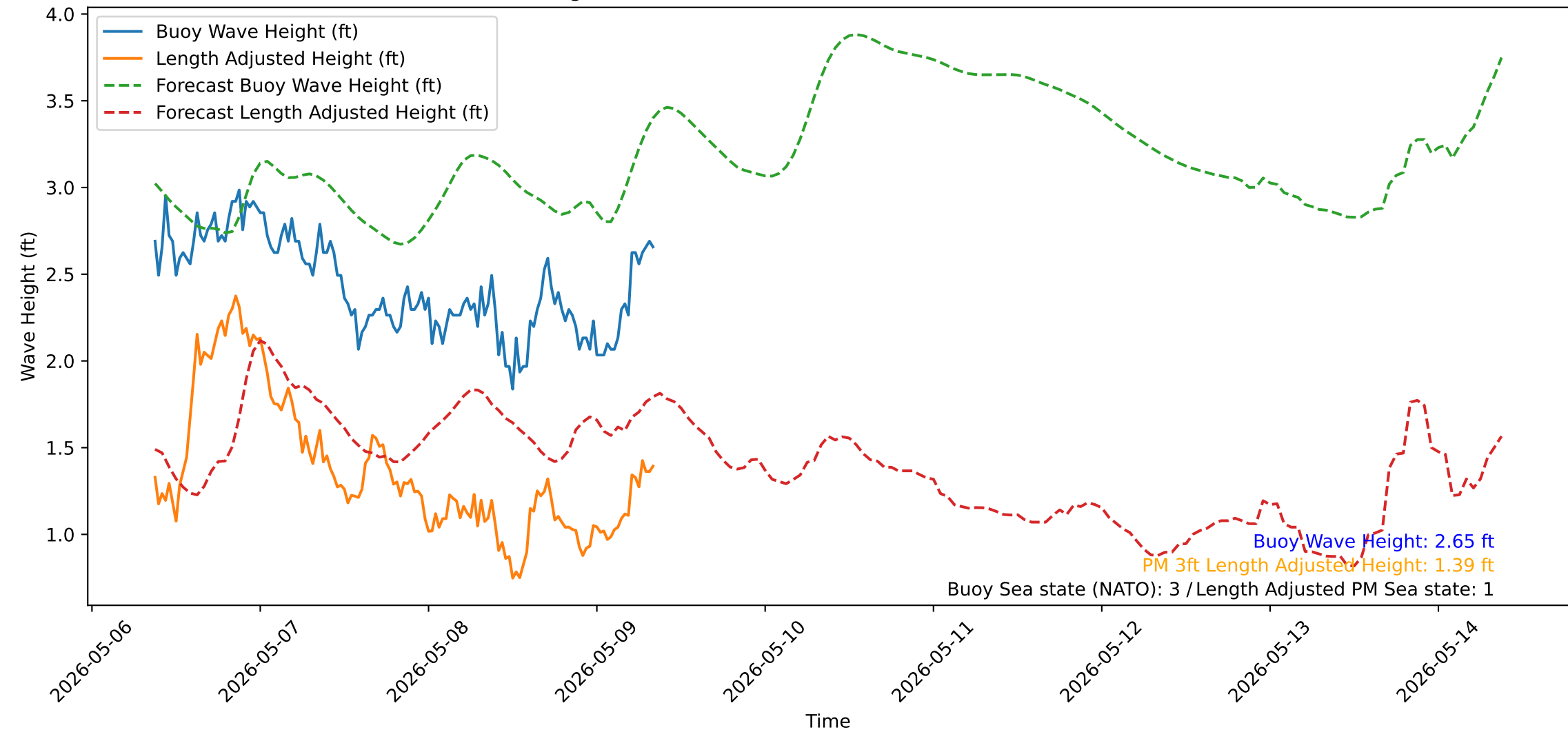
Wave Heights over Time for Green Beach at 2026-05-09 08:51:15
