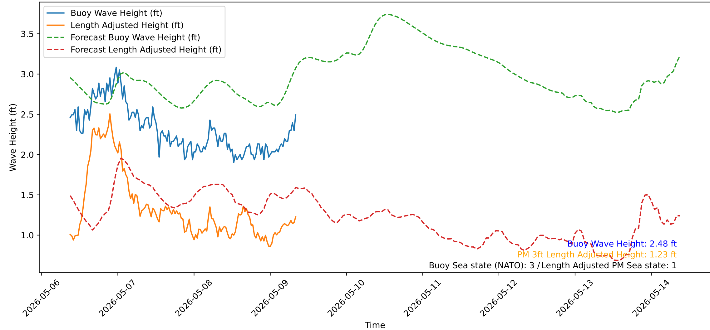
Wave Heights over Time for Red Beach at 2026-05-09 08:50:52
