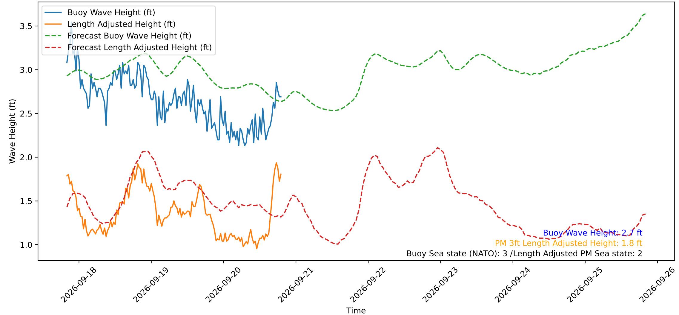
Wave Heights over Time for Oceanside Harbor at 2026-09-20 19:50:30
