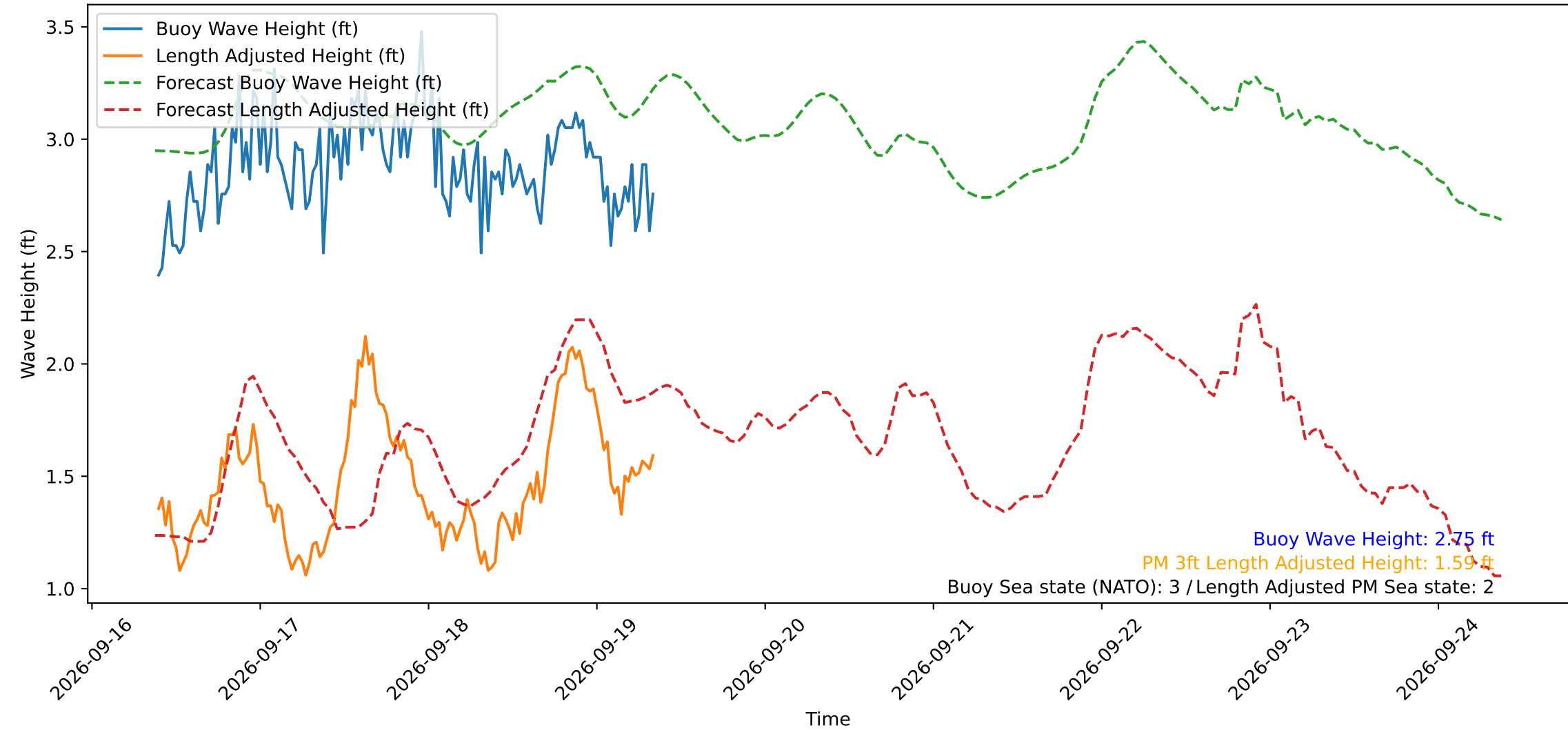
Wave Heights over Time for Green Beach at 2026-09-19 09:01:11
