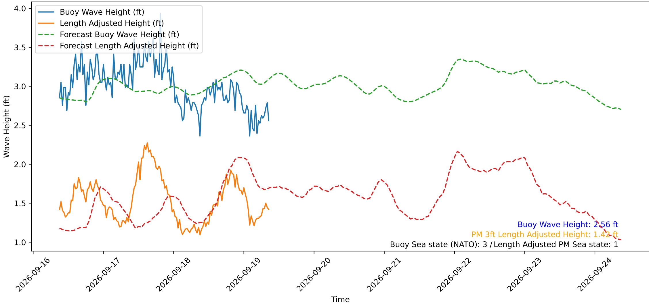
Wave Heights over Time for Oceanside Harbor at 2026-09-19 09:00:29
