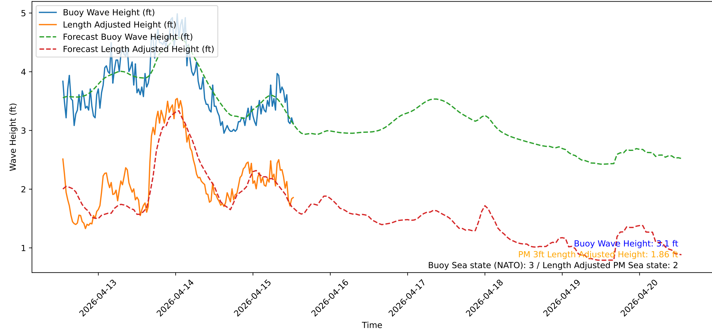
Wave Heights over Time for Green Beach at 2026-04-15 13:11:13
