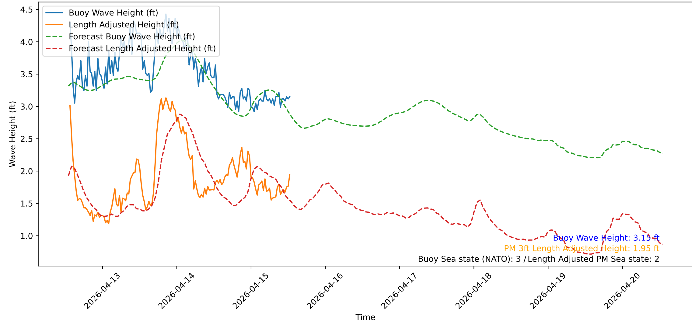
Wave Heights over Time for Red Beach at 2026-04-15 13:10:51
