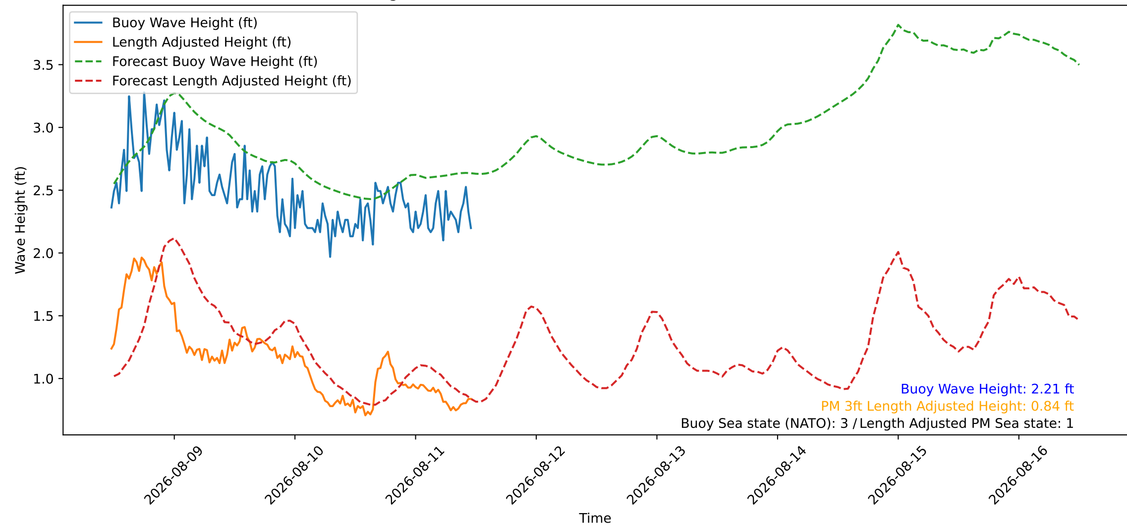
Wave Heights over Time for Oceanside Harbor at 2026-08-11 11:40:26
