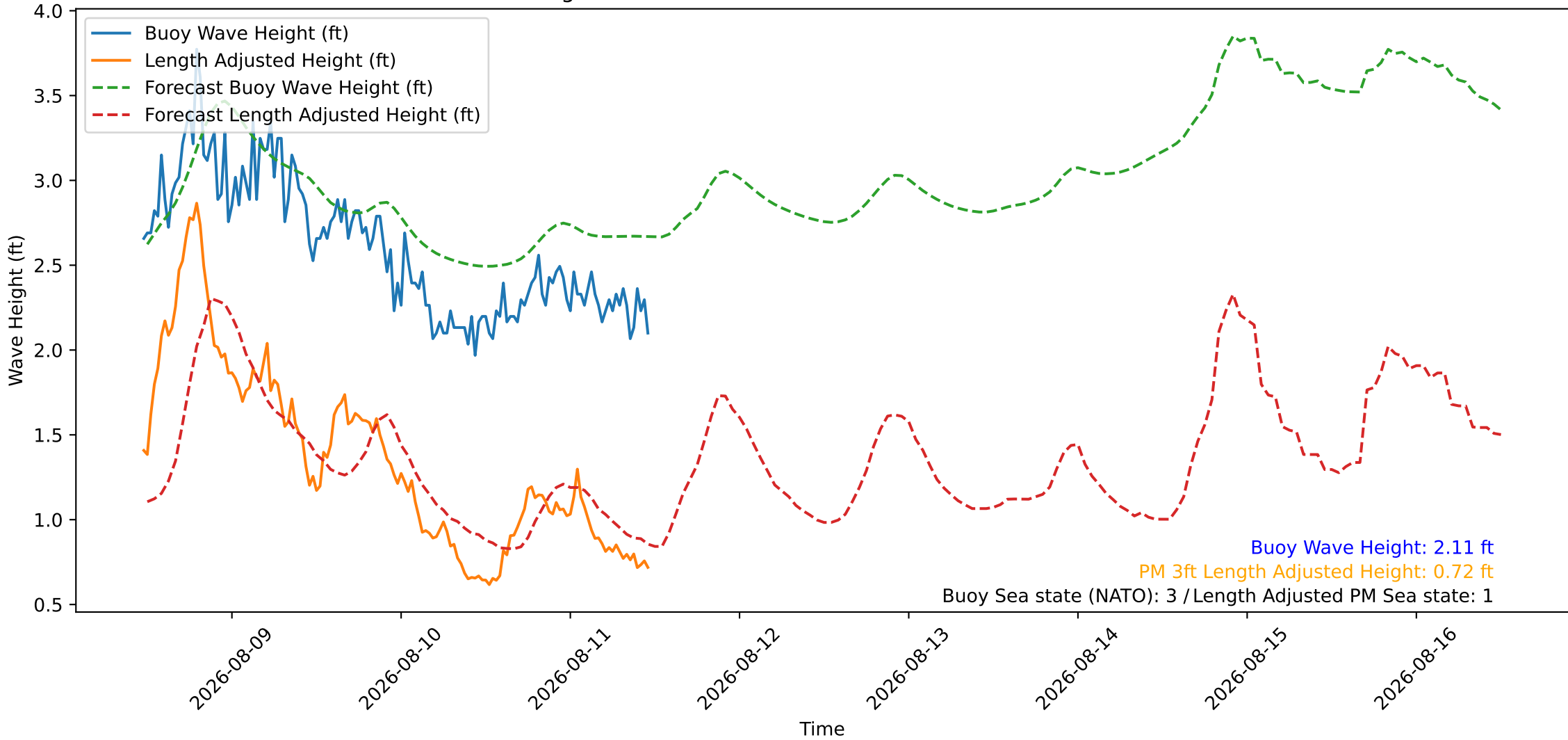
Wave Heights over Time for Green Beach at 2026-08-11 11:41:08
