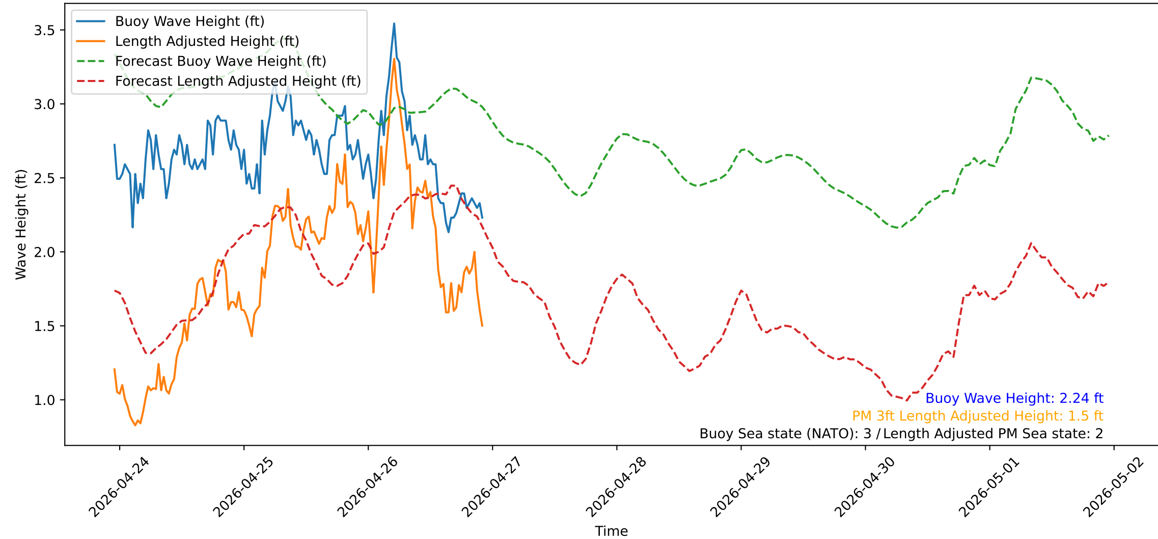
Wave Heights over Time for Red Beach at 2026-04-26 22:50:52
