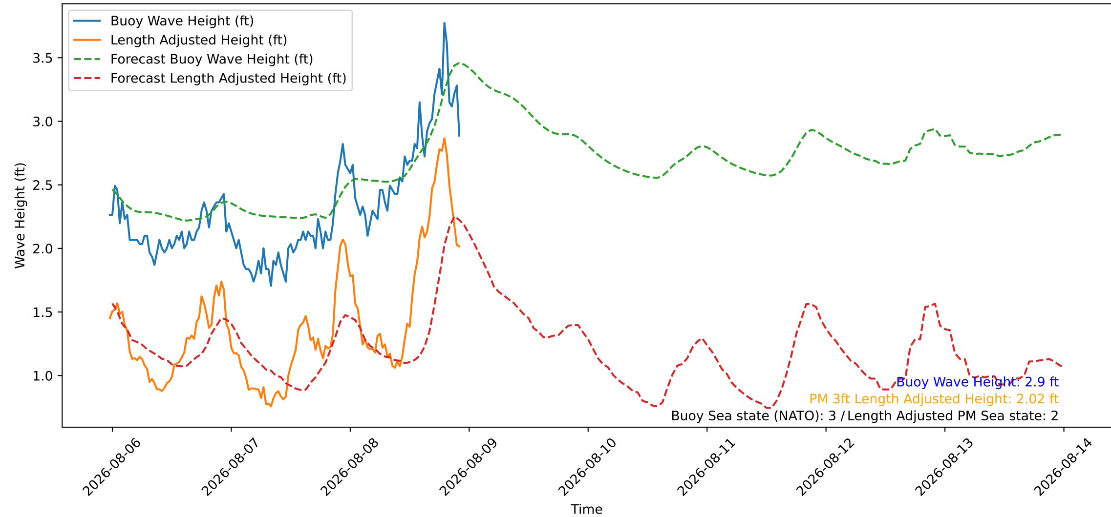
Wave Heights over Time for Green Beach at 2026-08-08 23:31:09
