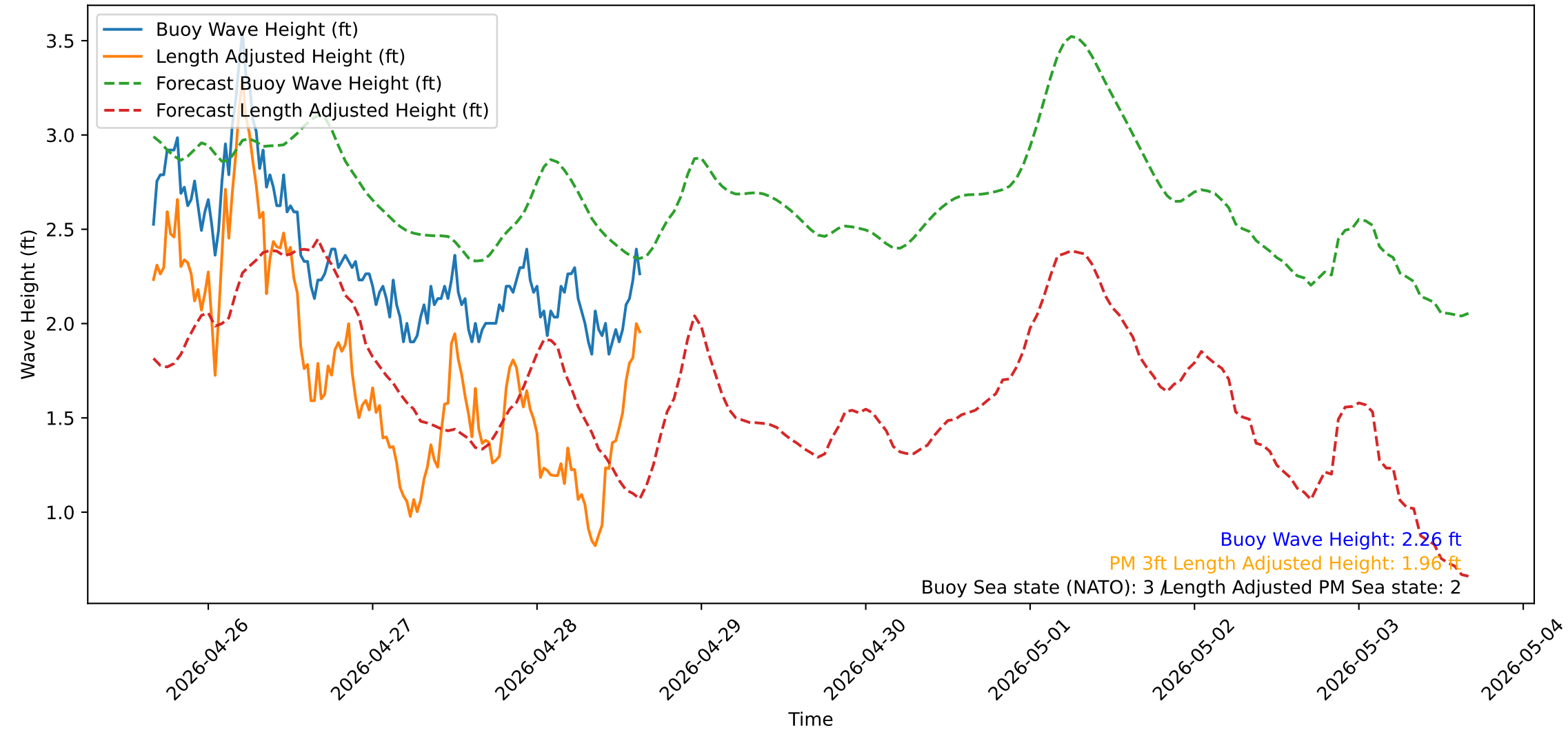
Wave Heights over Time for Red Beach at 2026-04-28 15:40:51
