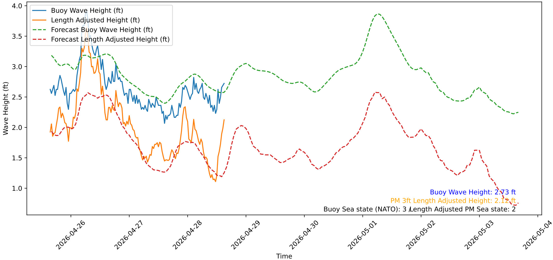
Wave Heights over Time for Oceanside Harbor at 2026-04-28 15:40:31
