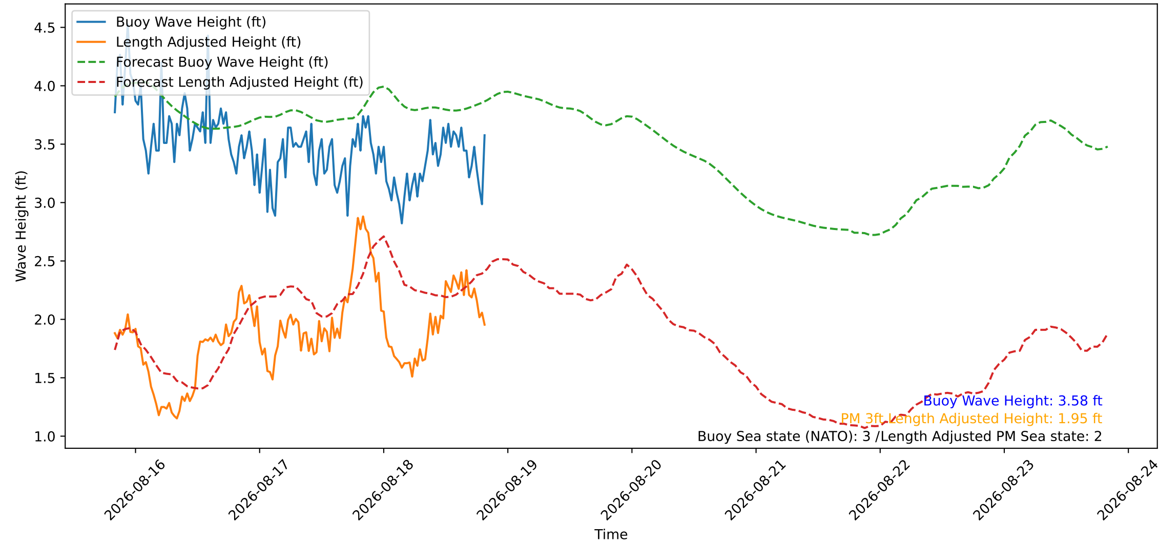
Wave Heights over Time for Oceanside Harbor at 2026-08-18 20:10:26
