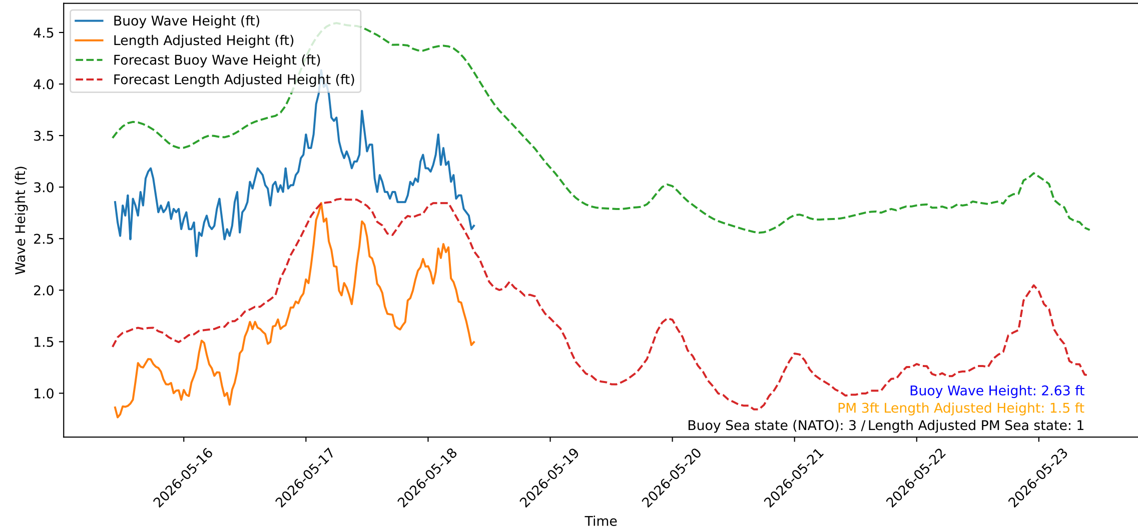
Wave Heights over Time for Red Beach at 2026-05-18 10:00:51
