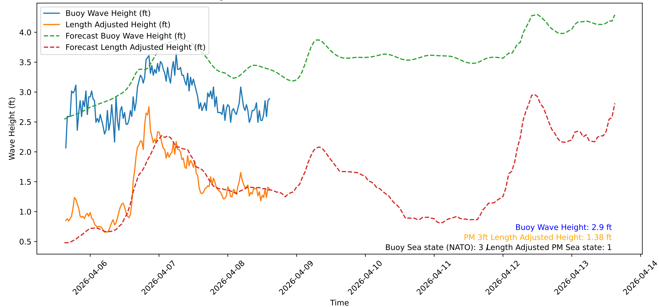
Wave Heights over Time for Oceanside Harbor at 2026-04-08 15:20:31
