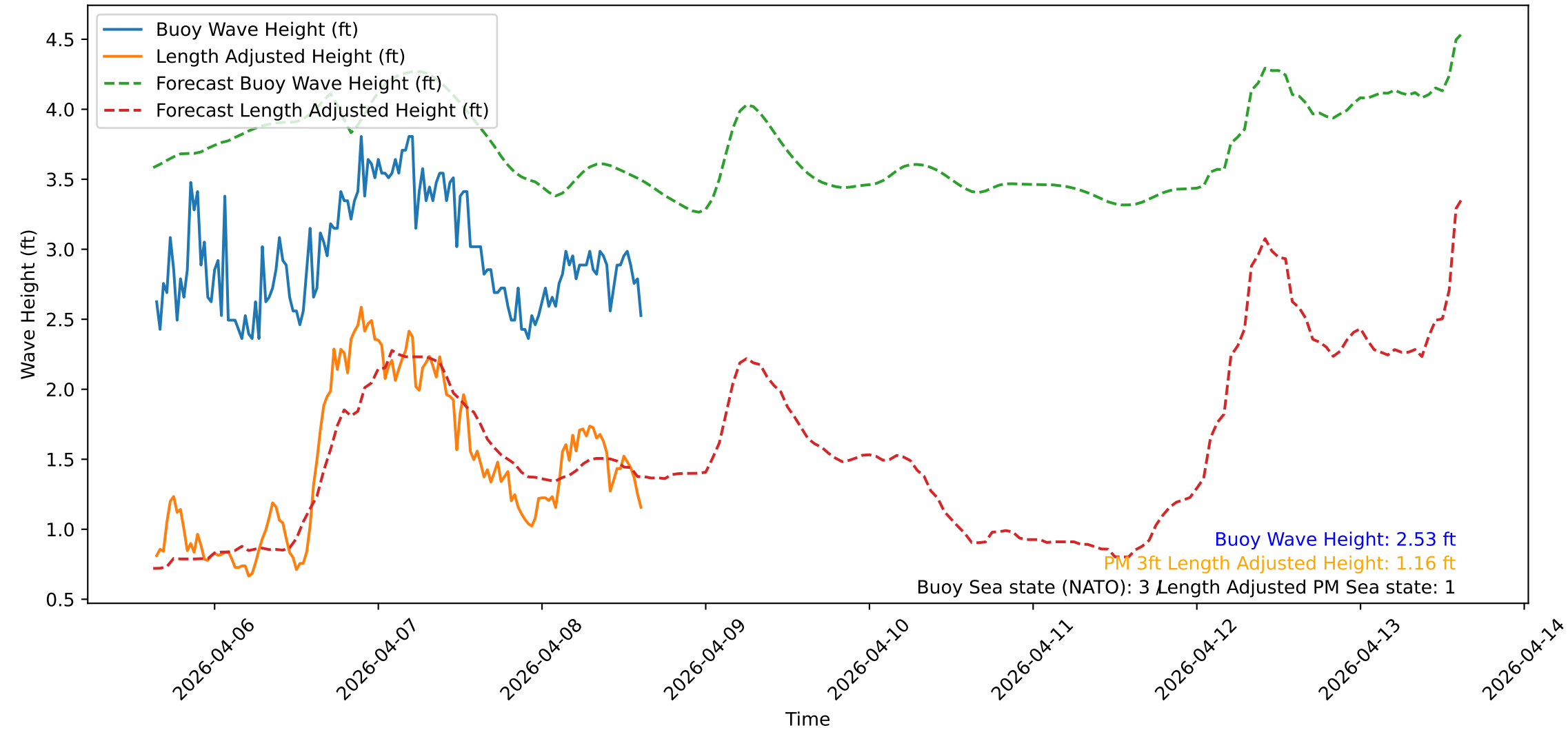
Wave Heights over Time for Green Beach at 2026-04-08 15:21:09
