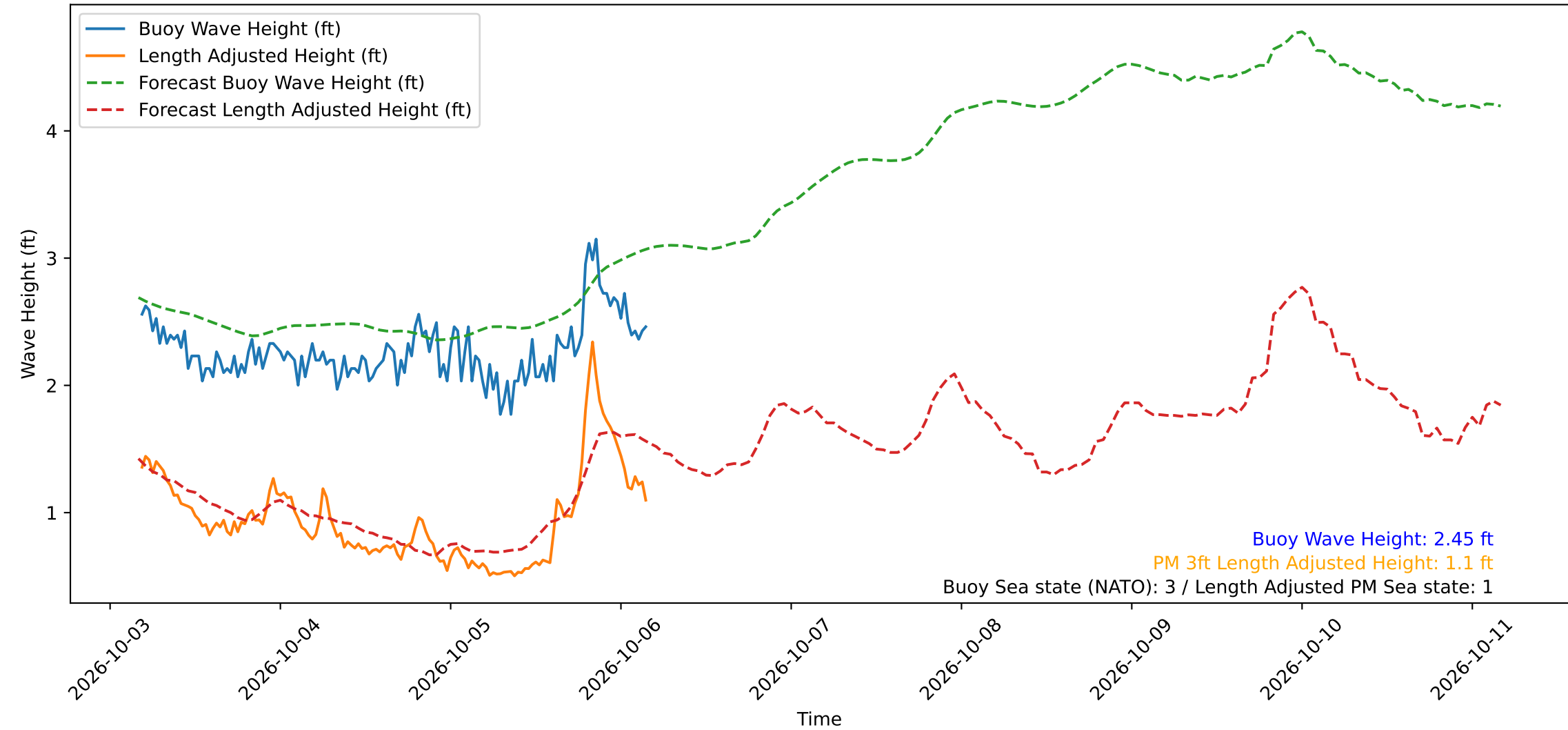
Wave Heights over Time for Green Beach at 2026-10-06 04:11:11
