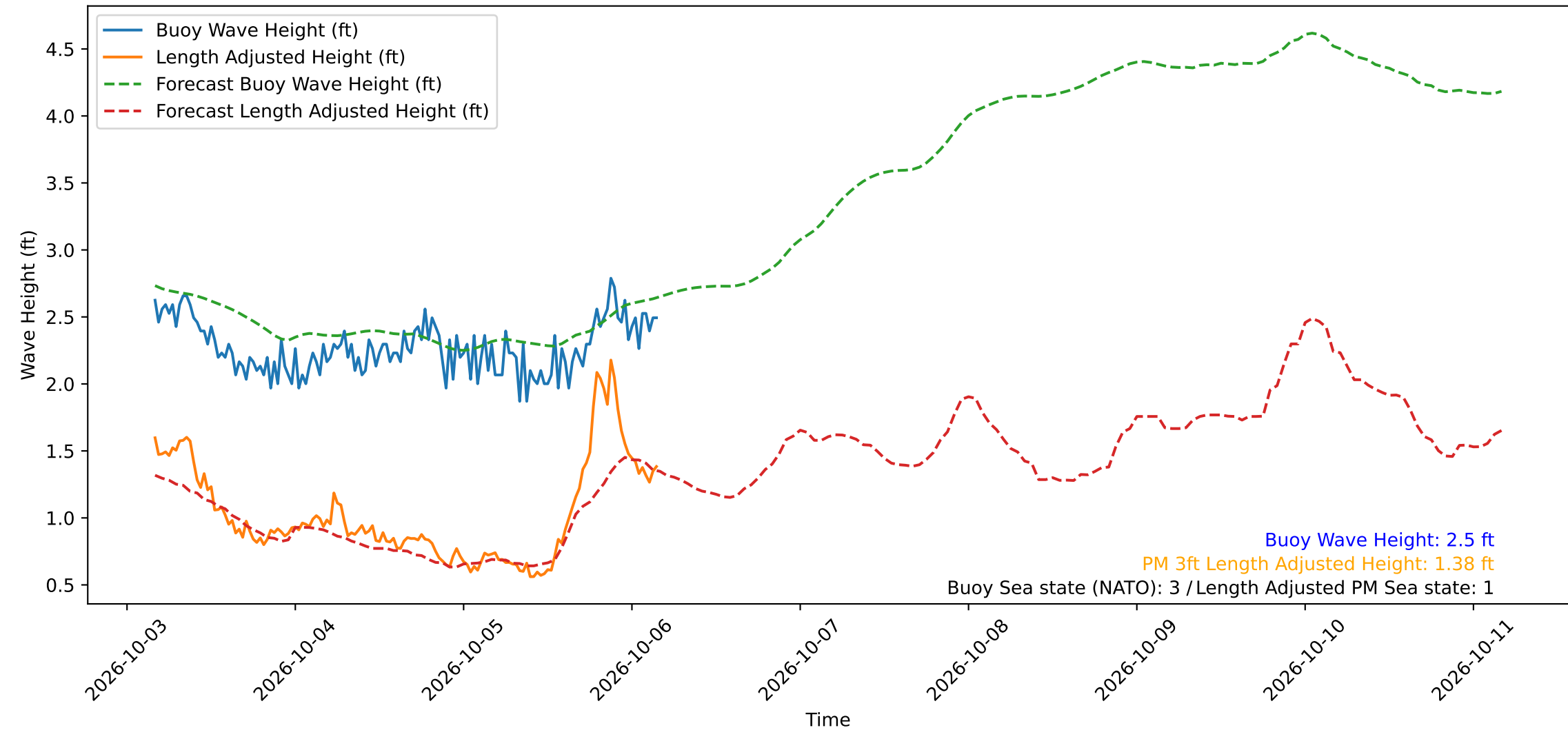
Wave Heights over Time for Oceanside Harbor at 2026-10-06 04:10:29
