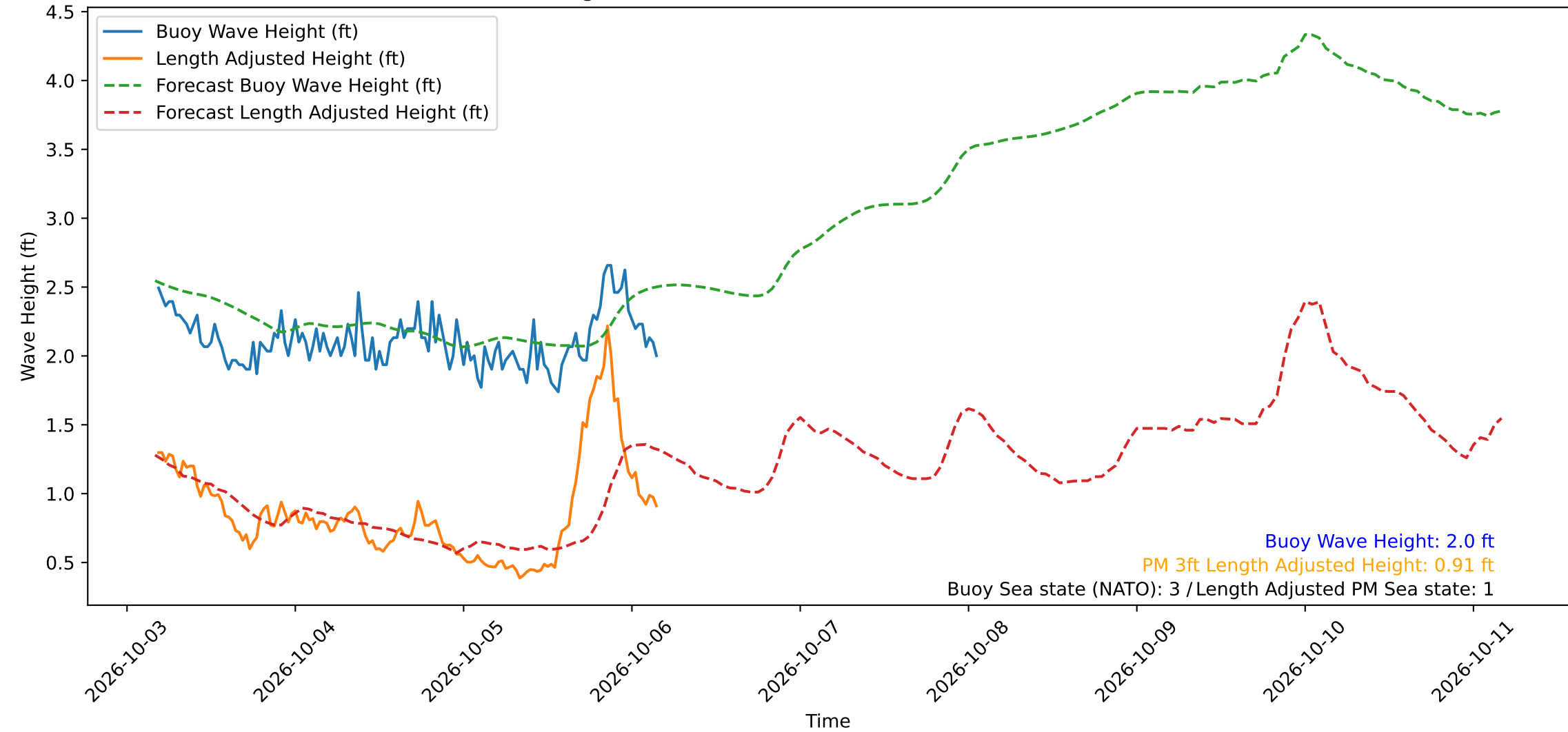
Wave Heights over Time for Red Beach at 2026-10-06 04:10:49
