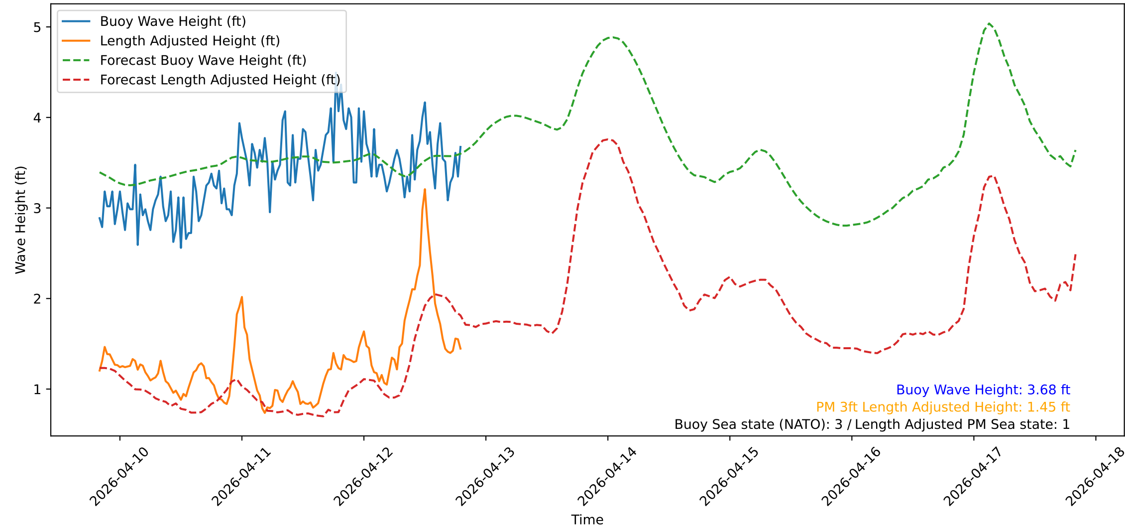
Wave Heights over Time for Green Beach at 2026-04-12 20:01:13
