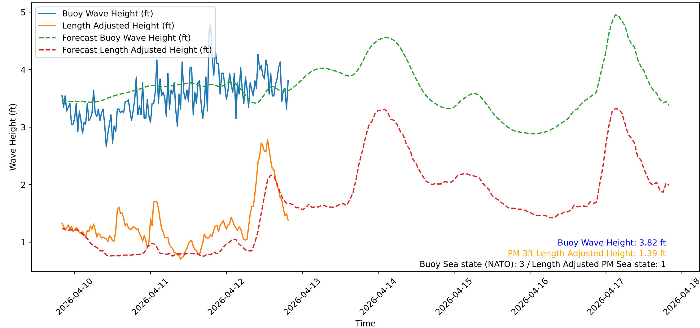
Wave Heights over Time for Oceanside Harbor at 2026-04-12 20:00:31
