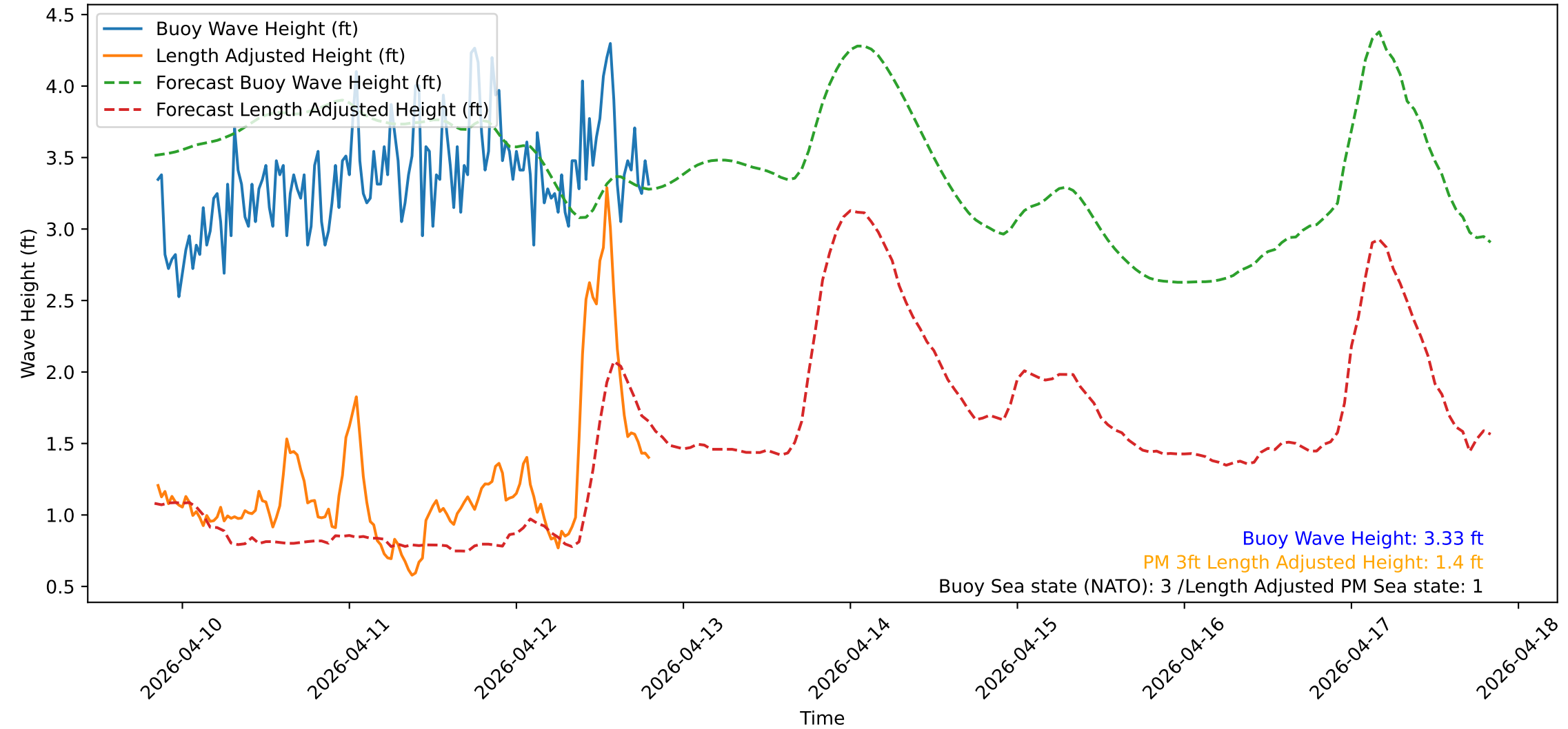
Wave Heights over Time for Red Beach at 2026-04-12 20:00:50
