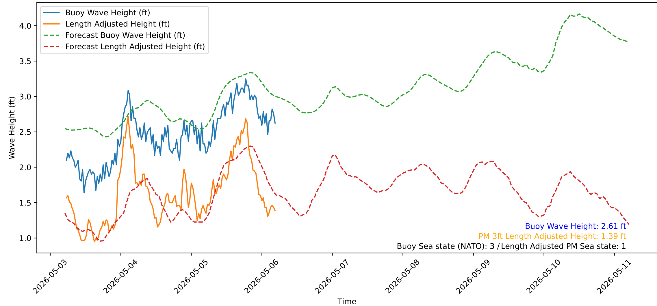
Wave Heights over Time for Oceanside Harbor at 2026-05-06 05:20:31
