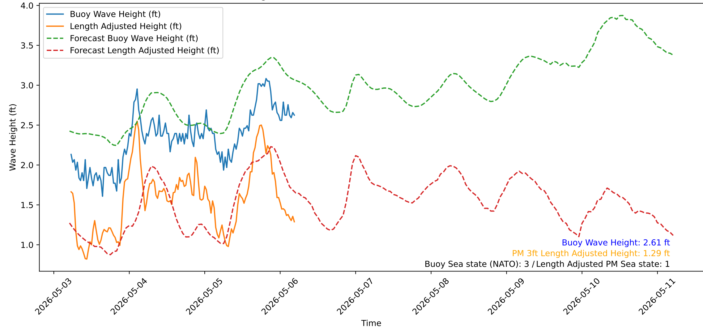
Wave Heights over Time for Red Beach at 2026-05-06 05:20:52
