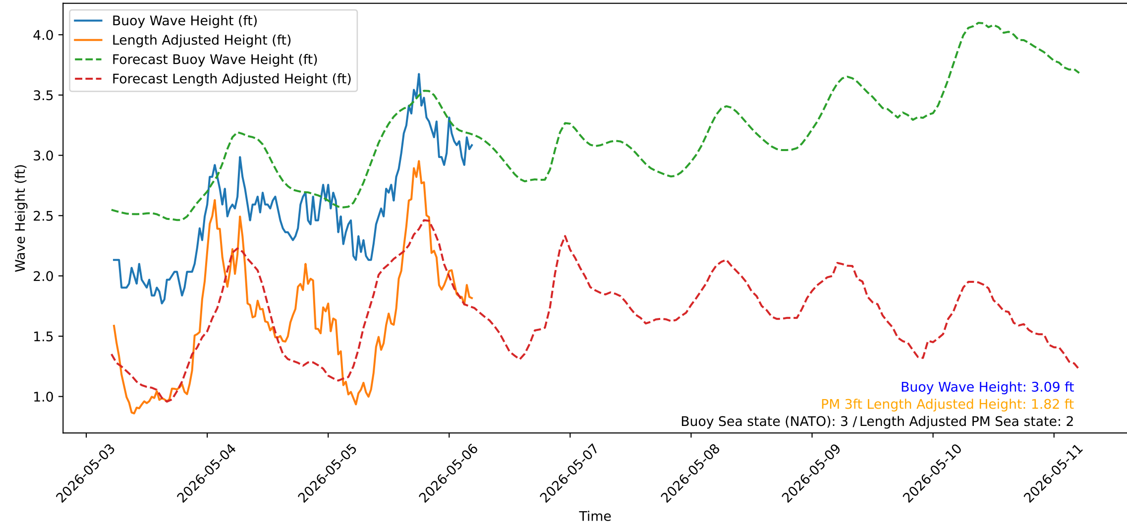
Wave Heights over Time for Green Beach at 2026-05-06 05:21:14
