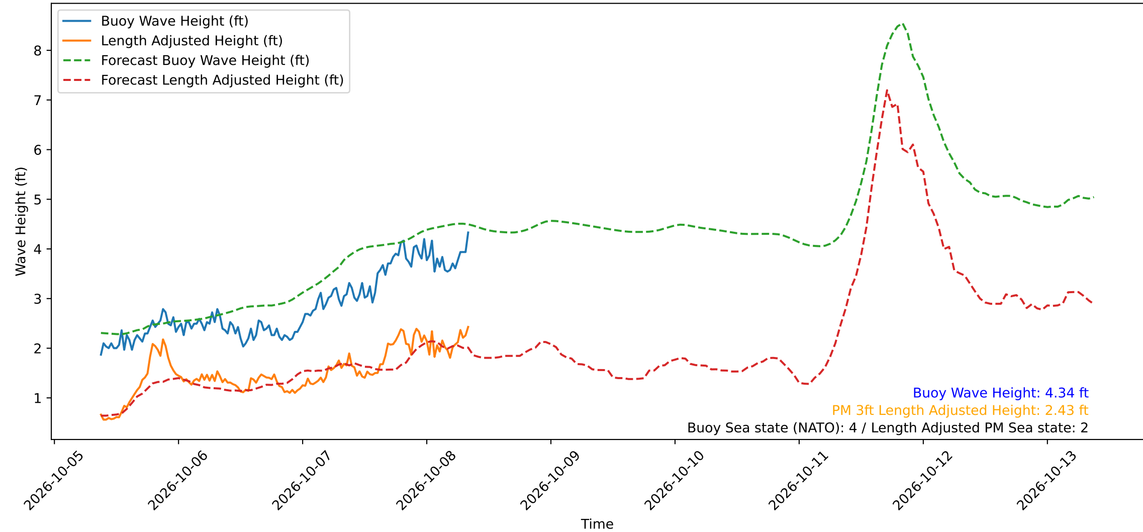
Wave Heights over Time for Oceanside Harbor at 2026-10-08 09:00:30
