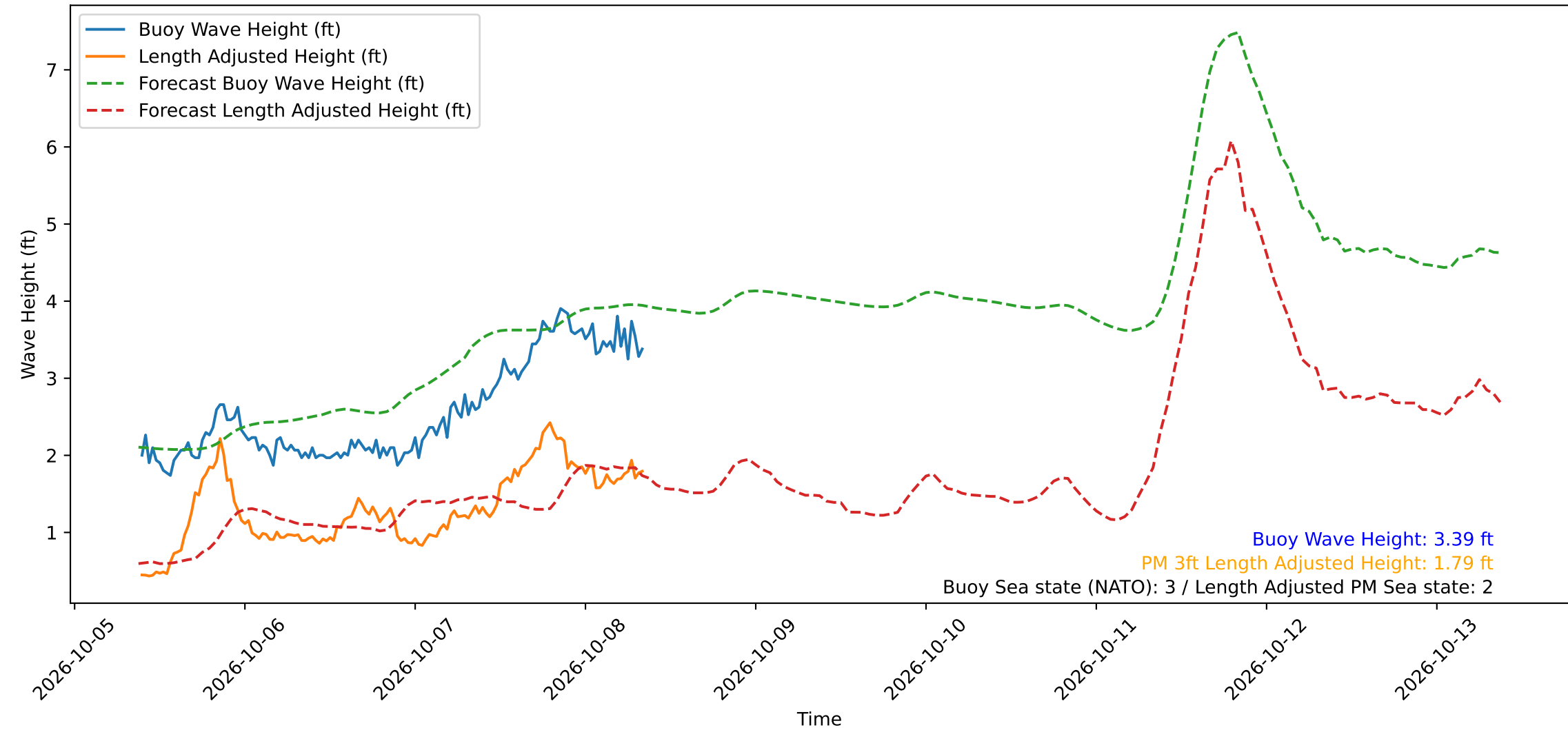
Wave Heights over Time for Red Beach at 2026-10-08 09:00:50
