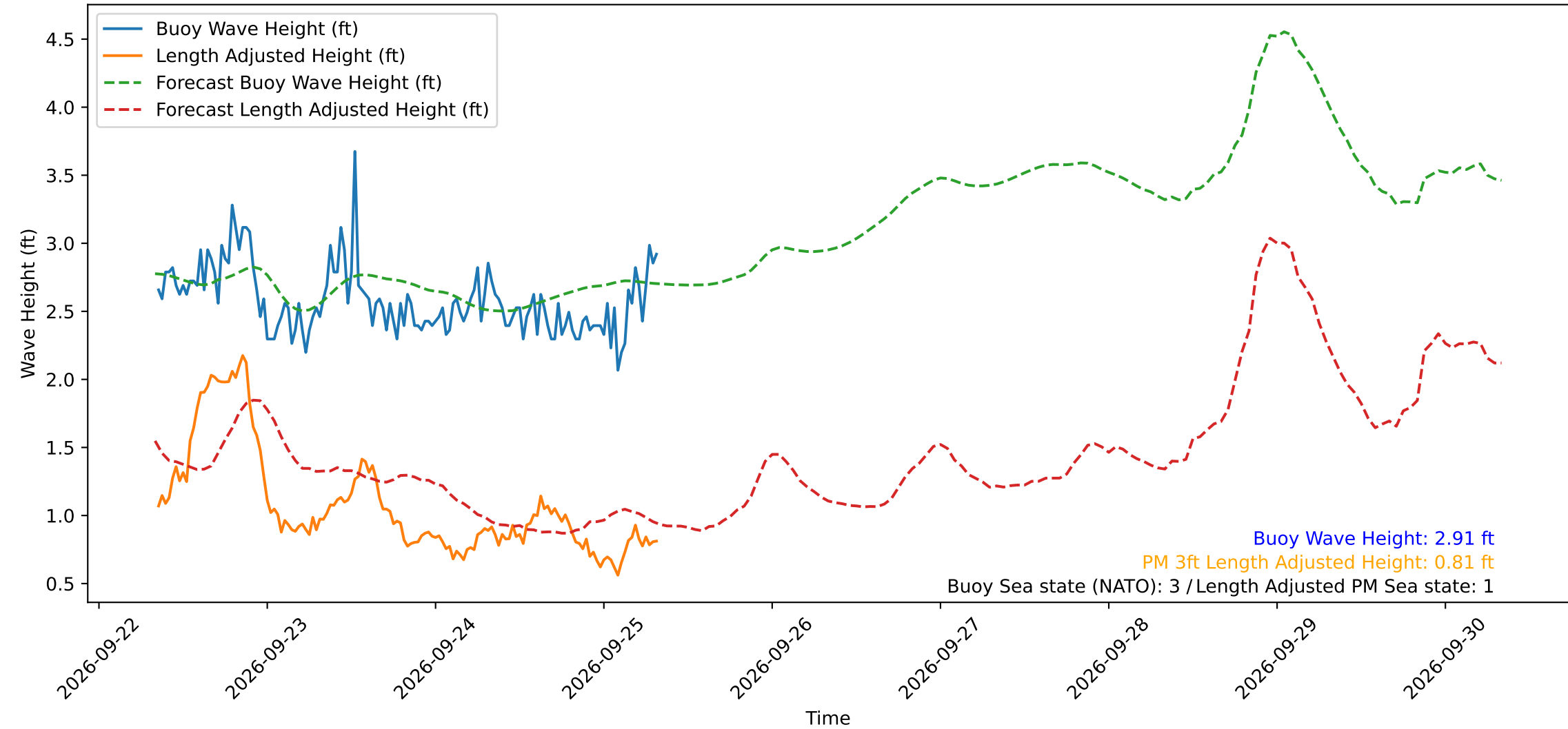
Wave Heights over Time for Red Beach at 2026-09-25 08:10:50
