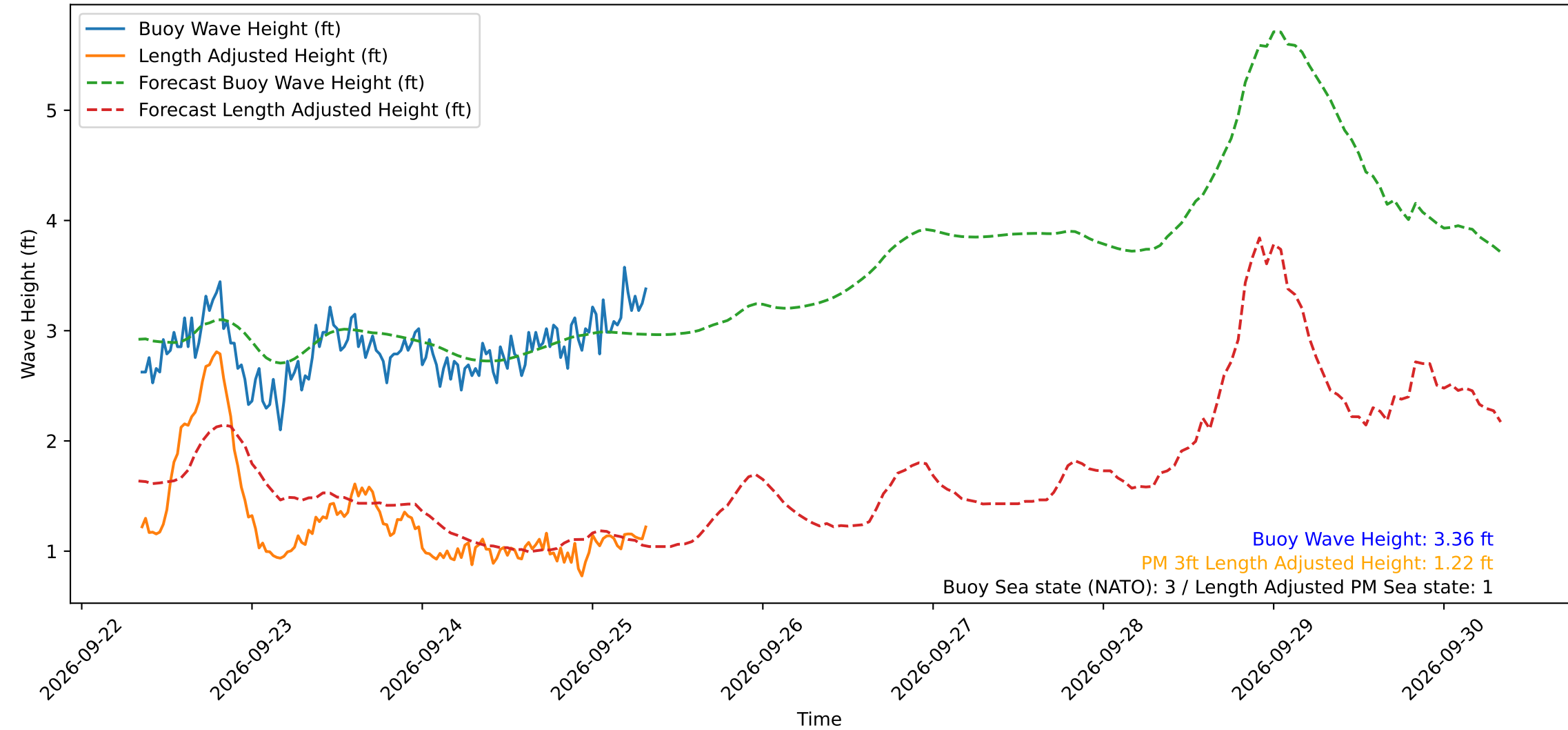
Wave Heights over Time for Green Beach at 2026-09-25 08:11:14
