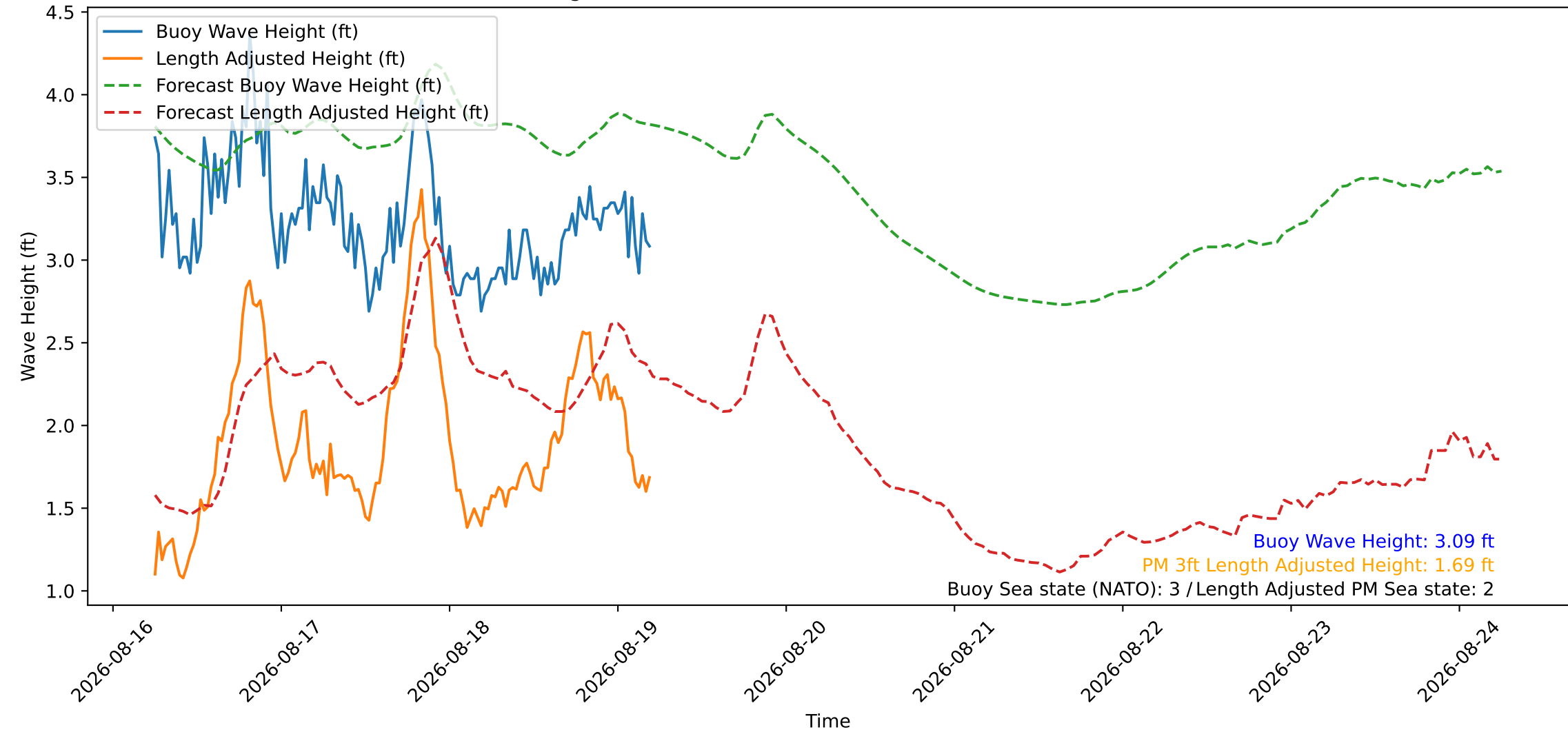
Wave Heights over Time for Green Beach at 2026-08-19 05:31:09
