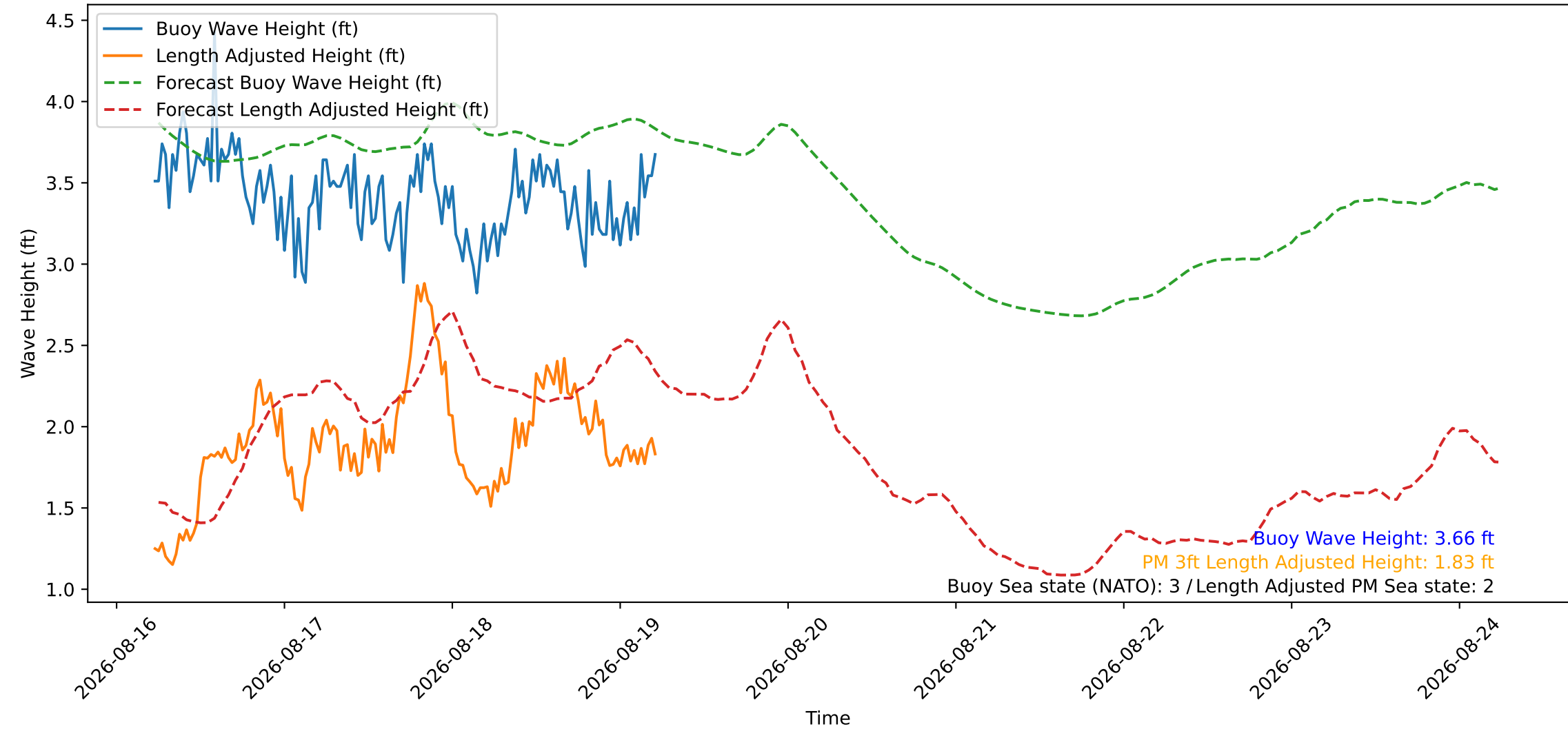
Wave Heights over Time for Oceanside Harbor at 2026-08-19 05:30:27
