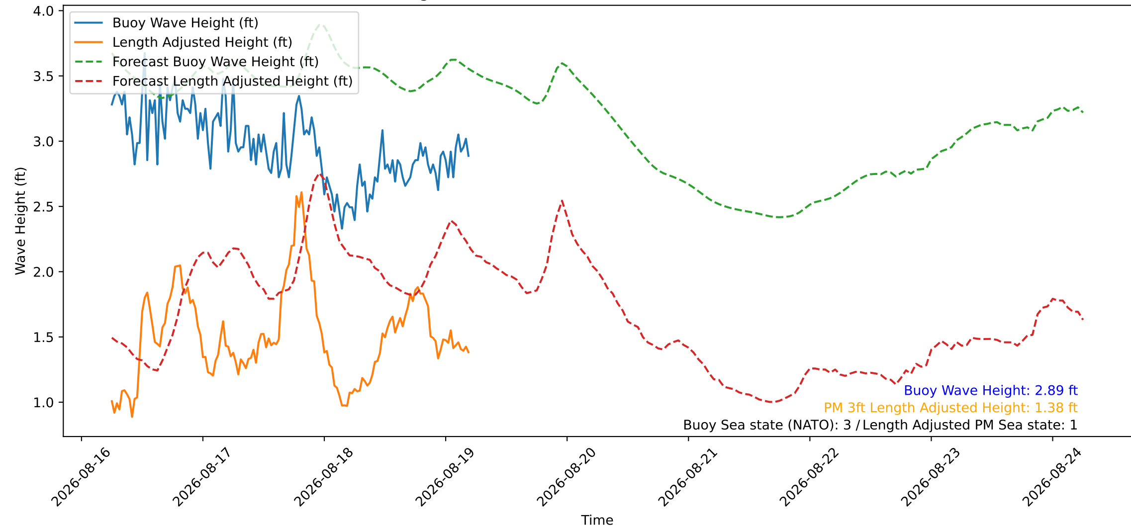
Wave Heights over Time for Red Beach at 2026-08-19 05:30:47
