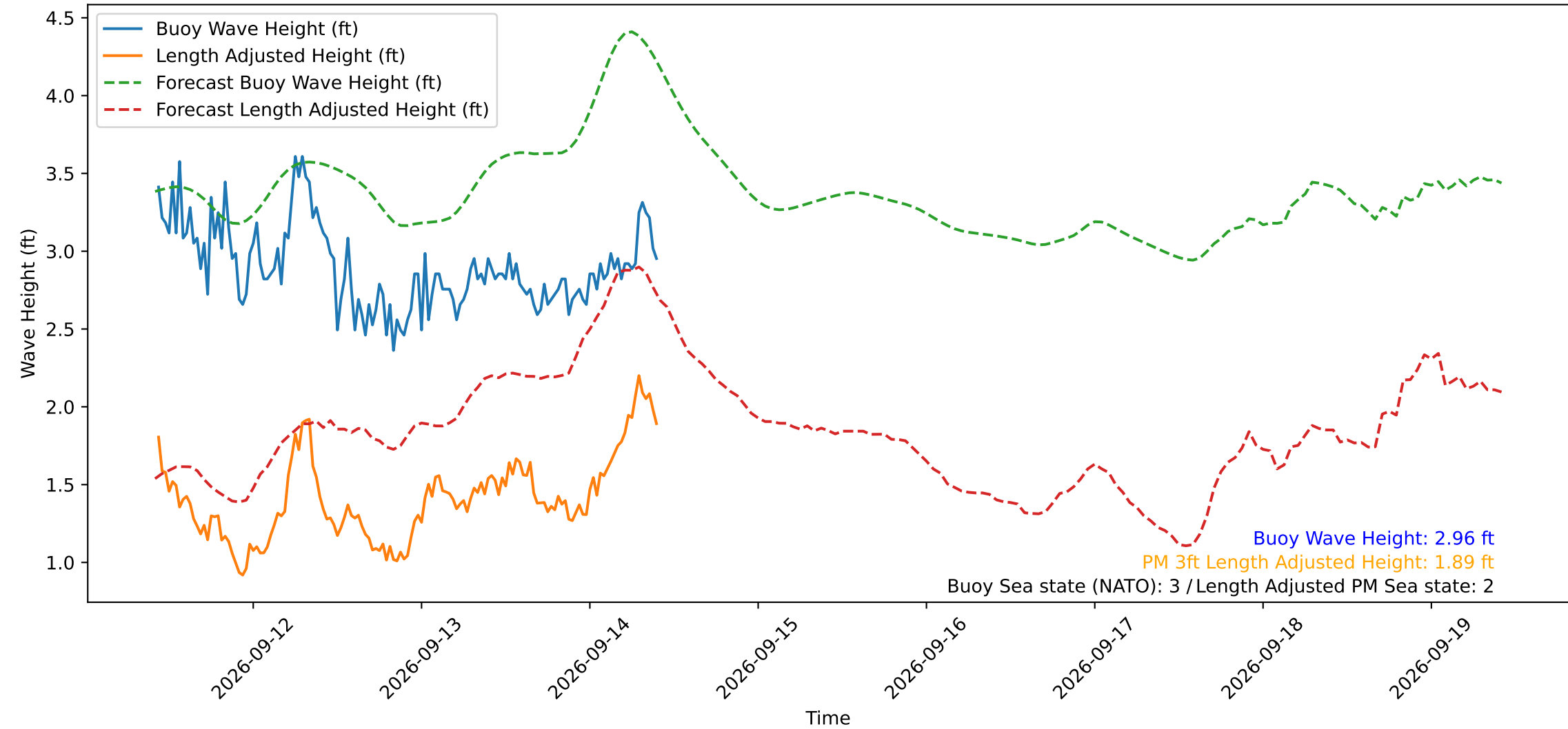
Wave Heights over Time for Green Beach at 2026-09-14 10:21:15
