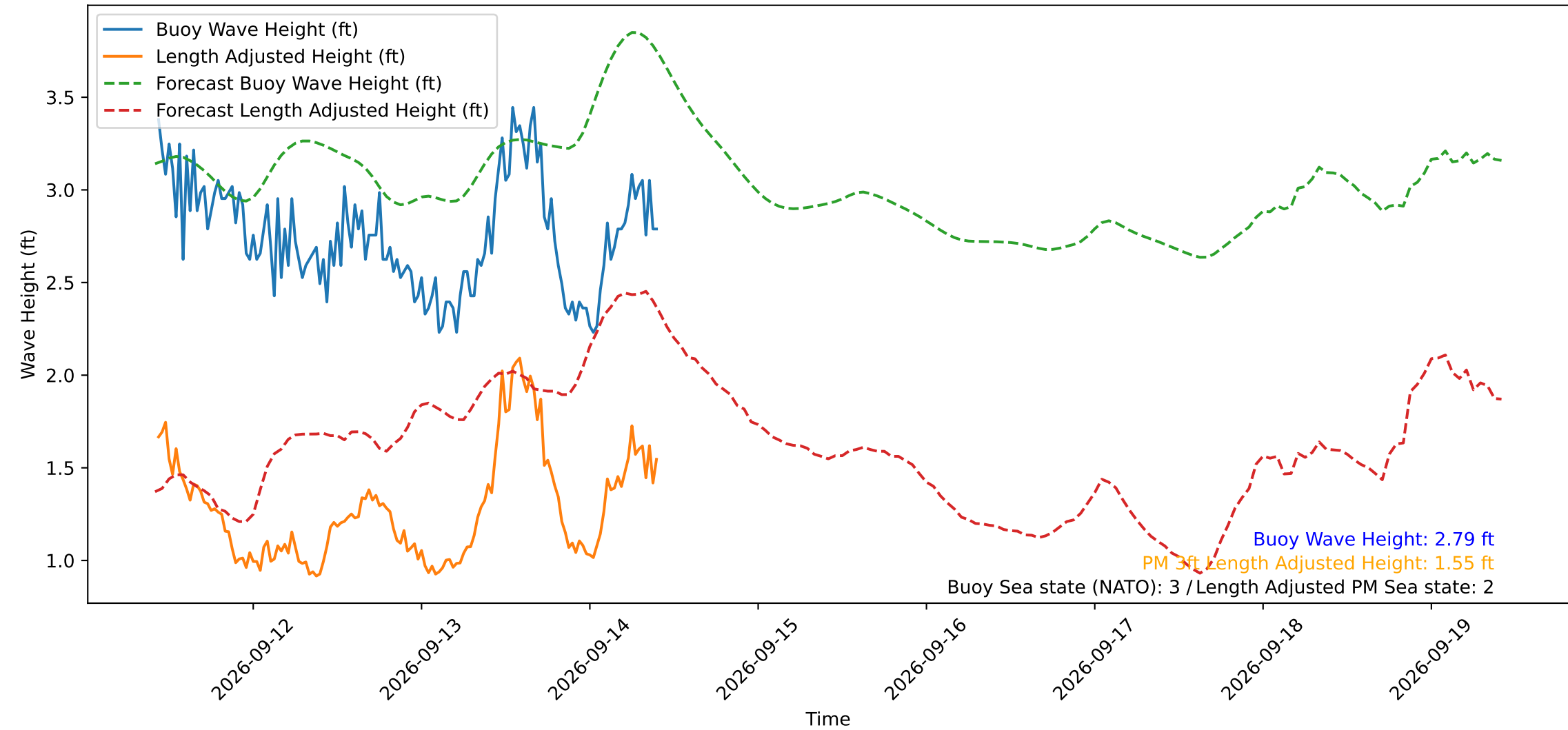
Wave Heights over Time for Red Beach at 2026-09-14 10:20:51
