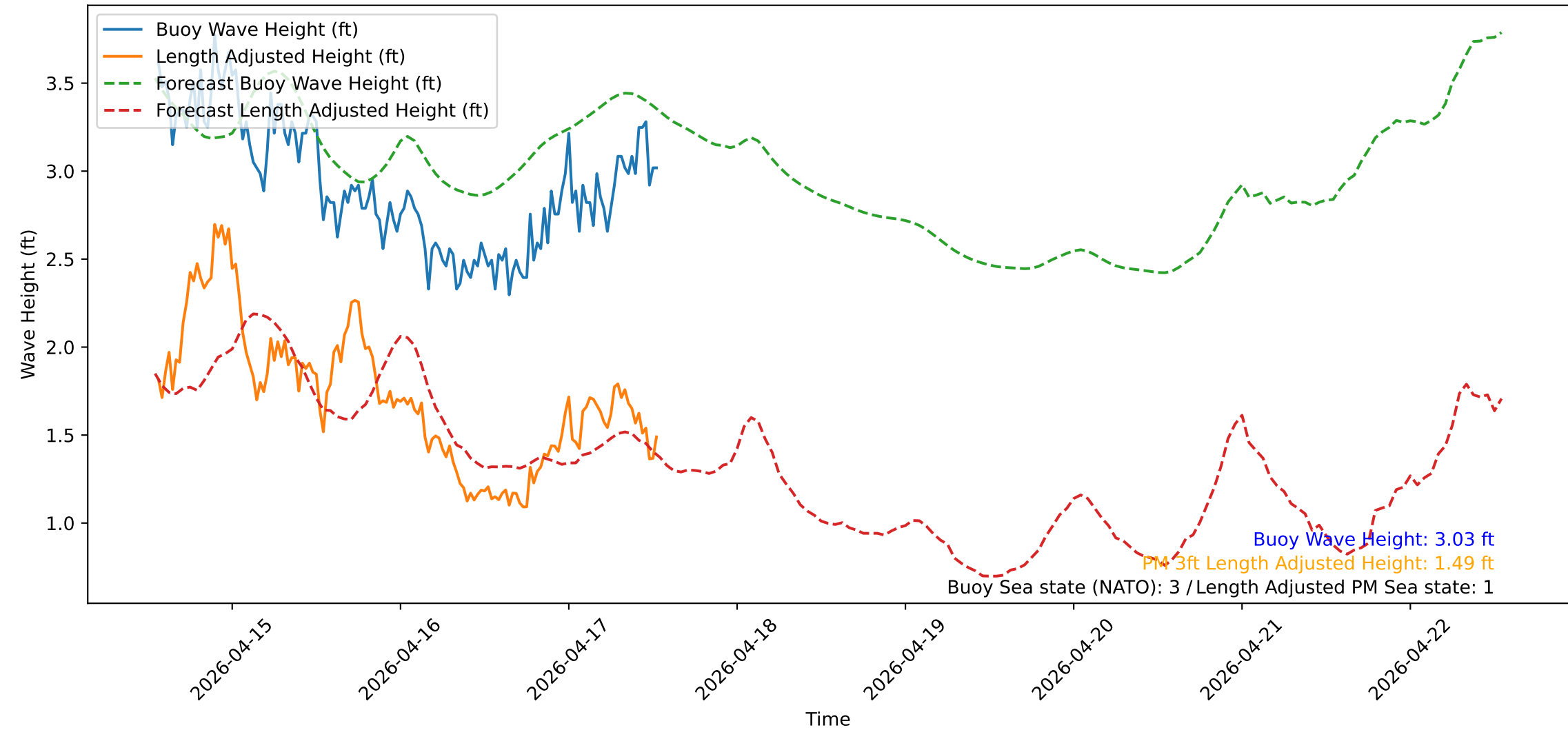
Wave Heights over Time for Oceanside Harbor at 2026-04-17 13:20:33
