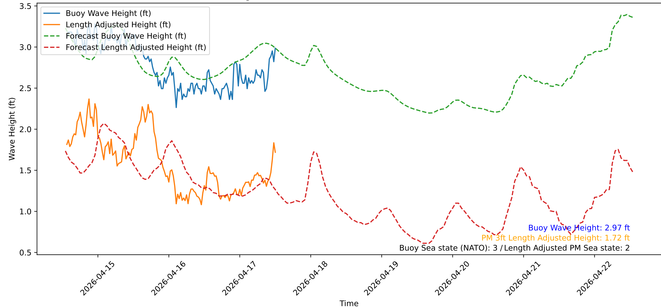
Wave Heights over Time for Red Beach at 2026-04-17 13:20:56
