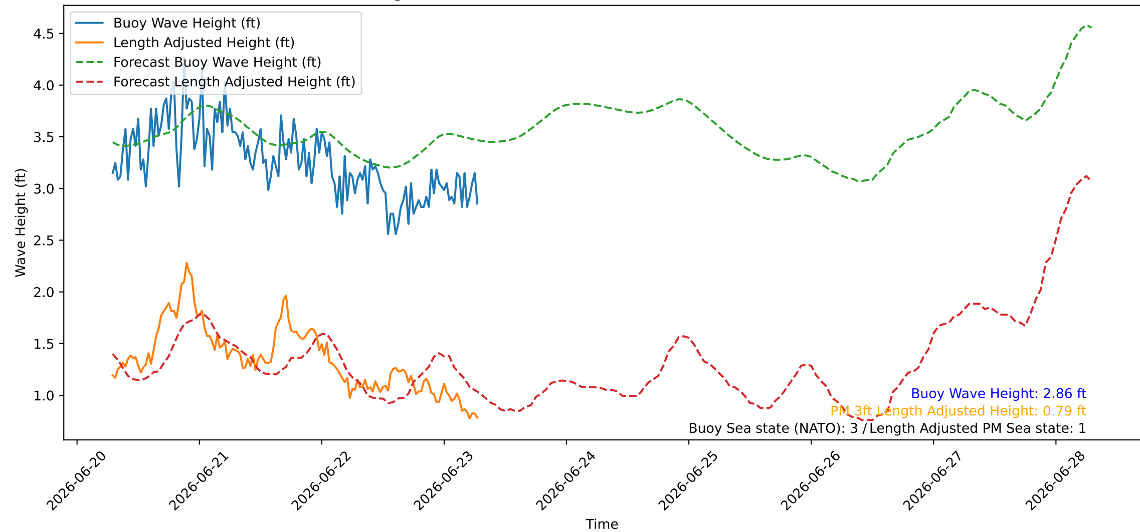
Wave Heights over Time for Oceanside Harbor at 2026-06-23 07:10:26
