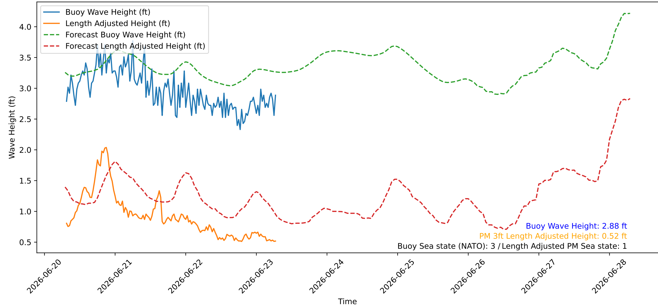
Wave Heights over Time for Red Beach at 2026-06-23 07:10:45
