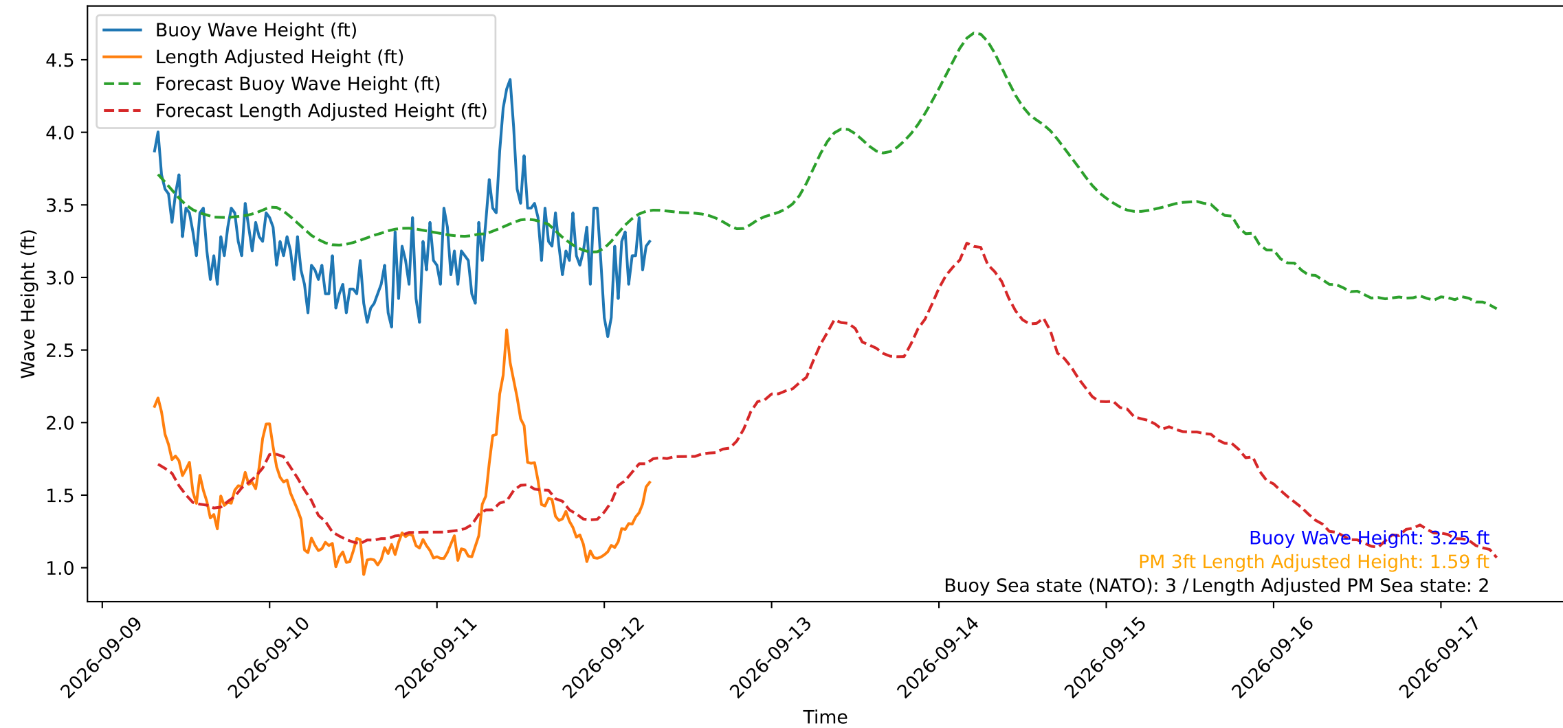
Wave Heights over Time for Oceanside Harbor at 2026-09-12 07:30:29
