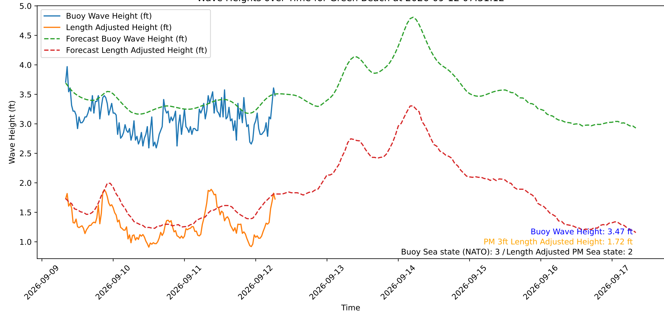
Wave Heights over Time for Green Beach at 2026-09-12 07:31:12
