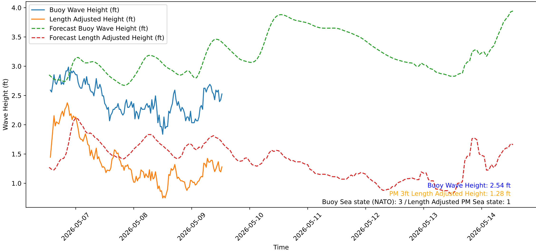
Wave Heights over Time for Green Beach at 2026-05-09 13:21:14
