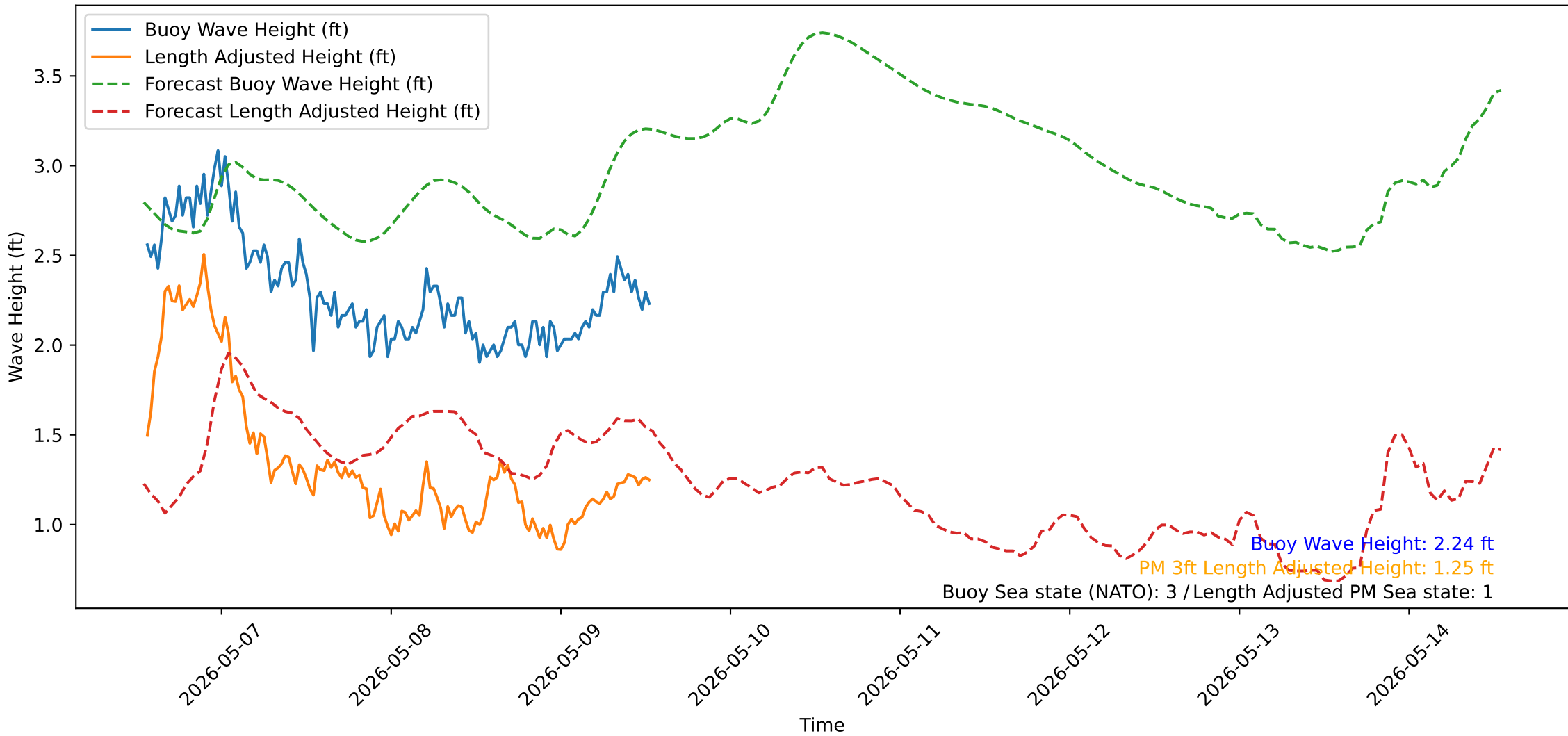
Wave Heights over Time for Red Beach at 2026-05-09 13:20:52
