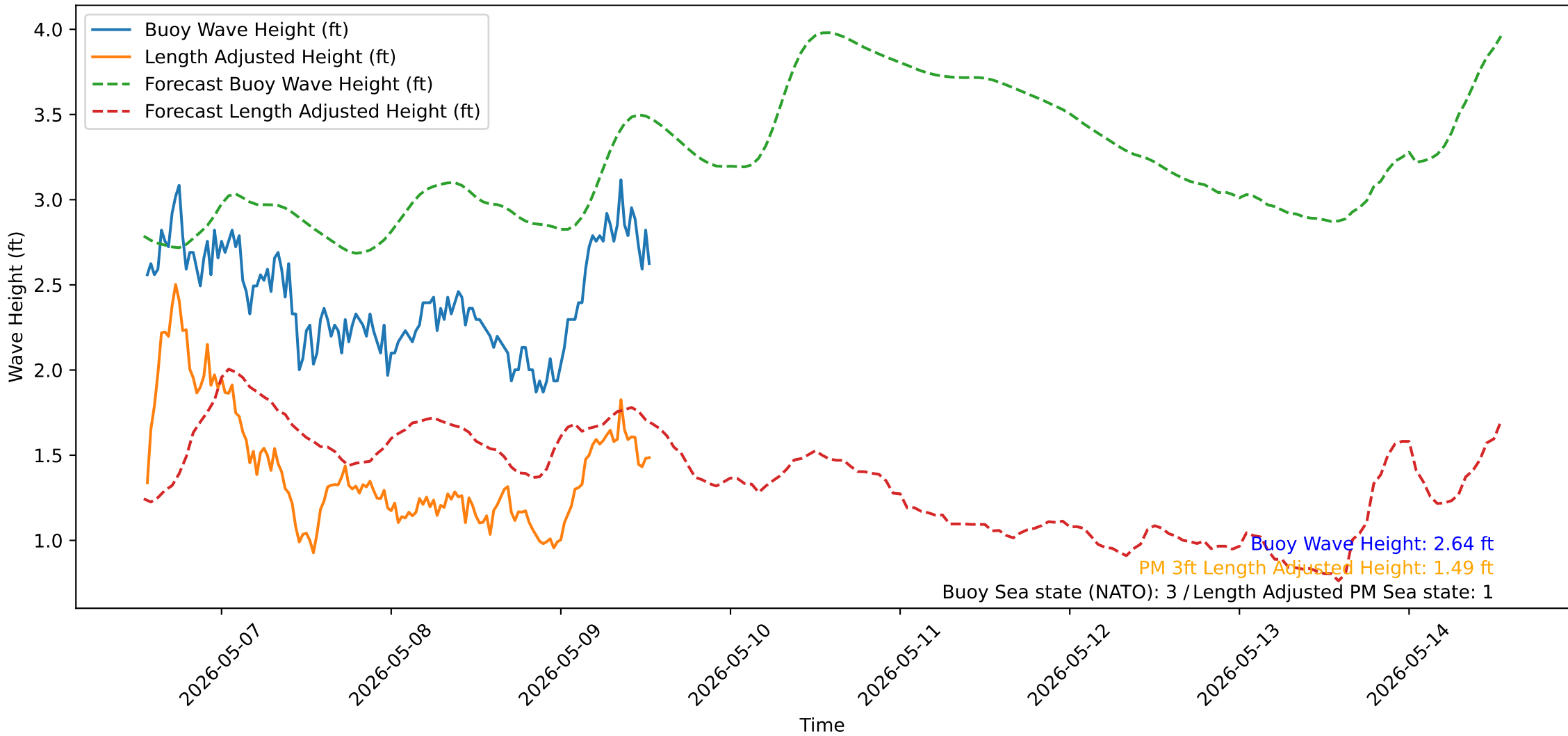
Wave Heights over Time for Oceanside Harbor at 2026-05-09 13:20:31
