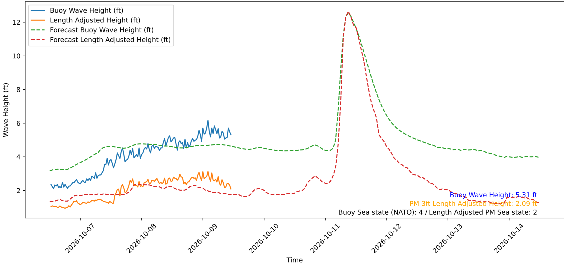
Wave Heights over Time for Green Beach at 2026-10-09 12:01:12
