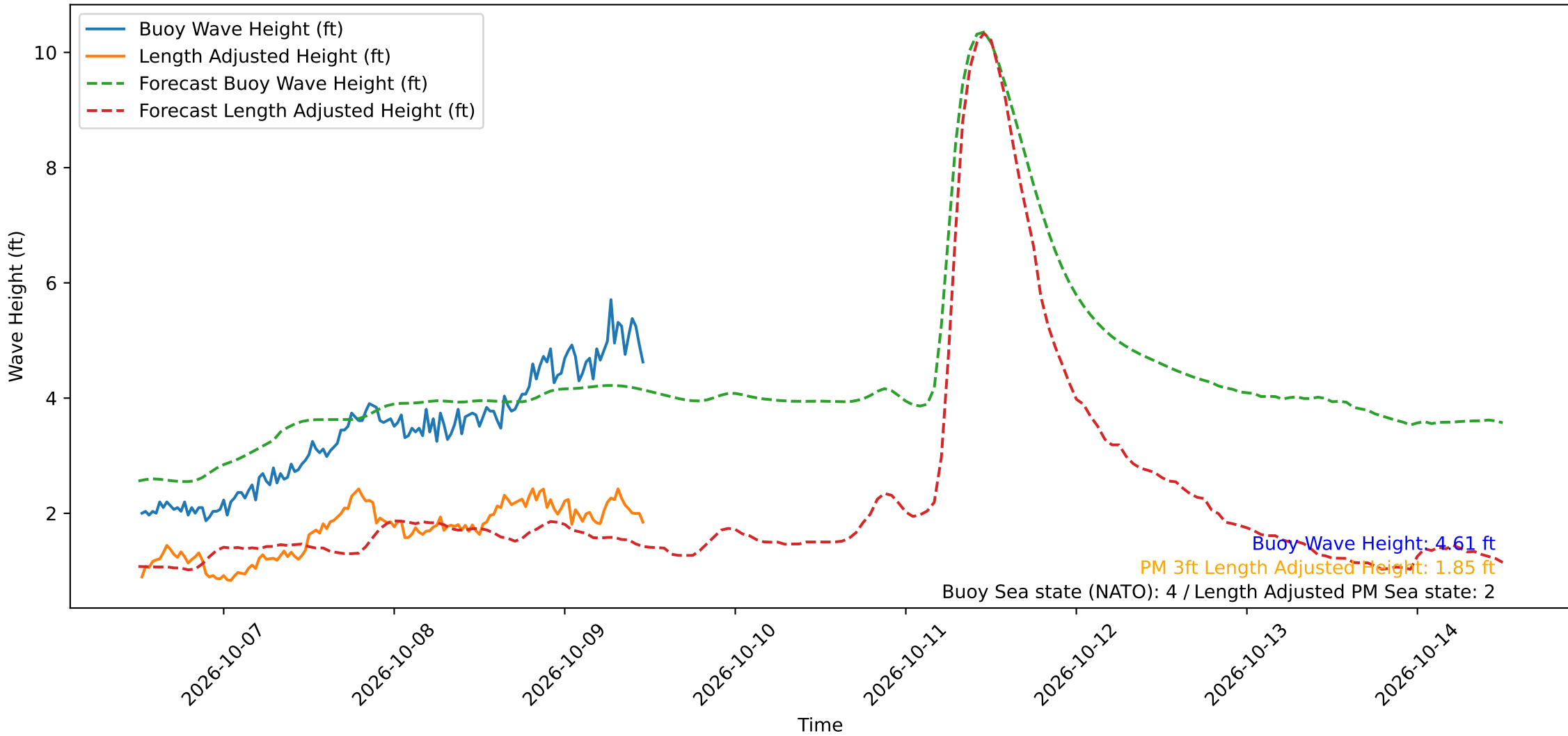
Wave Heights over Time for Red Beach at 2026-10-09 12:00:49
