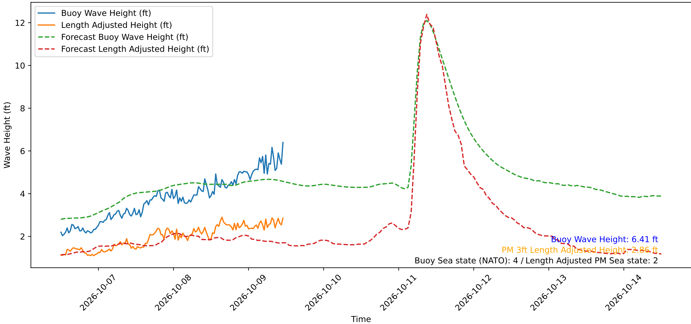
Wave Heights over Time for Oceanside Harbor at 2026-10-09 12:00:30
