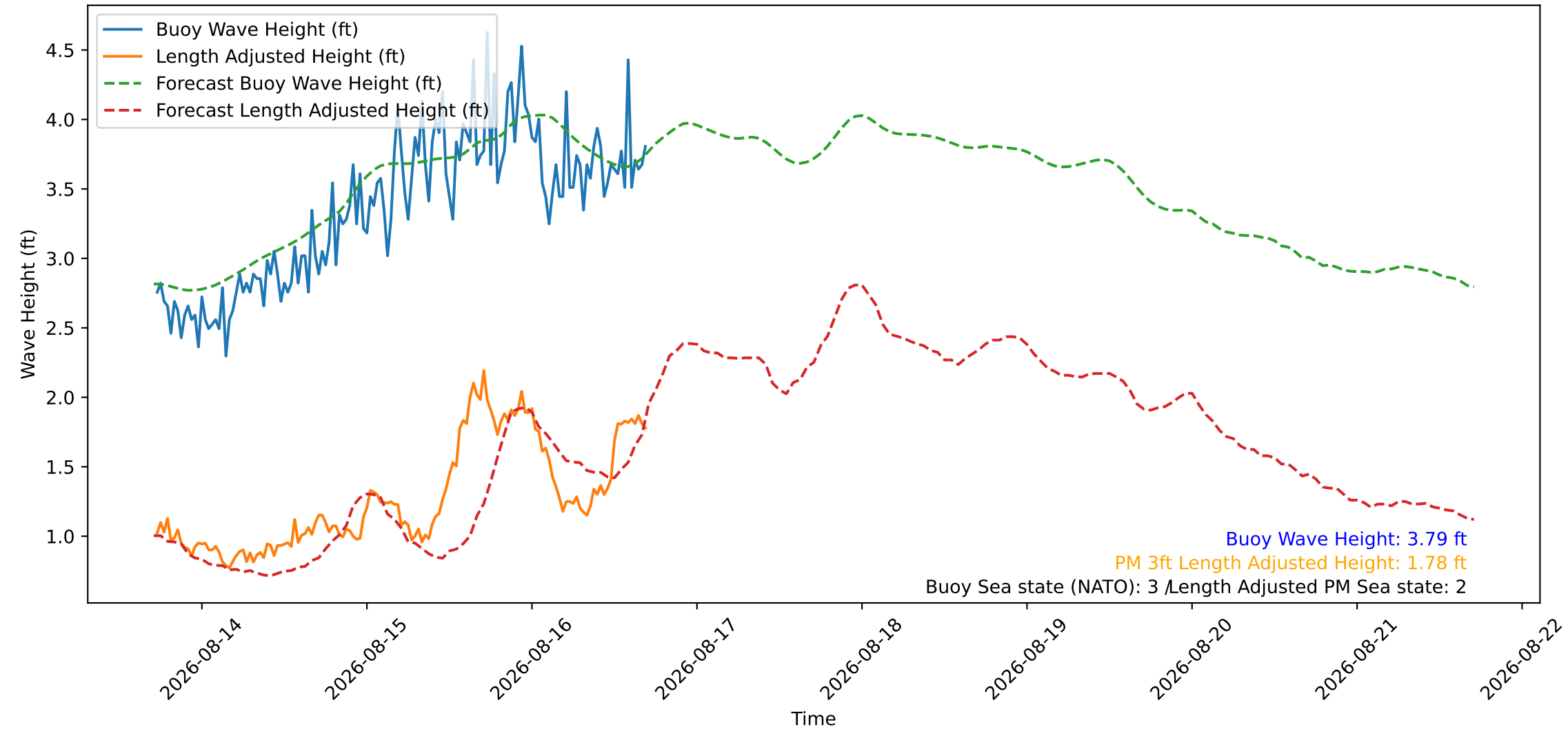
Wave Heights over Time for Oceanside Harbor at 2026-08-16 17:20:27
