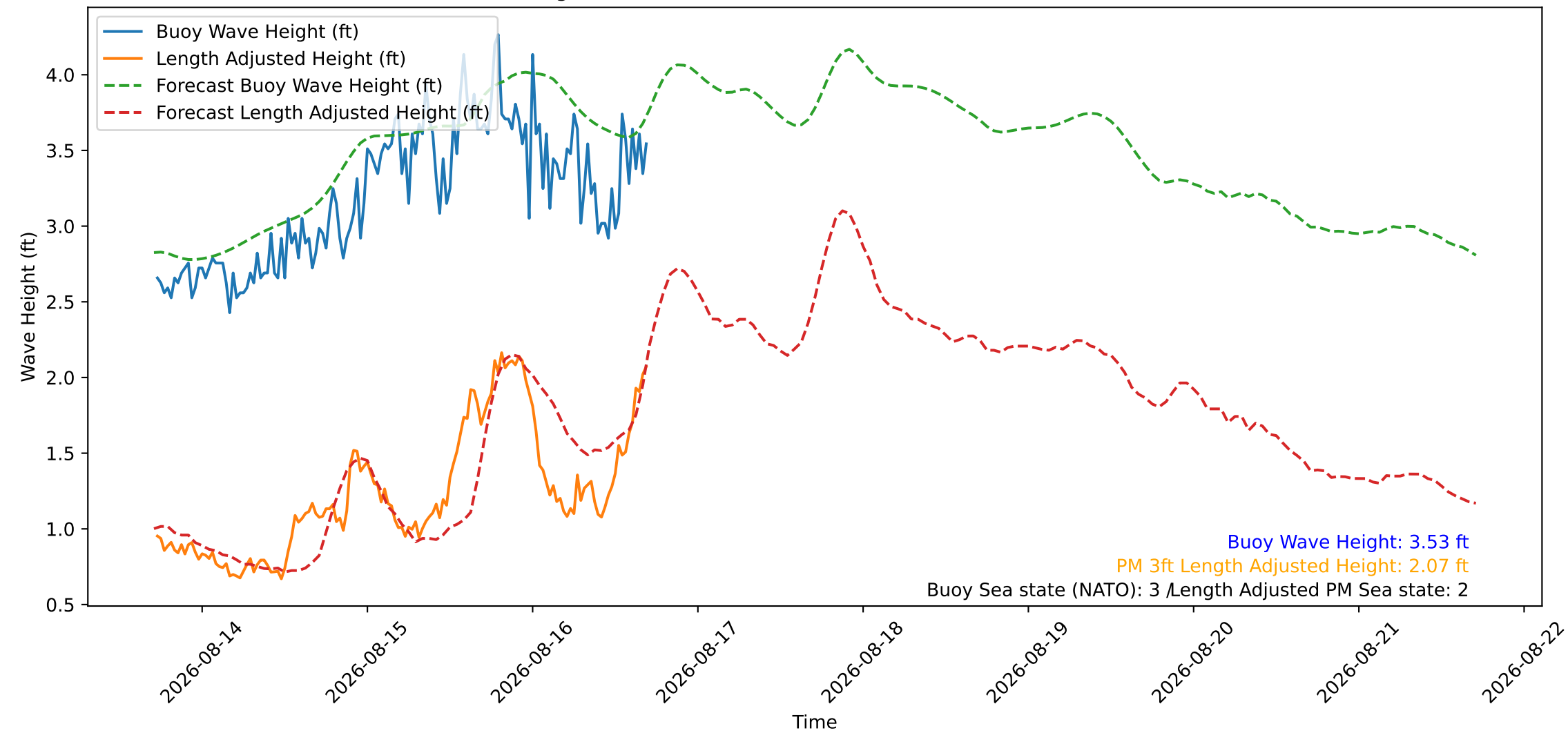
Wave Heights over Time for Green Beach at 2026-08-16 17:21:12
