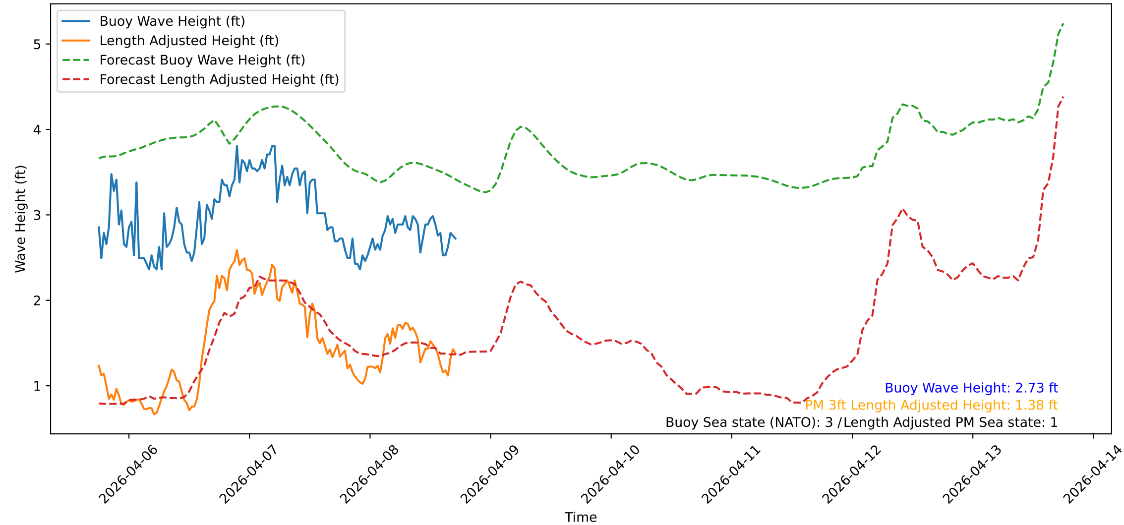
Wave Heights over Time for Green Beach at 2026-04-08 17:51:11
