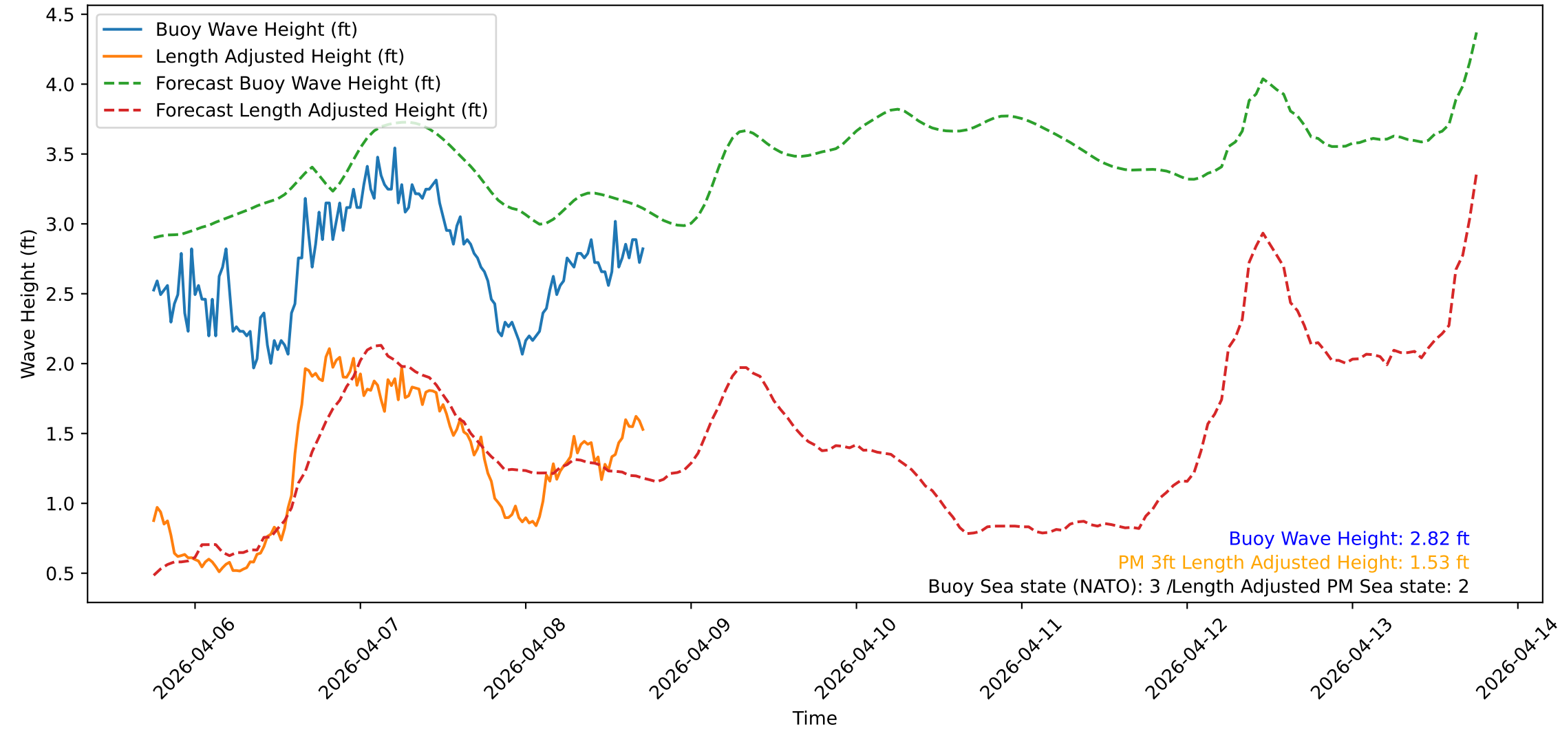
Wave Heights over Time for Red Beach at 2026-04-08 17:50:48
