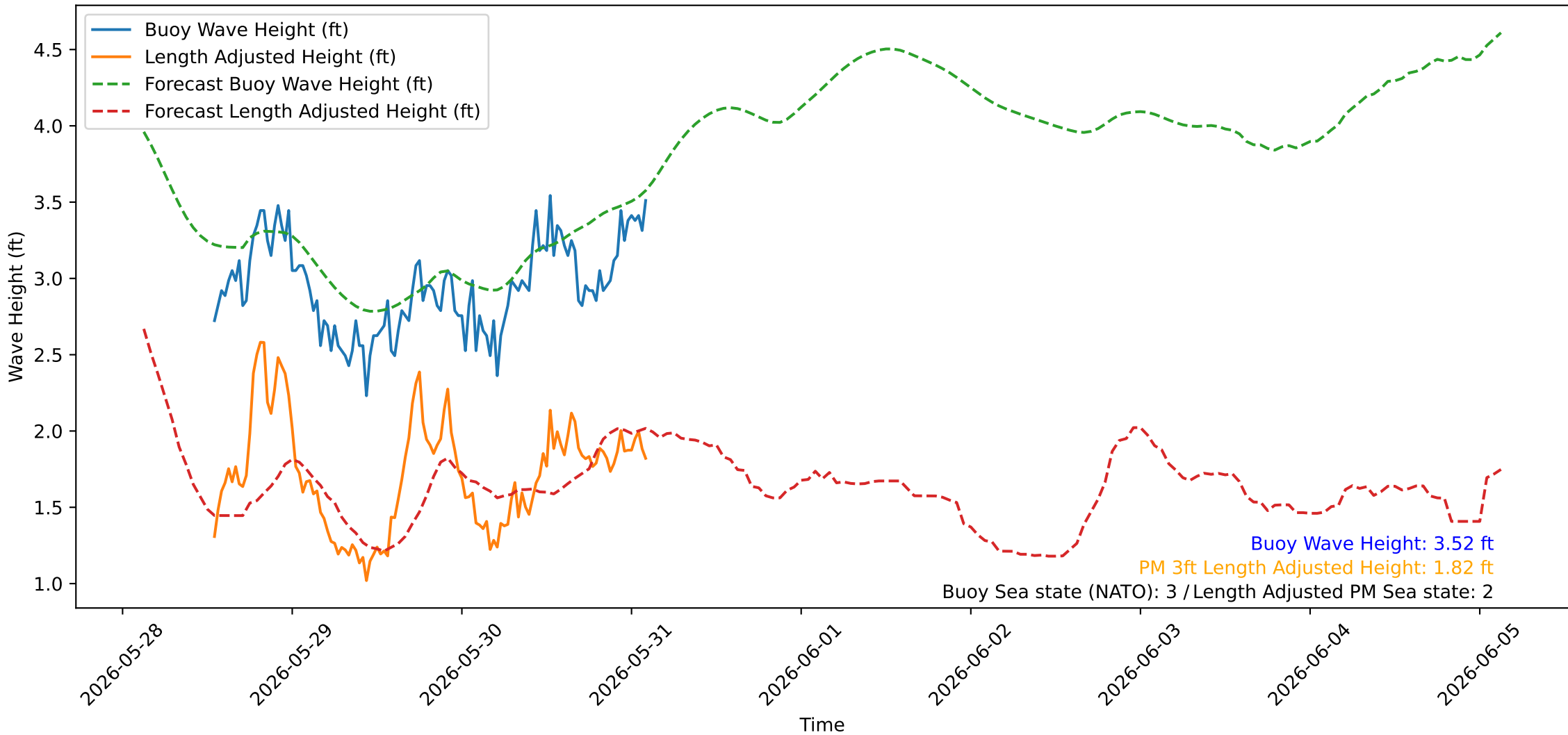
Wave Heights over Time for Oceanside Harbor at 2026-05-31 02:50:25
