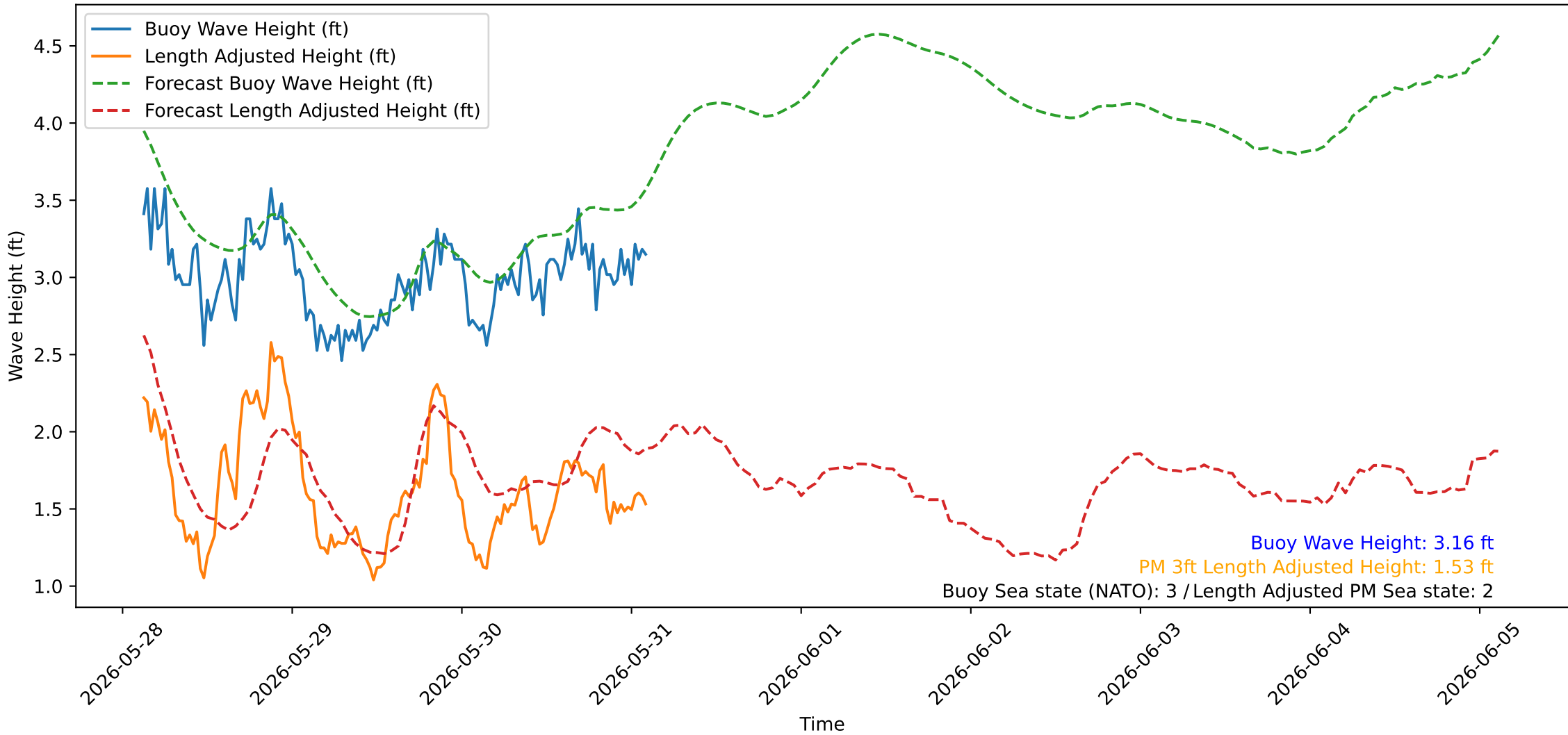
Wave Heights over Time for Green Beach at 2026-05-31 02:51:08
