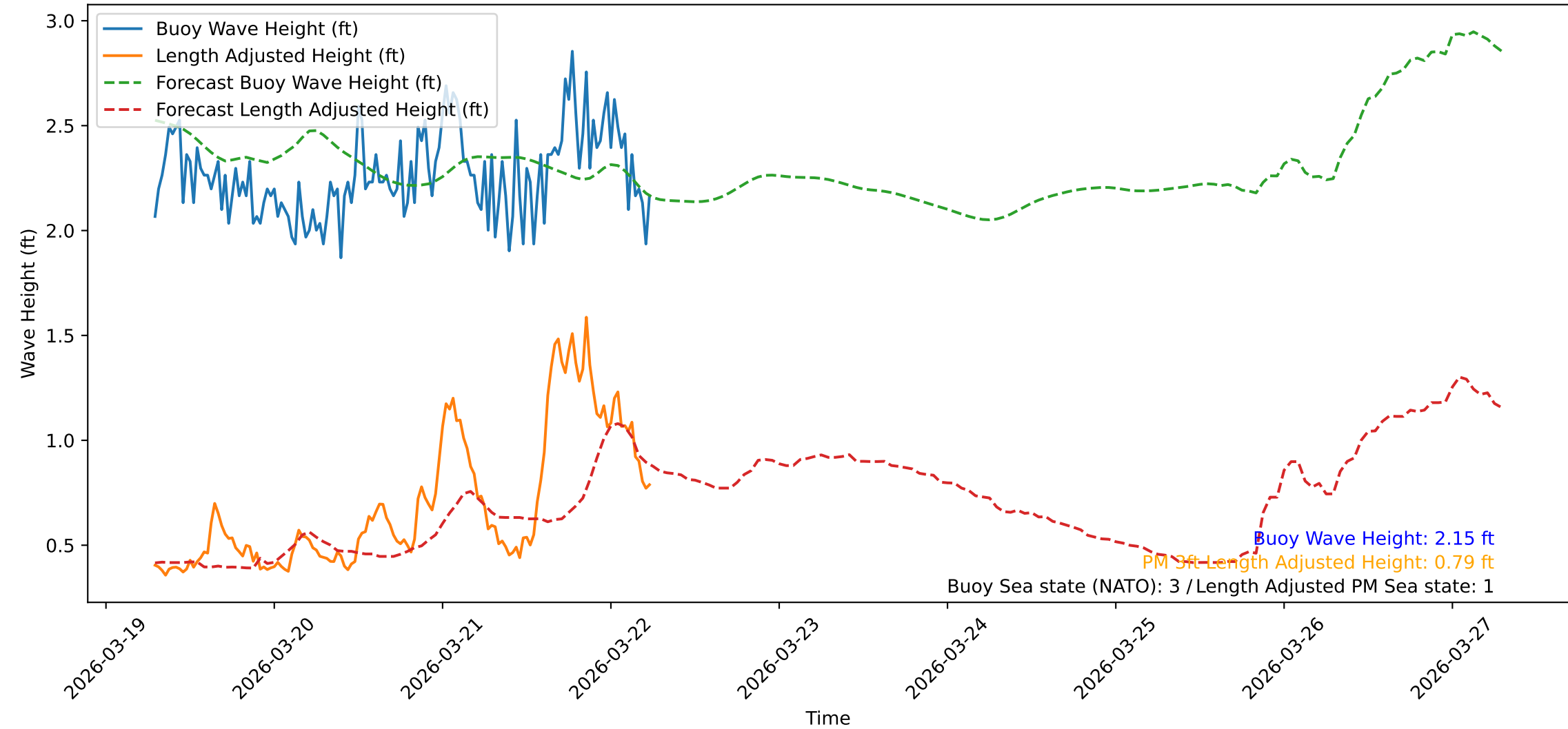
Wave Heights over Time for Red Beach at 2026-03-22 06:30:47
