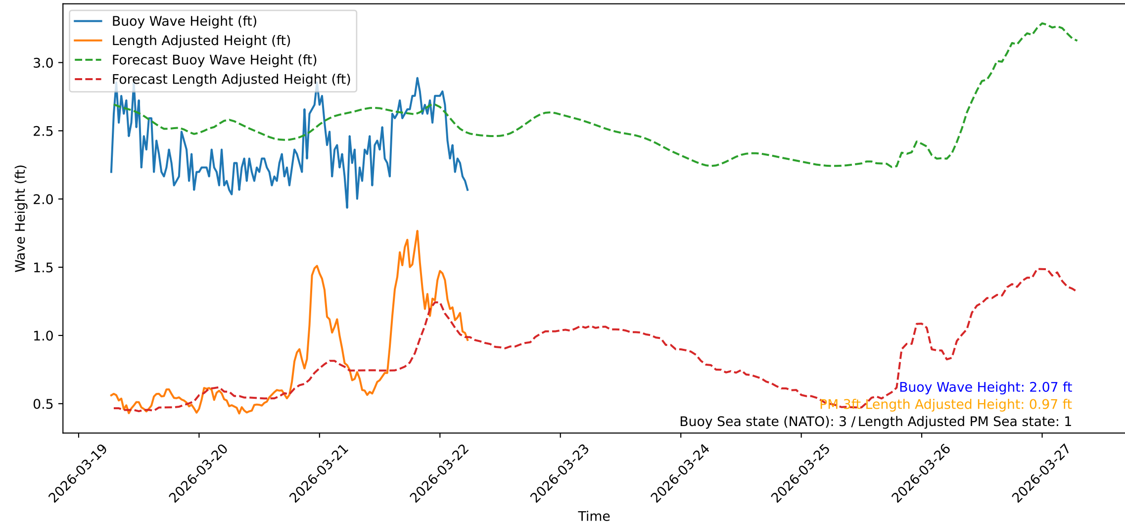
Wave Heights over Time for Green Beach at 2026-03-22 06:31:09
