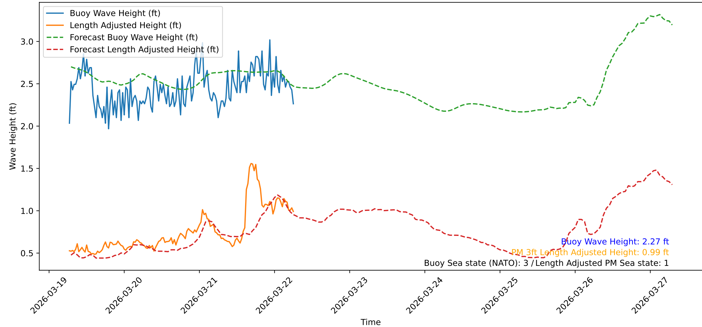
Wave Heights over Time for Oceanside Harbor at 2026-03-22 06:30:31
