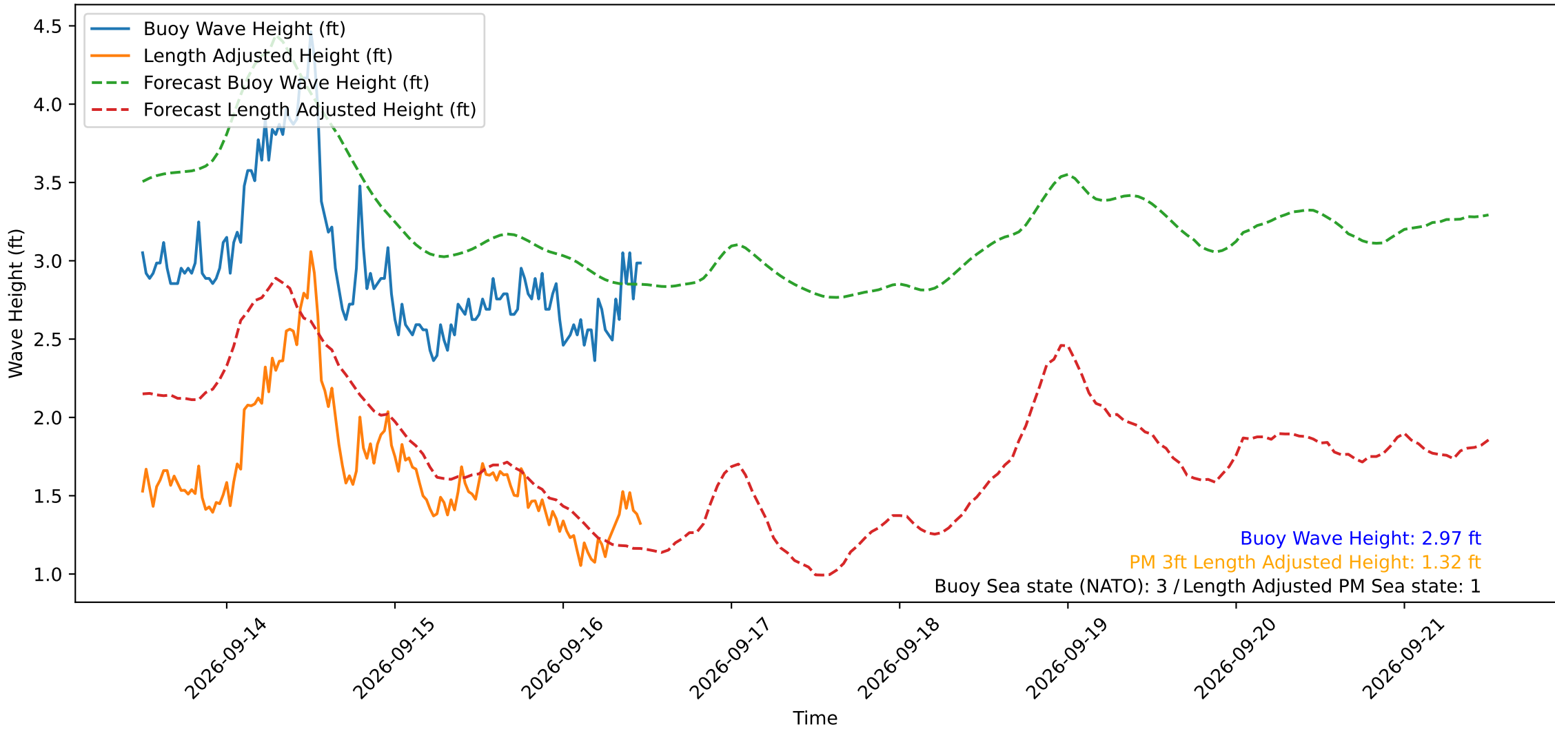
Wave Heights over Time for Oceanside Harbor at 2026-09-16 11:50:30
