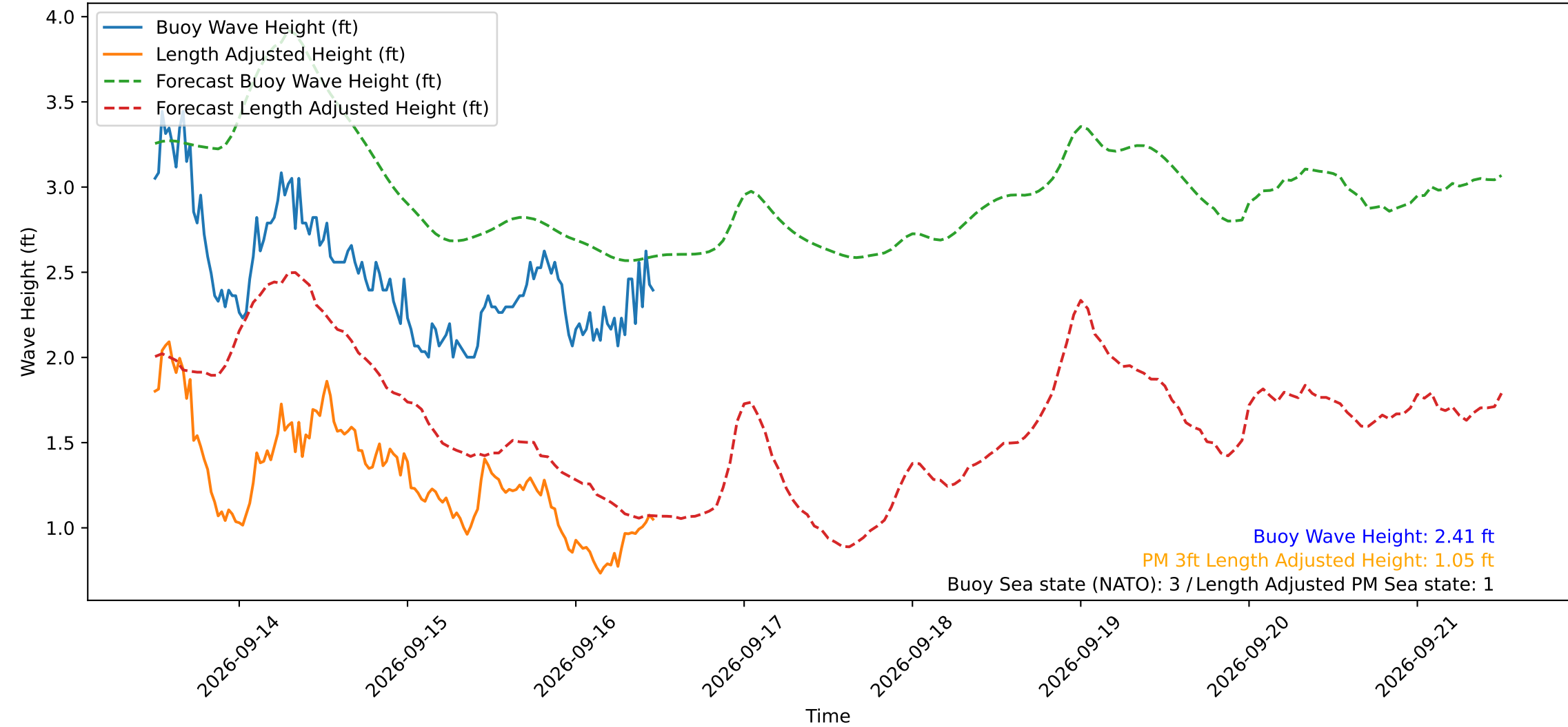
Wave Heights over Time for Red Beach at 2026-09-16 11:50:51
