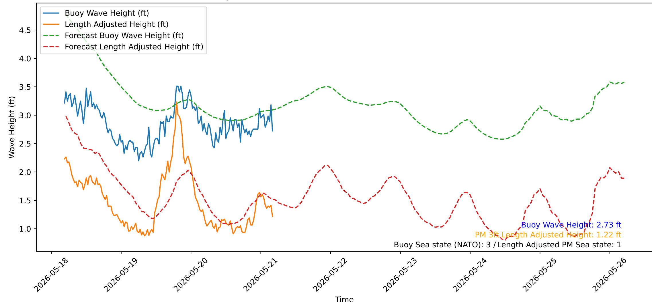
Wave Heights over Time for Oceanside Harbor at 2026-05-21 04:40:31
