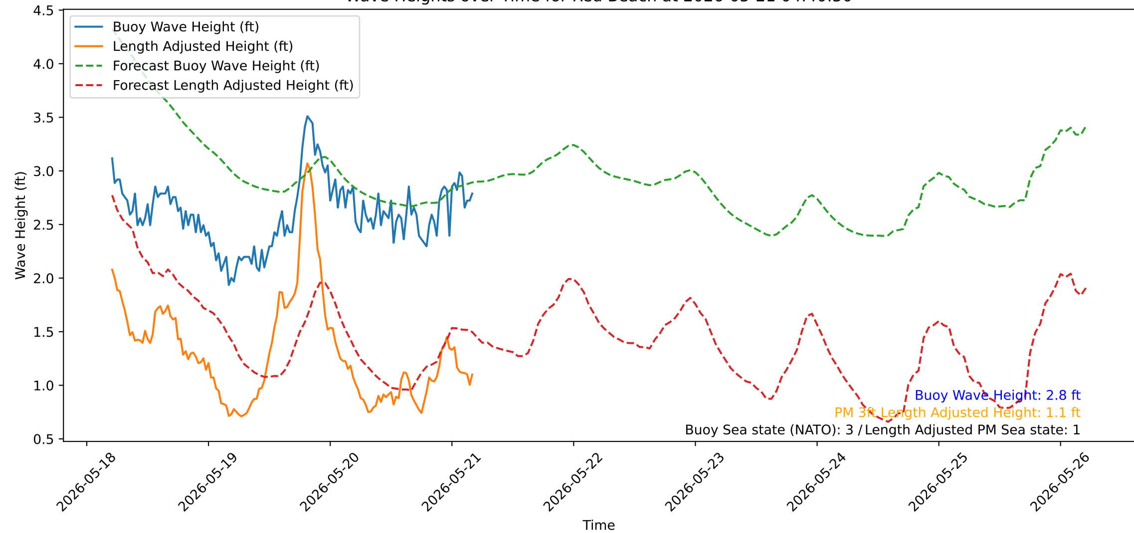
Wave Heights over Time for Red Beach at 2026-05-21 04:40:50
