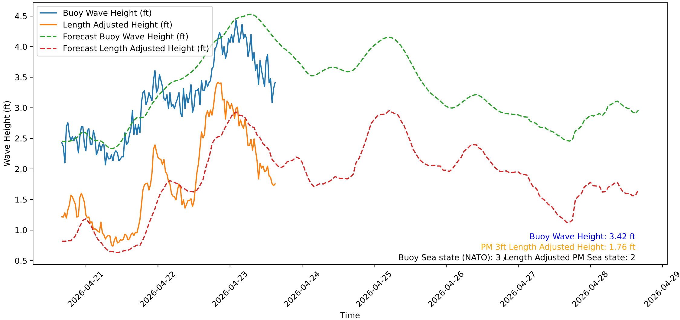
Wave Heights over Time for Oceanside Harbor at 2026-04-23 15:50:31
