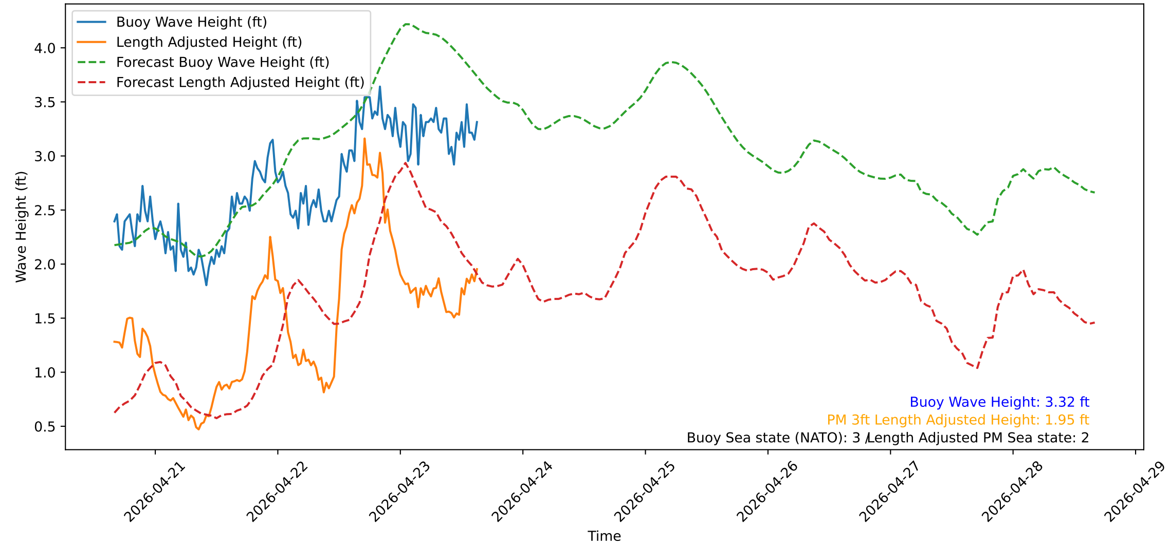
Wave Heights over Time for Red Beach at 2026-04-23 15:50:51
