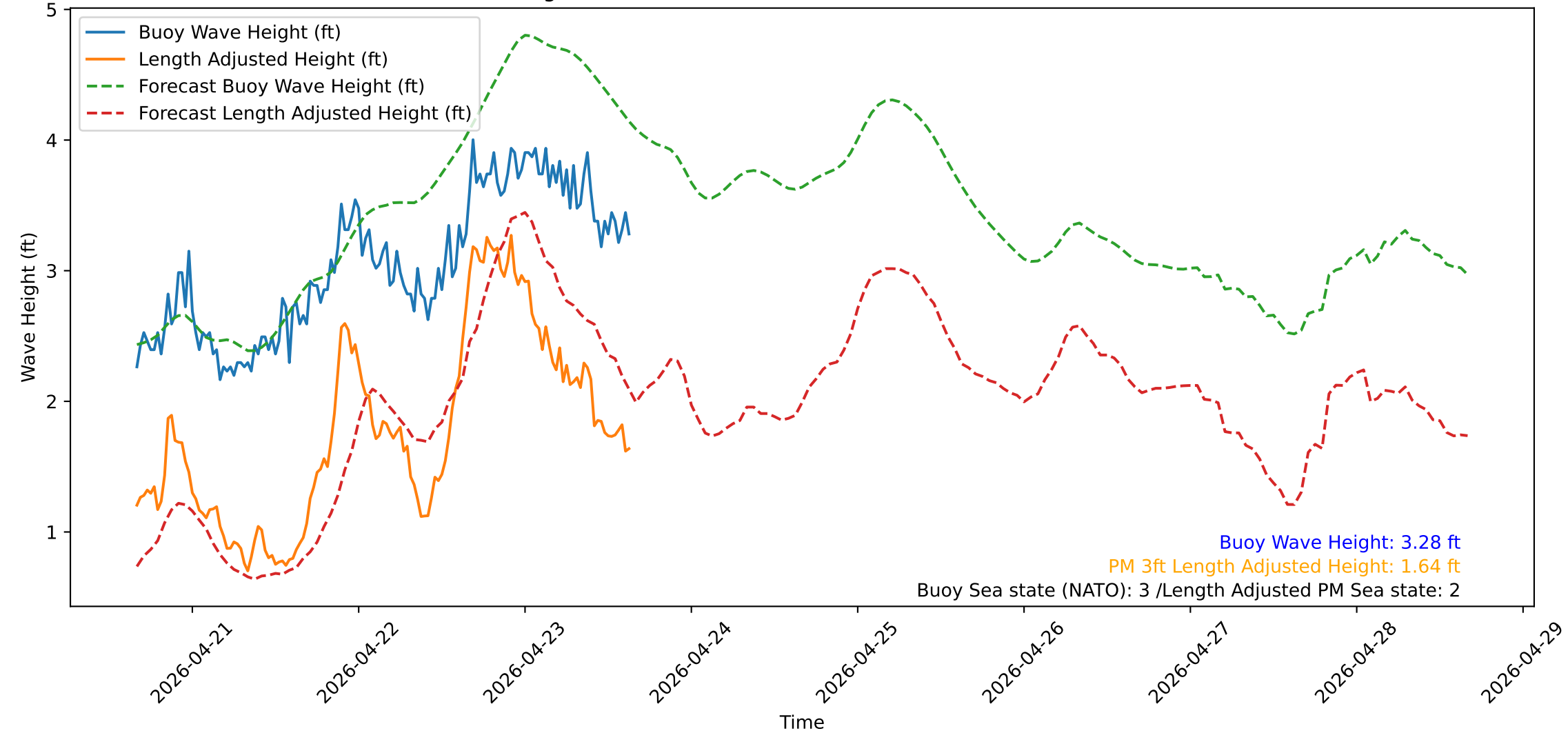
Wave Heights over Time for Green Beach at 2026-04-23 15:51:14
