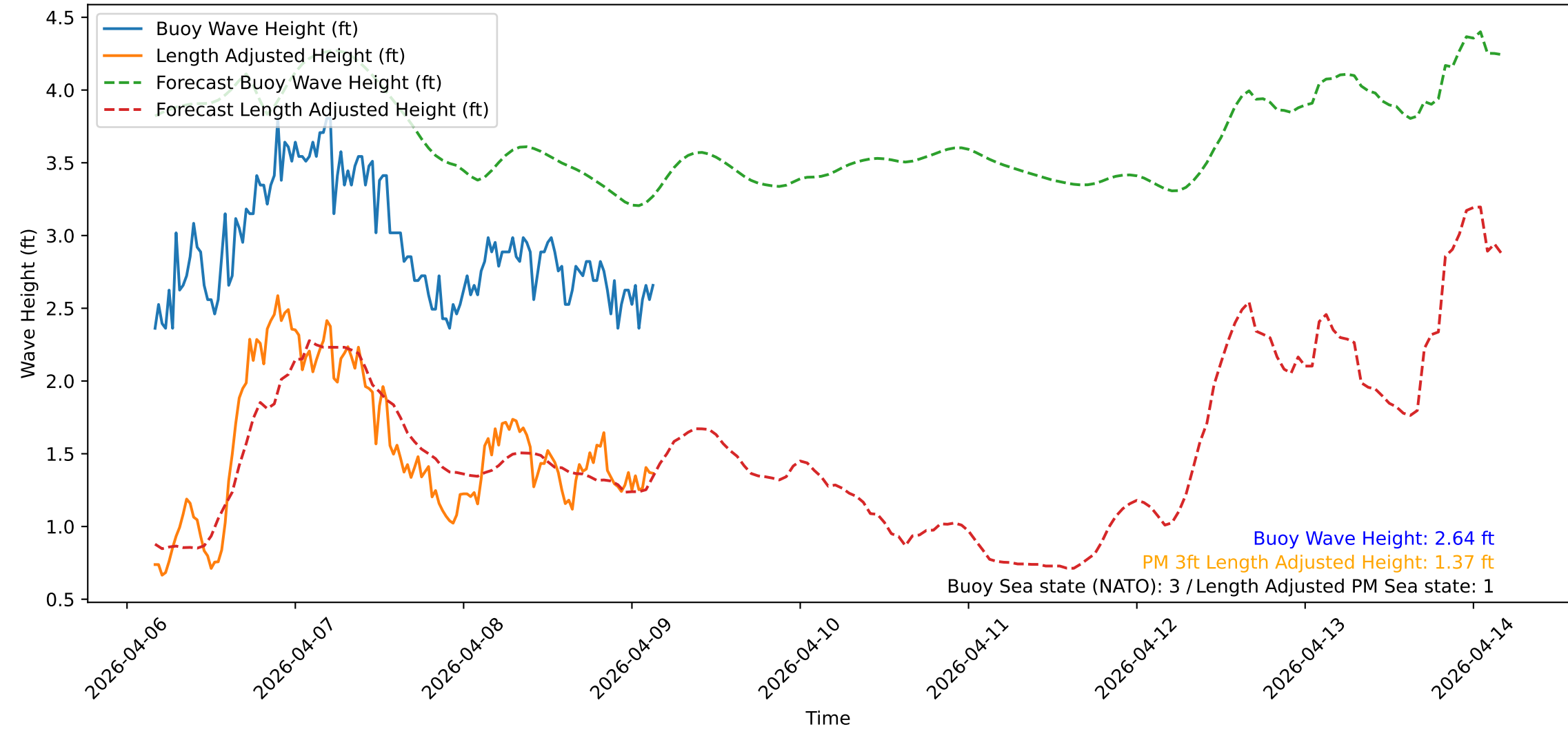
Wave Heights over Time for Green Beach at 2026-04-09 04:01:08
