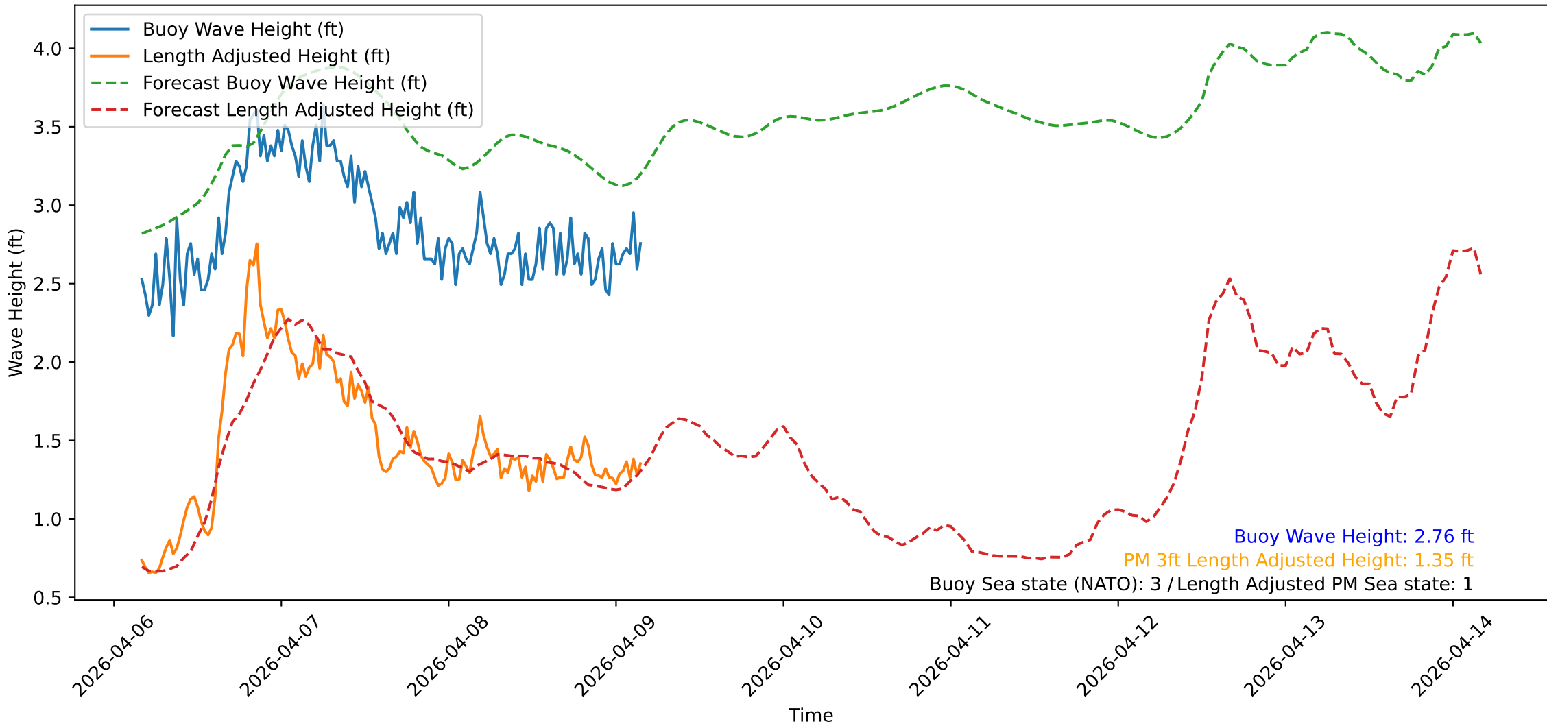
Wave Heights over Time for Oceanside Harbor at 2026-04-09 04:00:31
