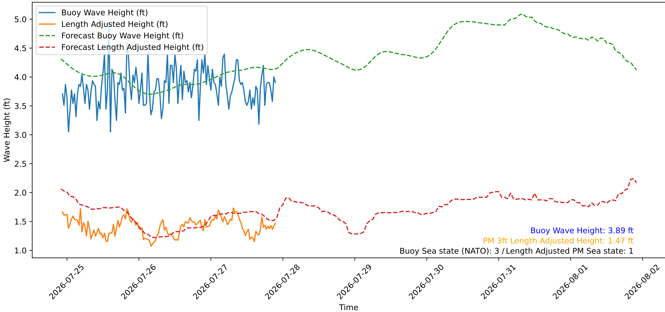
Wave Heights over Time for Oceanside Harbor at 2026-07-27 22:20:26
