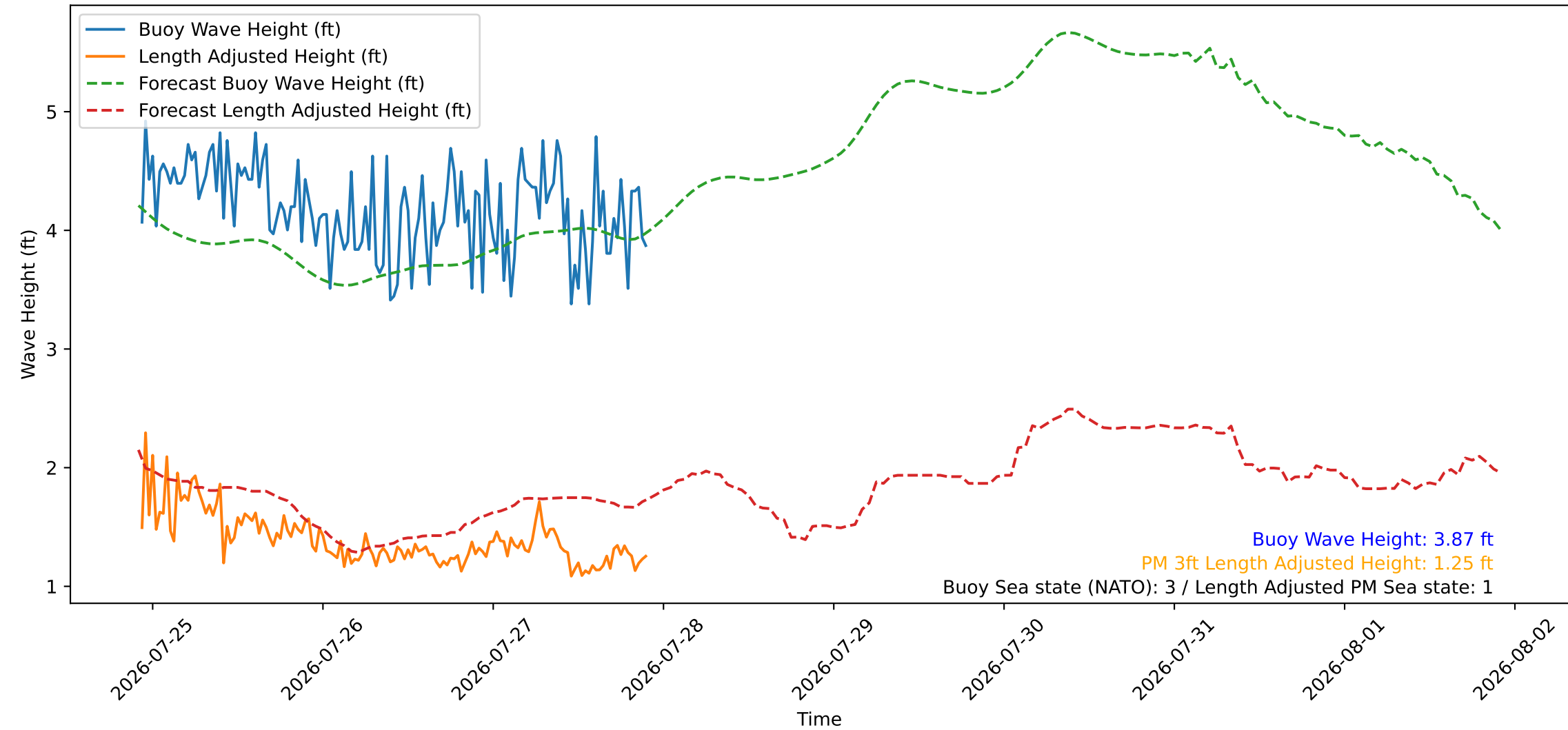
Wave Heights over Time for Green Beach at 2026-07-27 22:21:10
