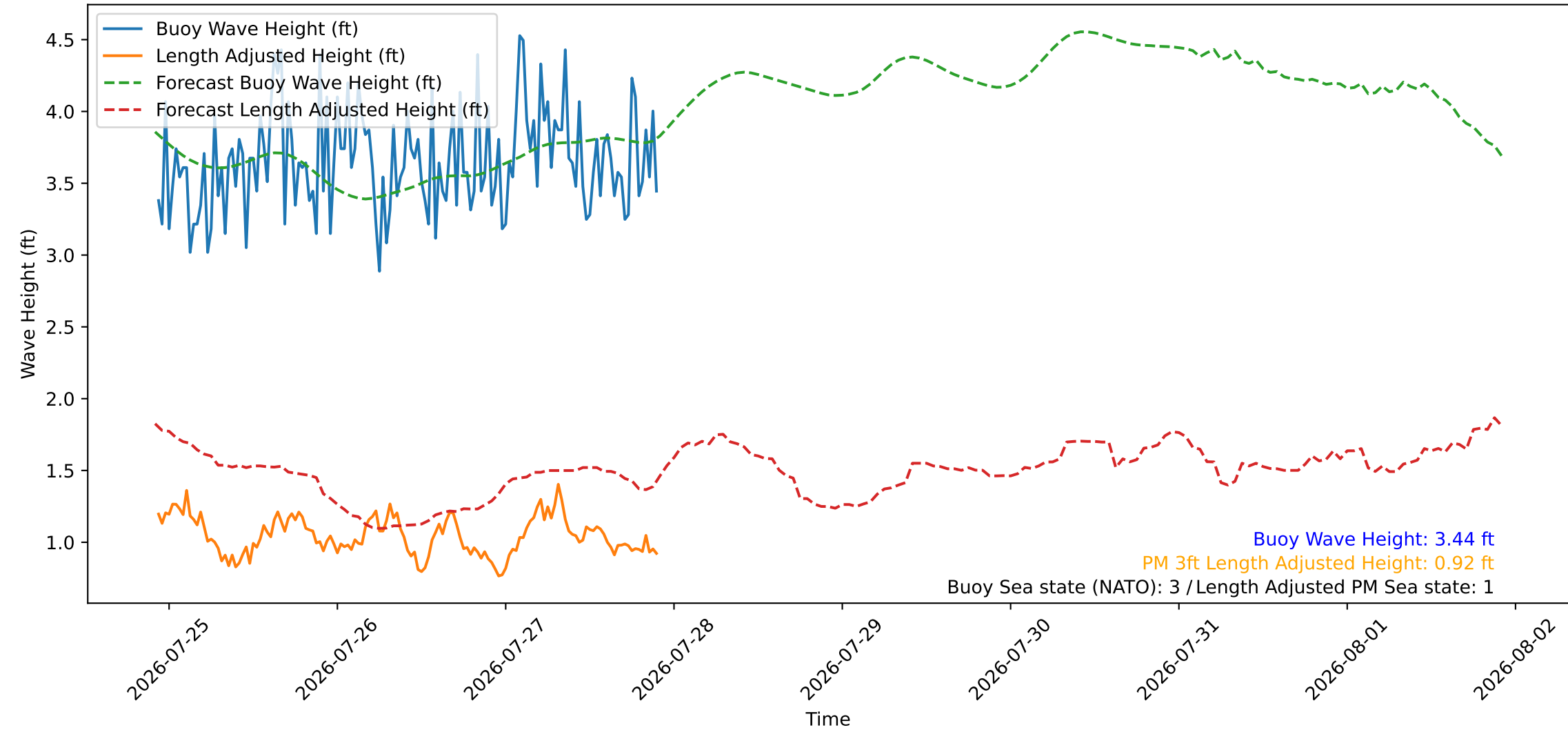
Wave Heights over Time for Red Beach at 2026-07-27 22:20:47
