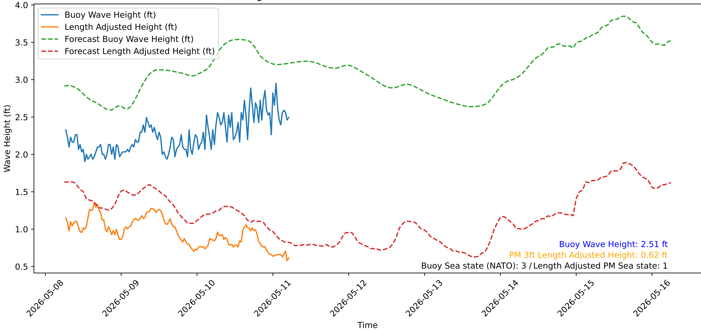
Wave Heights over Time for Red Beach at 2026-05-11 06:00:50
