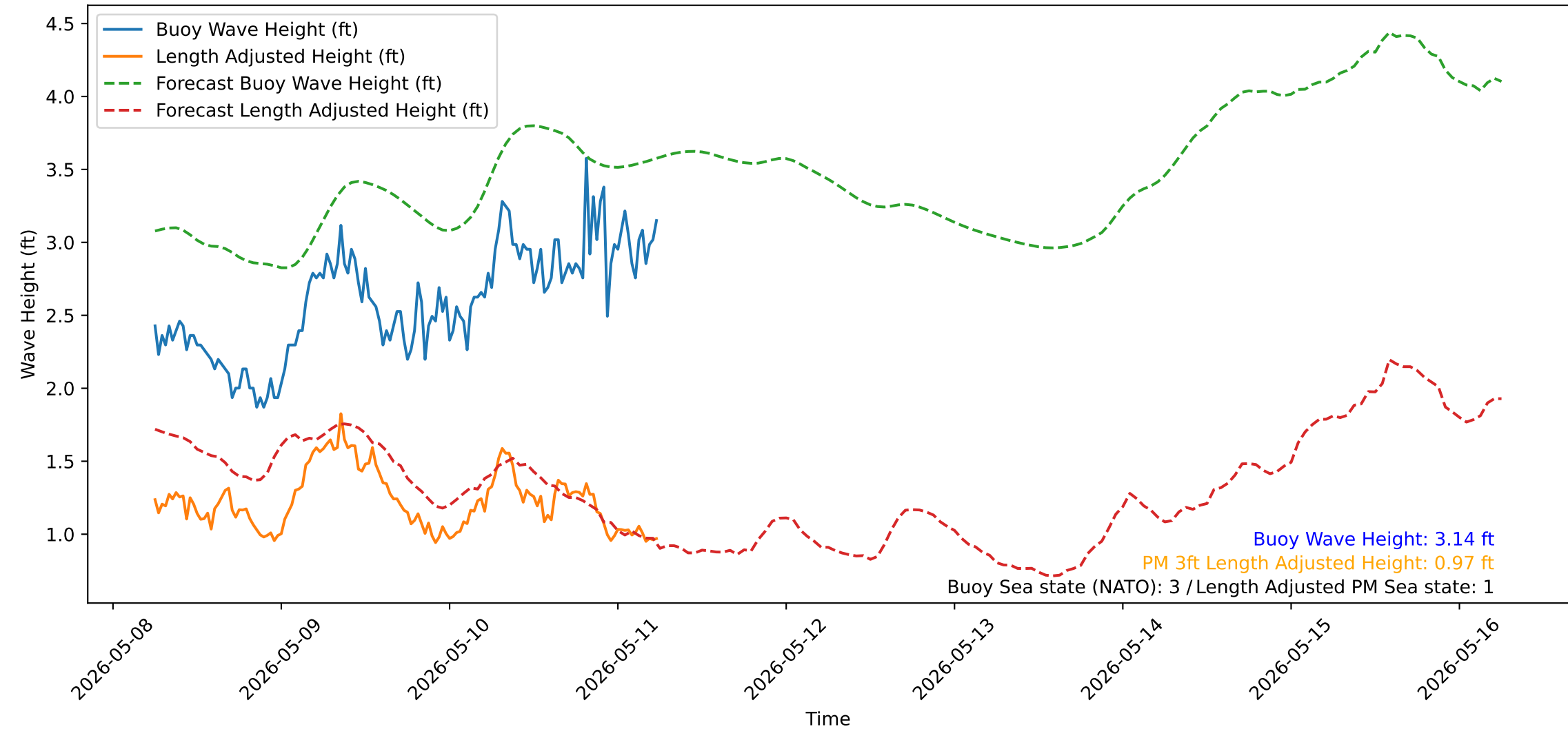
Wave Heights over Time for Oceanside Harbor at 2026-05-11 06:00:31
