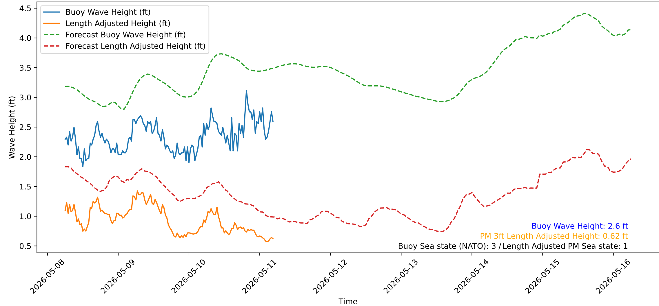
Wave Heights over Time for Green Beach at 2026-05-11 06:01:12
