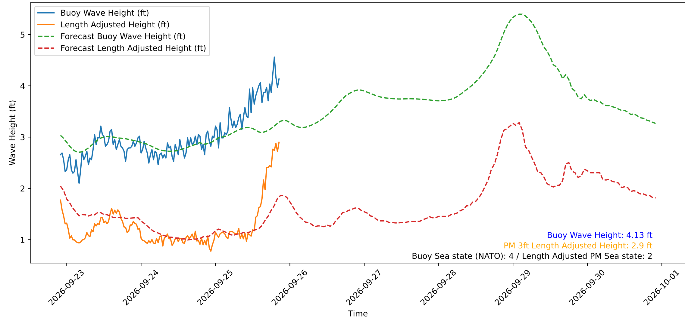
Wave Heights over Time for Green Beach at 2026-09-25 21:31:12
