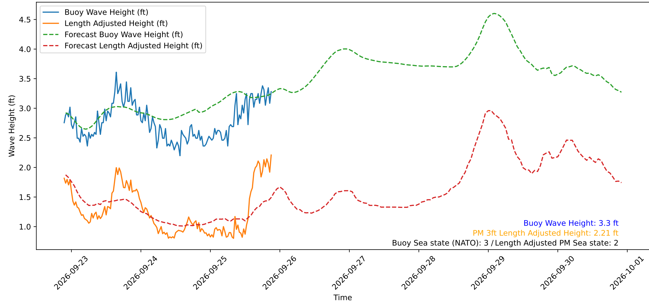
Wave Heights over Time for Oceanside Harbor at 2026-09-25 21:30:29
