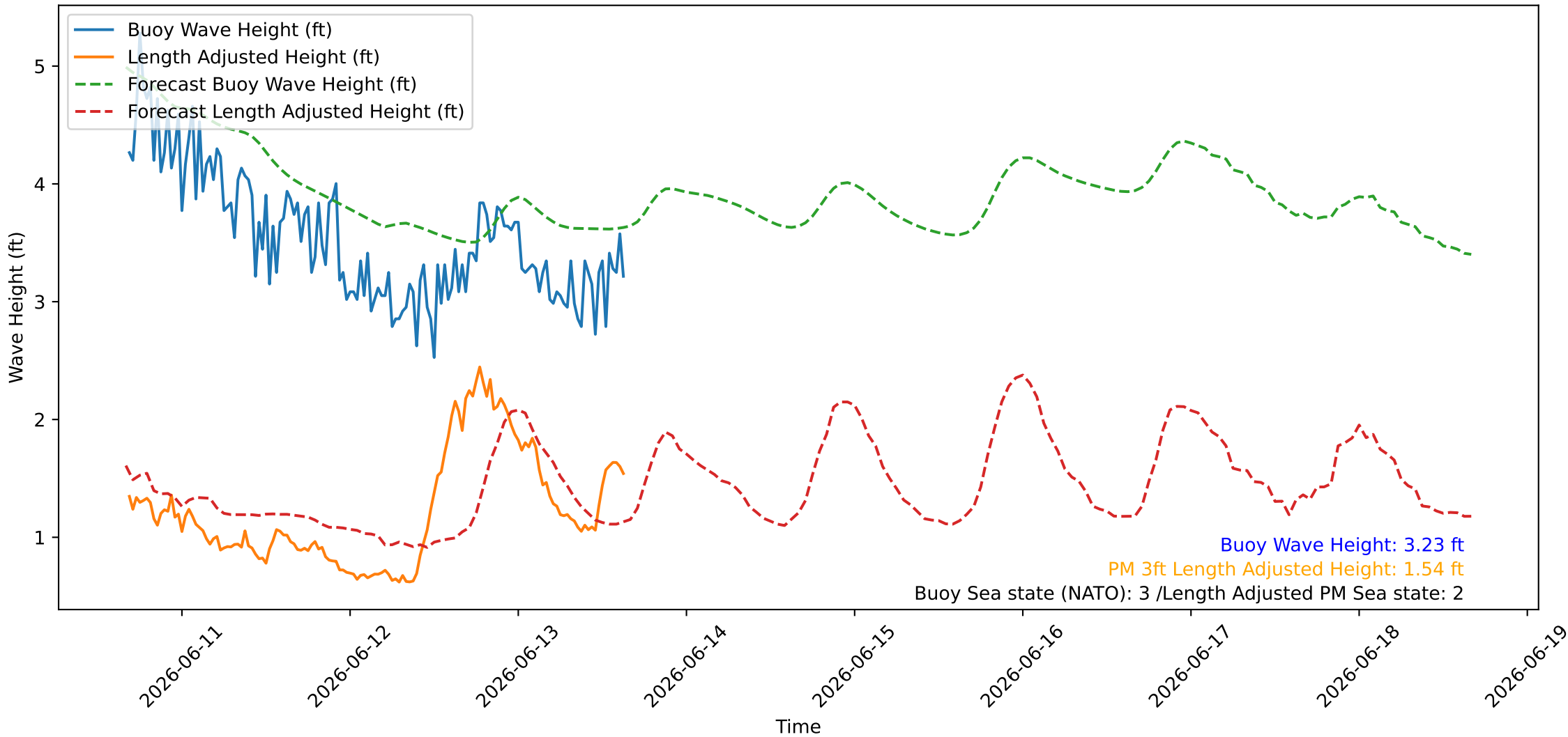
Wave Heights over Time for Red Beach at 2026-06-13 16:00:45
